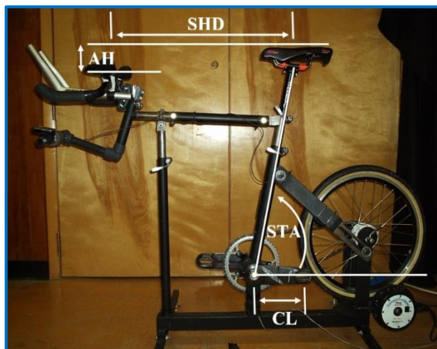
Figure 1. Illustration of several geometry variables transferred to the testing ergometer from each cyclist's time-trial bicycle: Seat-tube angle (STA), seat-to-handlebar distance (SHD), aero handlebar height (AH), and crank length (CL).
