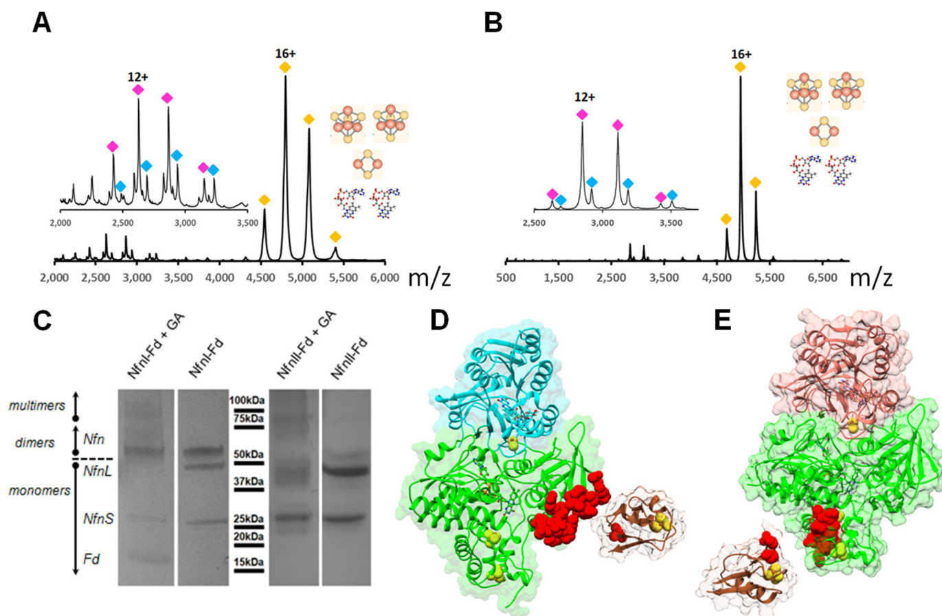
Figure 4. Native and chemical cross-linking mass spectrometry of NfnI and NfnII. Native mass spectrum of NfnI complex (A) and NfnII complex (B) in the gas phase. Yellow diamonds, charge states of the intact complex centered around charge 16+. After deconvolution, the intact NfnI complex is 86,407 Da (expected: 86,425 Da) and NfnII is 88,951 Da (expected 88,901 Da), consistent with complexes containing one small and large subunit, two FAD molecules, two [4Fe–4S] clusters, and one [2Fe–2S] cluster. Under conditions of low collision energy (80 V for NfnI and 60 V for NfnII), the subunits dissociated ( insets in A and B ). Blue and magenta diamonds, charge envelopes of small subunits with and without one FAD cofactor. C, SDS-PAGE of glutaraldehyde (GA)-cross-linked NfnI-Fd and NfnII-Fd complexes. LC-MS analysis revealed that ferredoxin (brown) interacts with the large subunits (green) of NfnI (D) and NfnII (E). Red space-filling regions show cross-linked peptides of NfnI and NfnII. Small subunits are colored in cyan and red, respectively. In all experiments, Nfn enzymes were used “as purified.” The NfnI structure is PDB entry 5JFC; NfnII structure is PDB entry 5VJ7.
