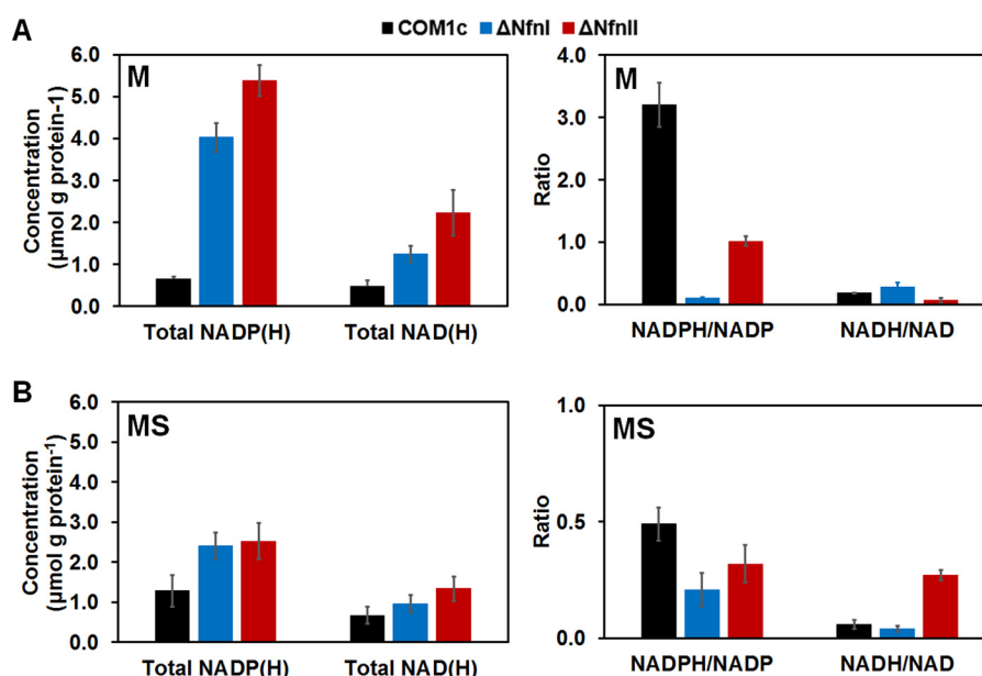
Figure 3. Redox nucleotide pool analysis: total concentration of NADP(H), NAD(H), NADPH/NADP + and NADH/NAD + ratios of COM1c (black; control), ΔNfnI (blue), and ΔNfnII (red) strains in M (A) and MS media (B) at 90 °C. The S.D. (error bars) analyses were taken from three independent biological samples.
