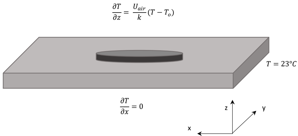
FIGURE 3. THE BASIC SHAPE OF THE MATHEMATICAL MODEL DOMAIN REPRESENTING THE FLATTENED INTESTINE (LIGHT GREY) WITH DIMENSIONS OF [50MM X 20MM X 4 MM] AND A CIRCULAR PATCH (DARK GREY) OF 10 MM DIAMETER PROTRUDING ATOP THE CENTER OF THE BRICK WAS USED IN THE MODEL WITH ITS CORRESPONDING BOUNDARY.
