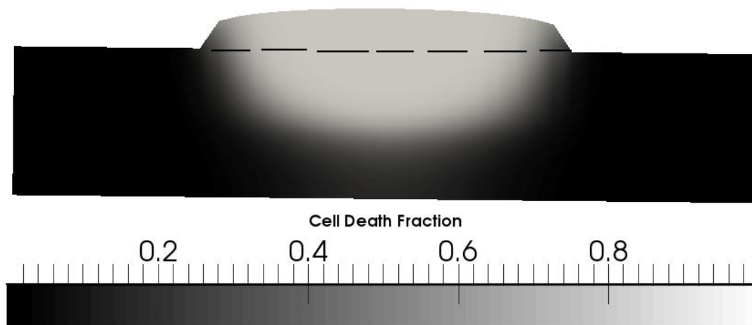
FIGURE 7. CELL DEATH FRACTION THROUGH THE PORCINE TISSUE AFTER 4 MINUTES OF LASER TREATMENT AT 2.33 W/CM 2 CW. THE DASHED LINE (–) REPRESENTS THE PATCH-TISSUE INTERFACE, WITH THE AREA ABOVE ENCOMPASSING THE CELL-FREE PATCH AND THE AREA BELOW ENCOMPASSING THE TISSUE.
