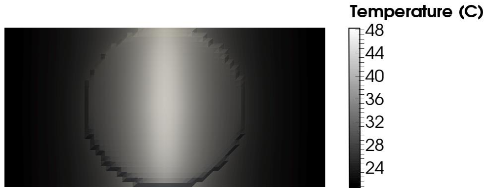
FIGURE 10. SURFACE TEMPERATURE PREDICTION FOR THE HEAT TRANSFER MODEL FOR MOUSE TISSUE AFTER 4 MINUTES OF LASER DURATION.
