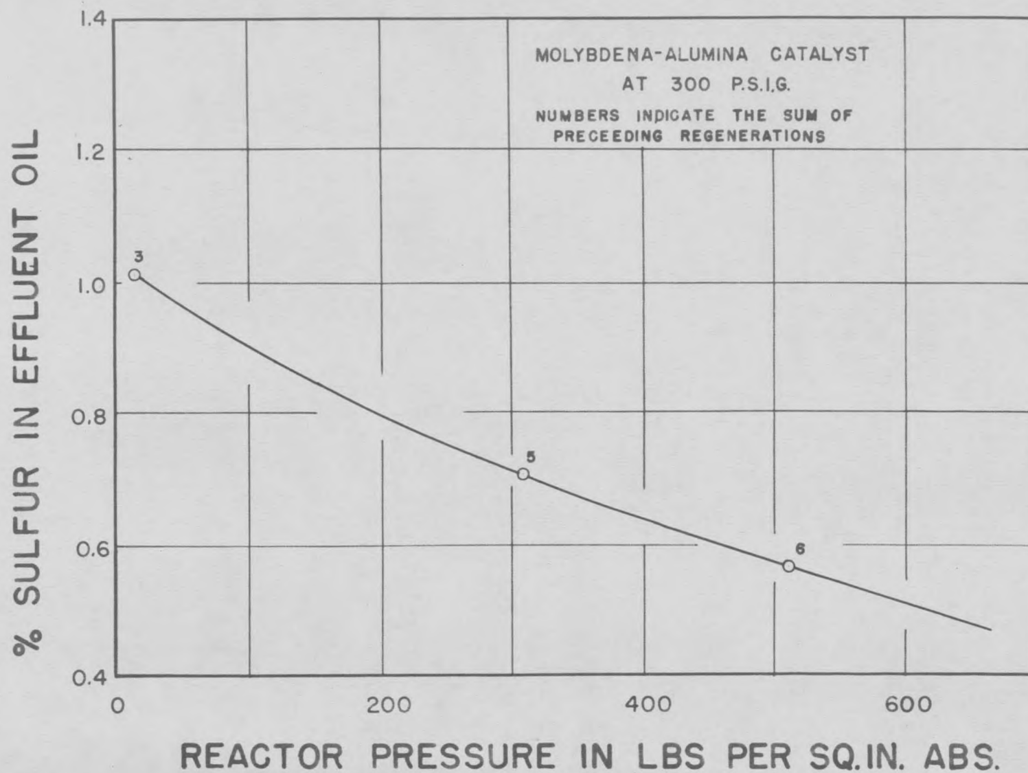
Fig. 12 Plot of Reactor Pressure vs. Desulfurization with Molybdena-alumina
