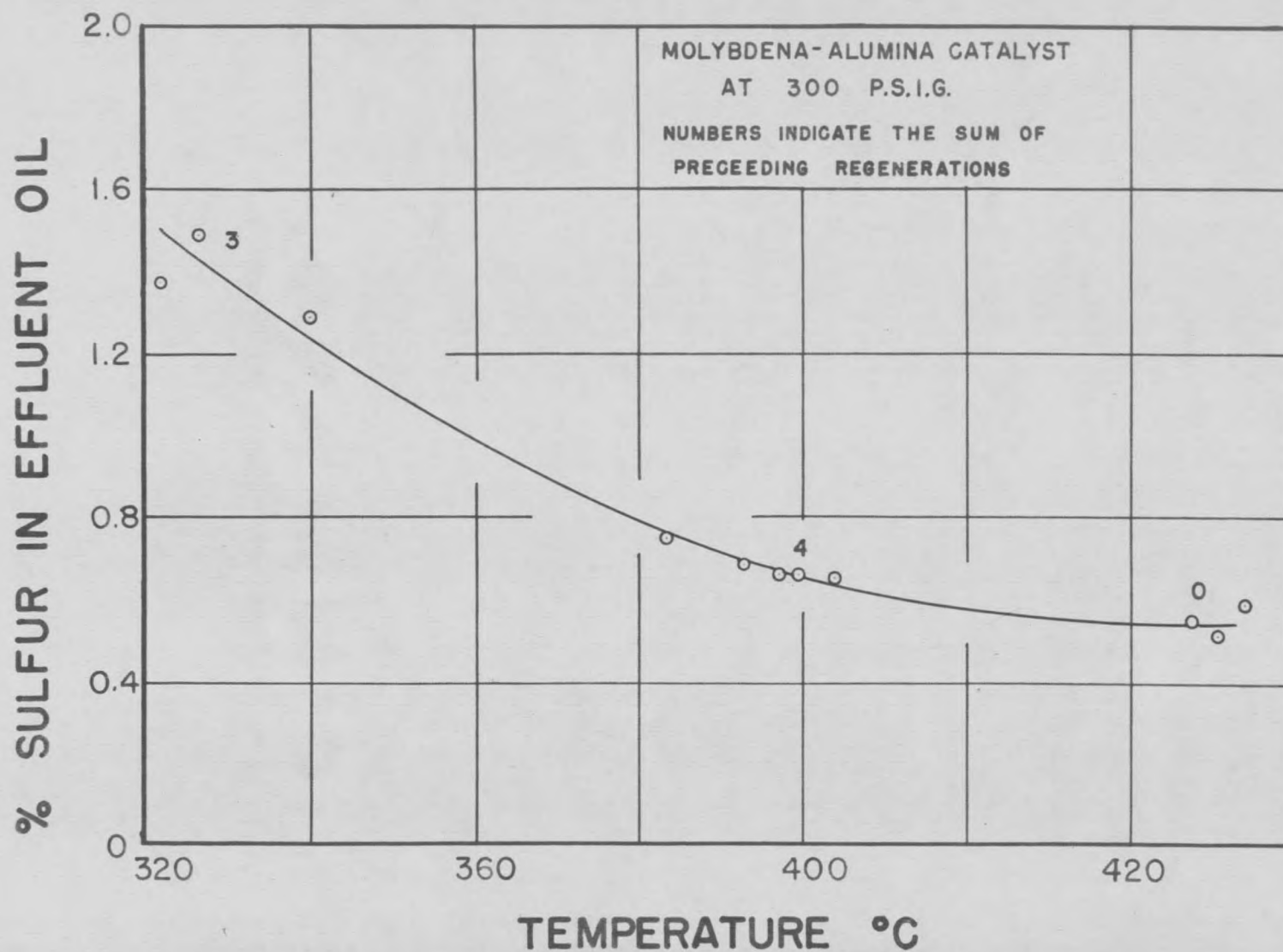
Fig. 11 Plot of Temperature vs. Desulfurization with Molybdena-alumina
