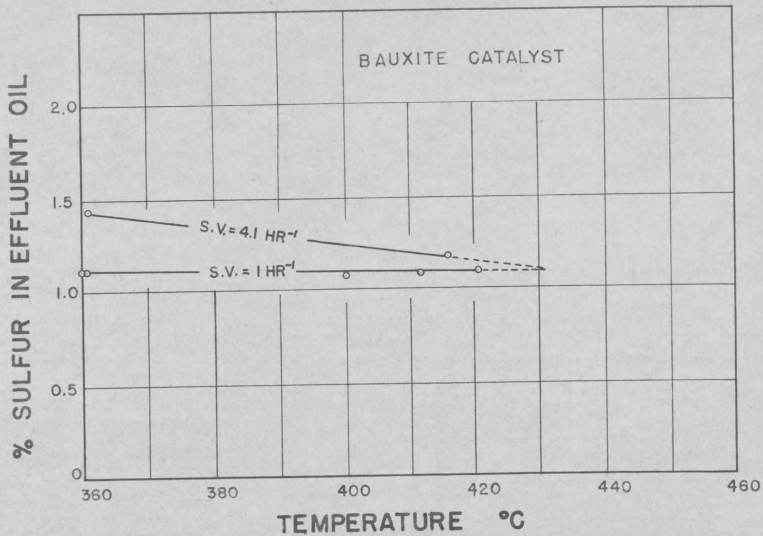
Fig. 8 Plot of Temperature vs. Desulfurization with Bauxite
