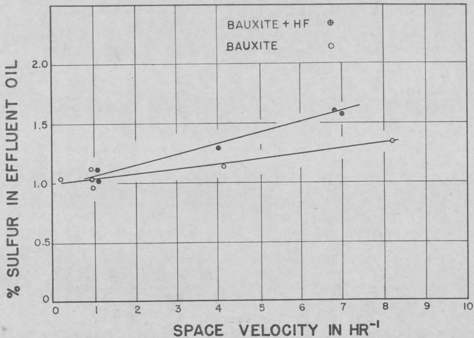
Fig. 9 Plot of Space Velocity vs. Desulfurization with HF and Bauxite
