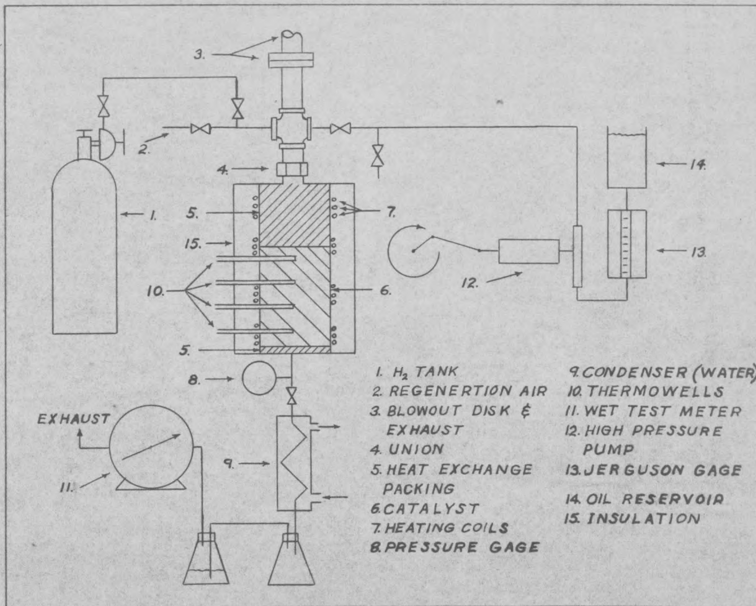
Fig. 1 Diagram of Hydrogenation Equipment for Super-atmospheric Work
