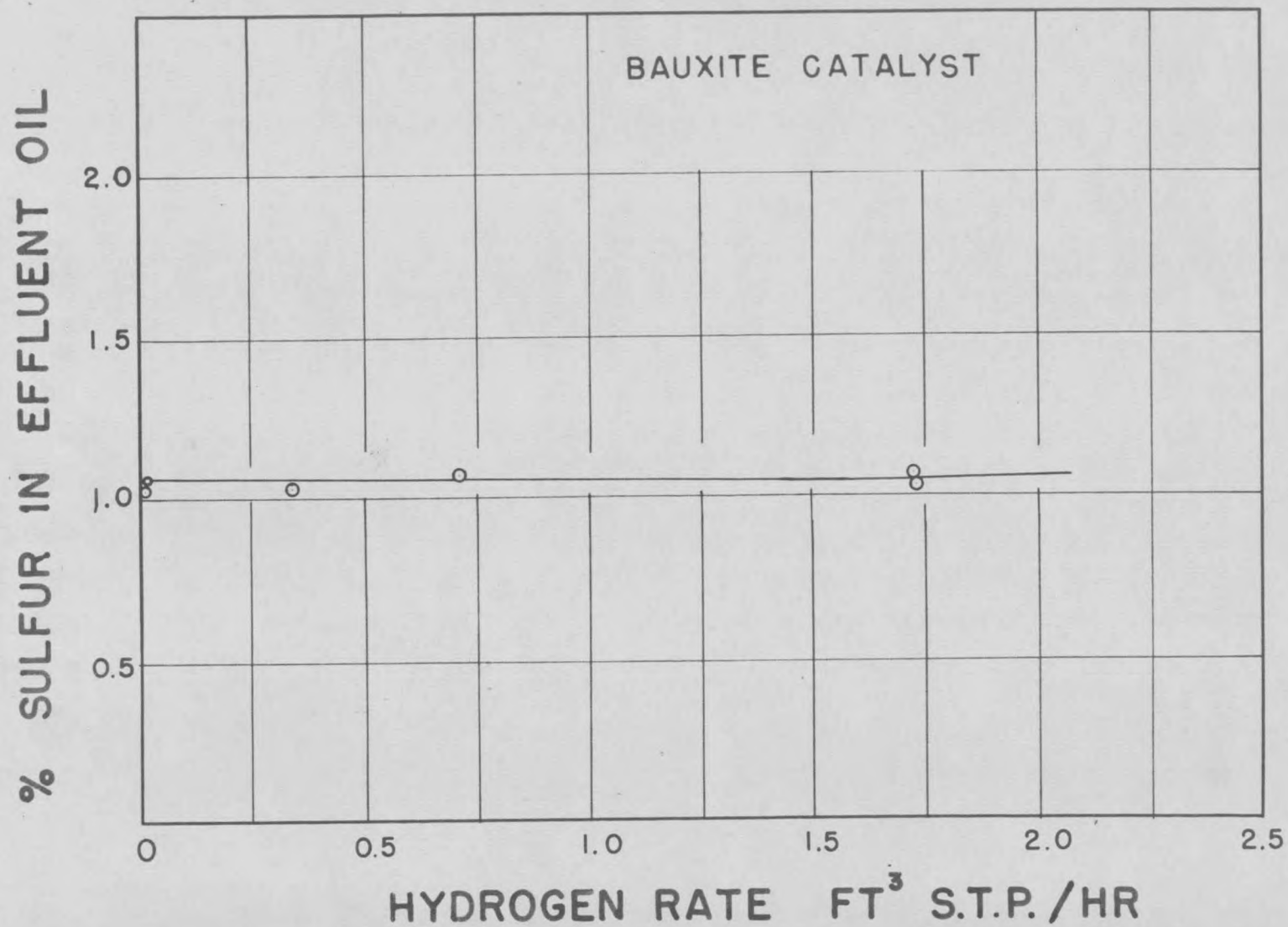
Fig. 7 Plot of Hydrogen Rate vs. Desulfurization with Bauxite
