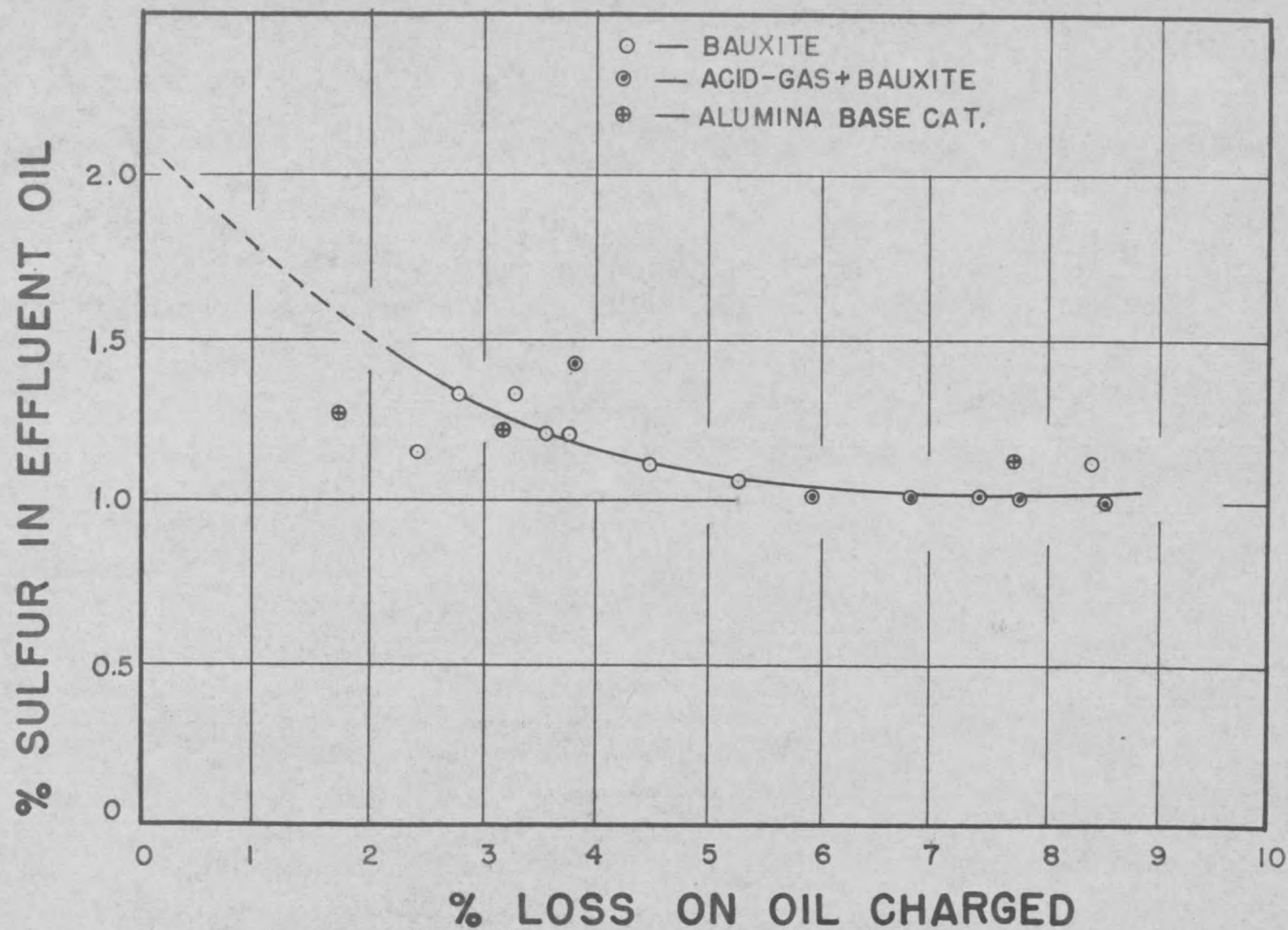
Fig. 10 Plot of % Loss on Charge vs. Desulfurization
