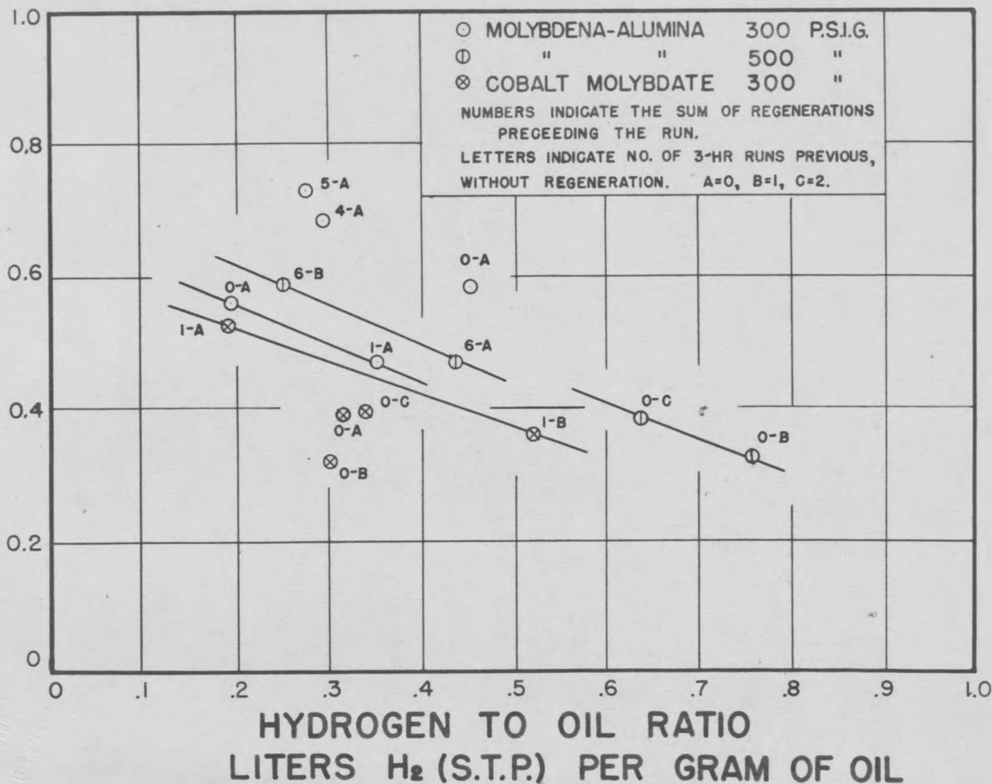
Fig. 13 Plot of Hydrogen to Oil Ratio vs. Desulfurization With Molybdena-alumina and Cobalt Molybdate
