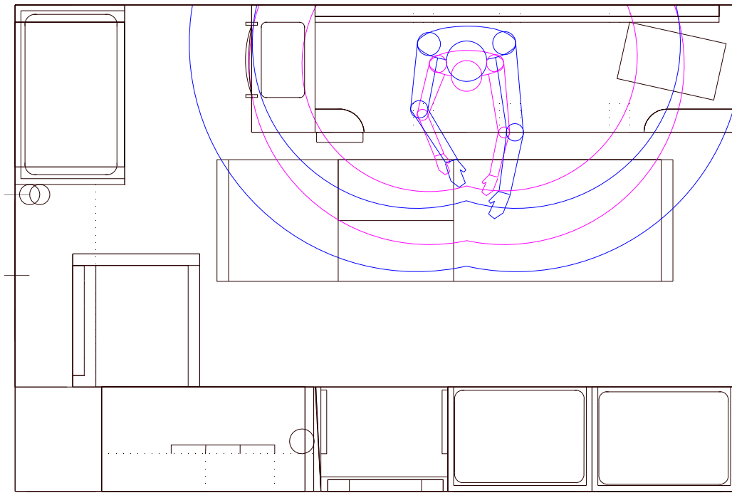
Figure 16. Overhead View of Rear Patient Compartment with Reach Envelopes: 5% Female and 95% Male
