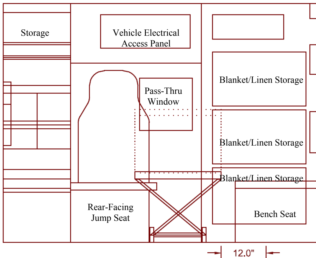
Figure 4. View of Front Wall in Rear Ambulance Cabin
