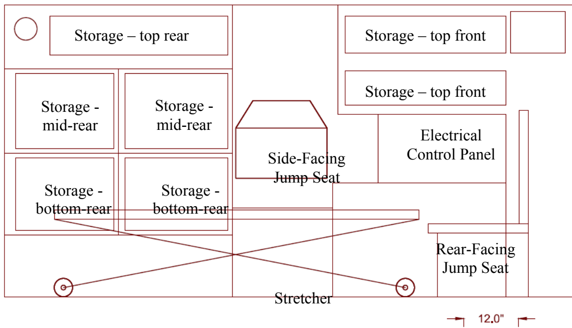
Figure 2. Side View: Driver's Side Wall
