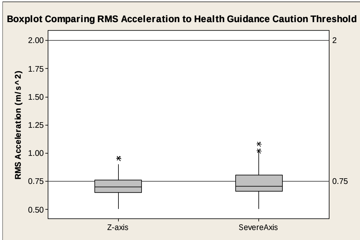
Figure 10. RMS Acceleration and Health Threshold Boxplot
