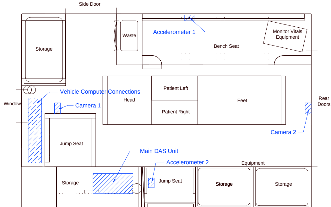
Figure 5. Overhead View of Ambulance and DAS Components ← 20" →
