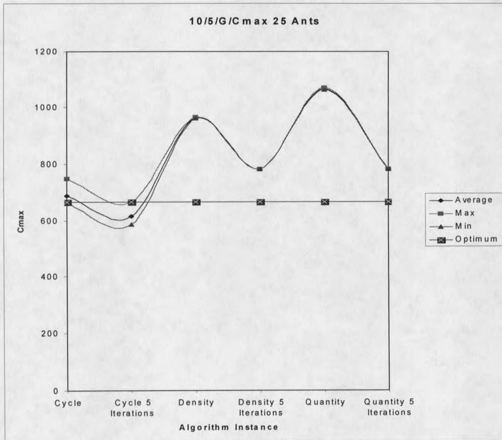
Figure 9: la01 problem instance with 25 ants
