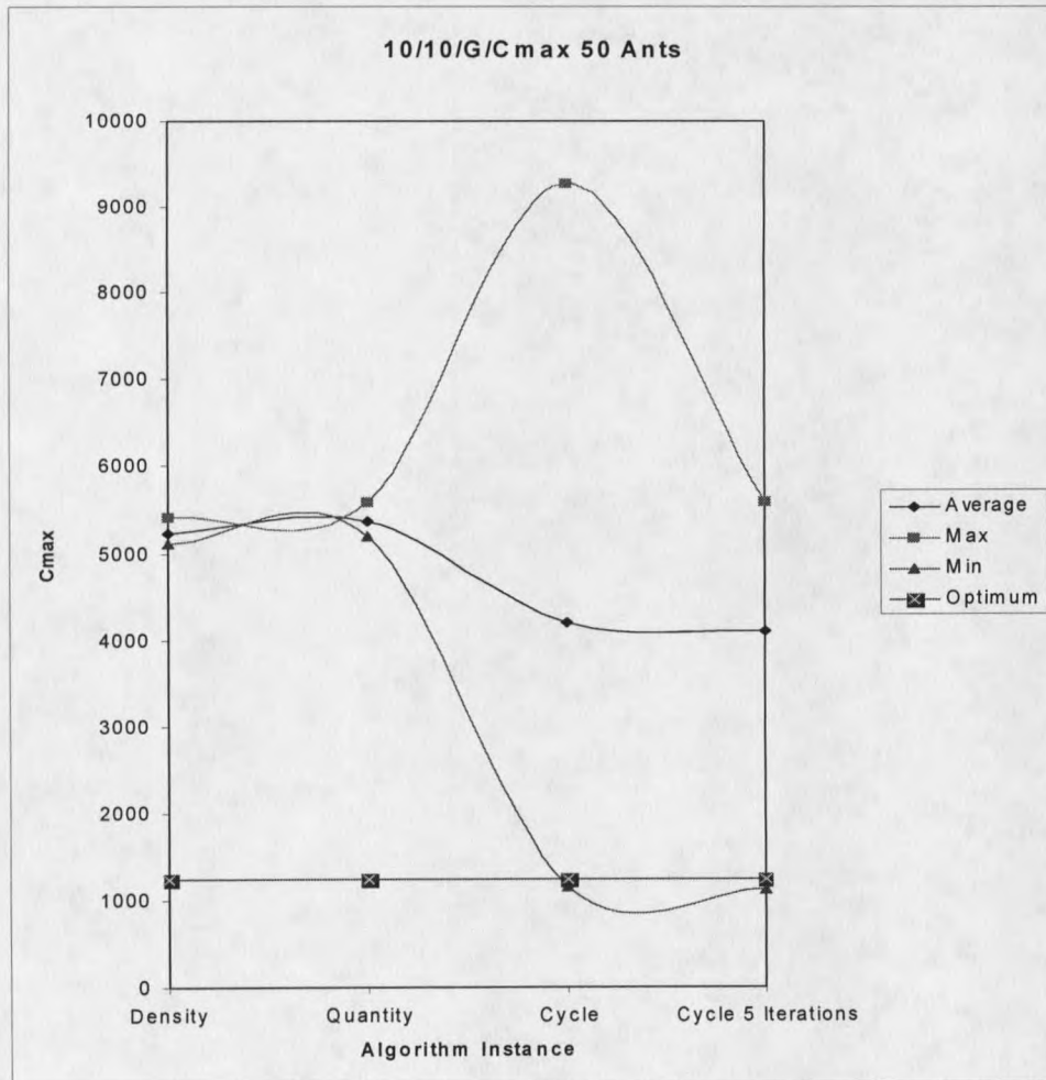
Figure 11: abz5 problem instance with 50 ants
