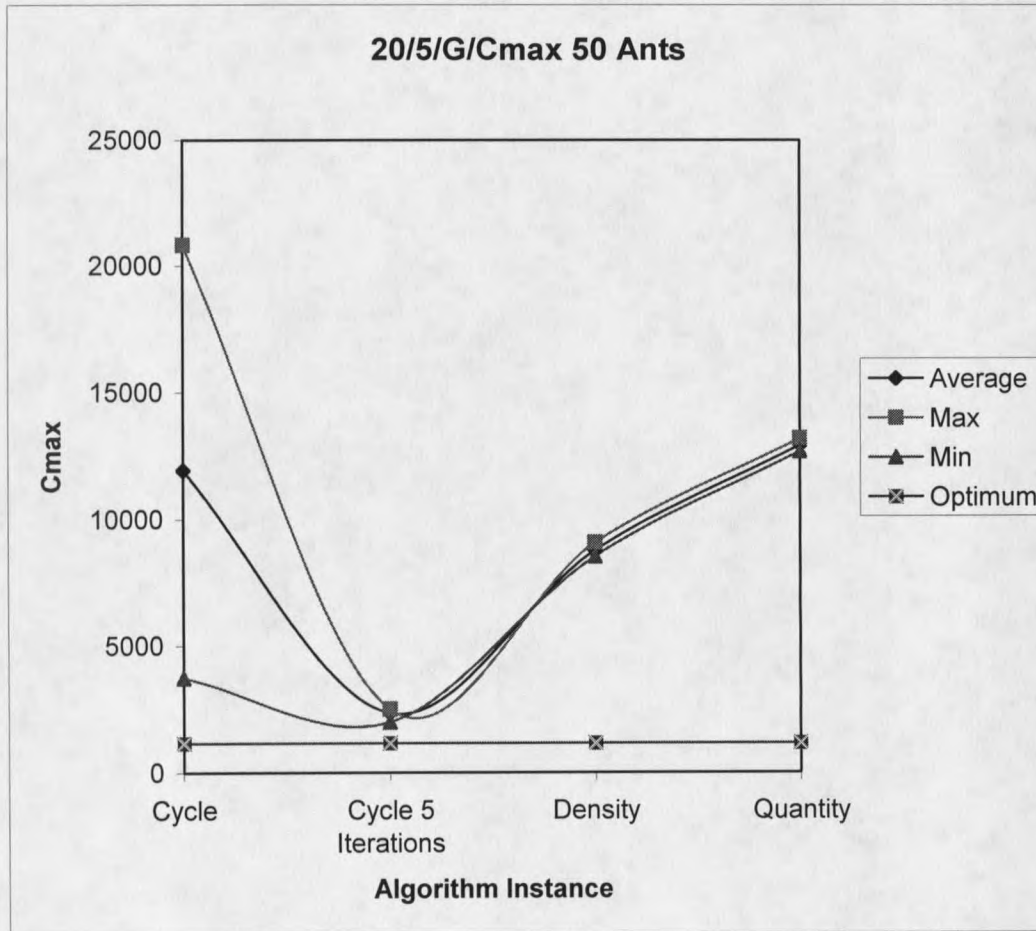
Figure 13: ft20 problem instance with 50 ants
