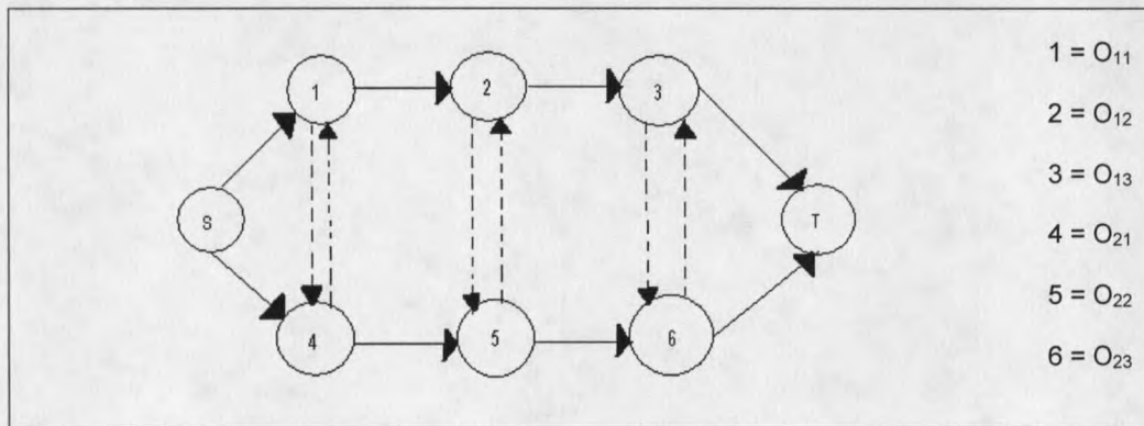
Figure 7: Representation of a 2/3/G/C_{max} job shop problem.
