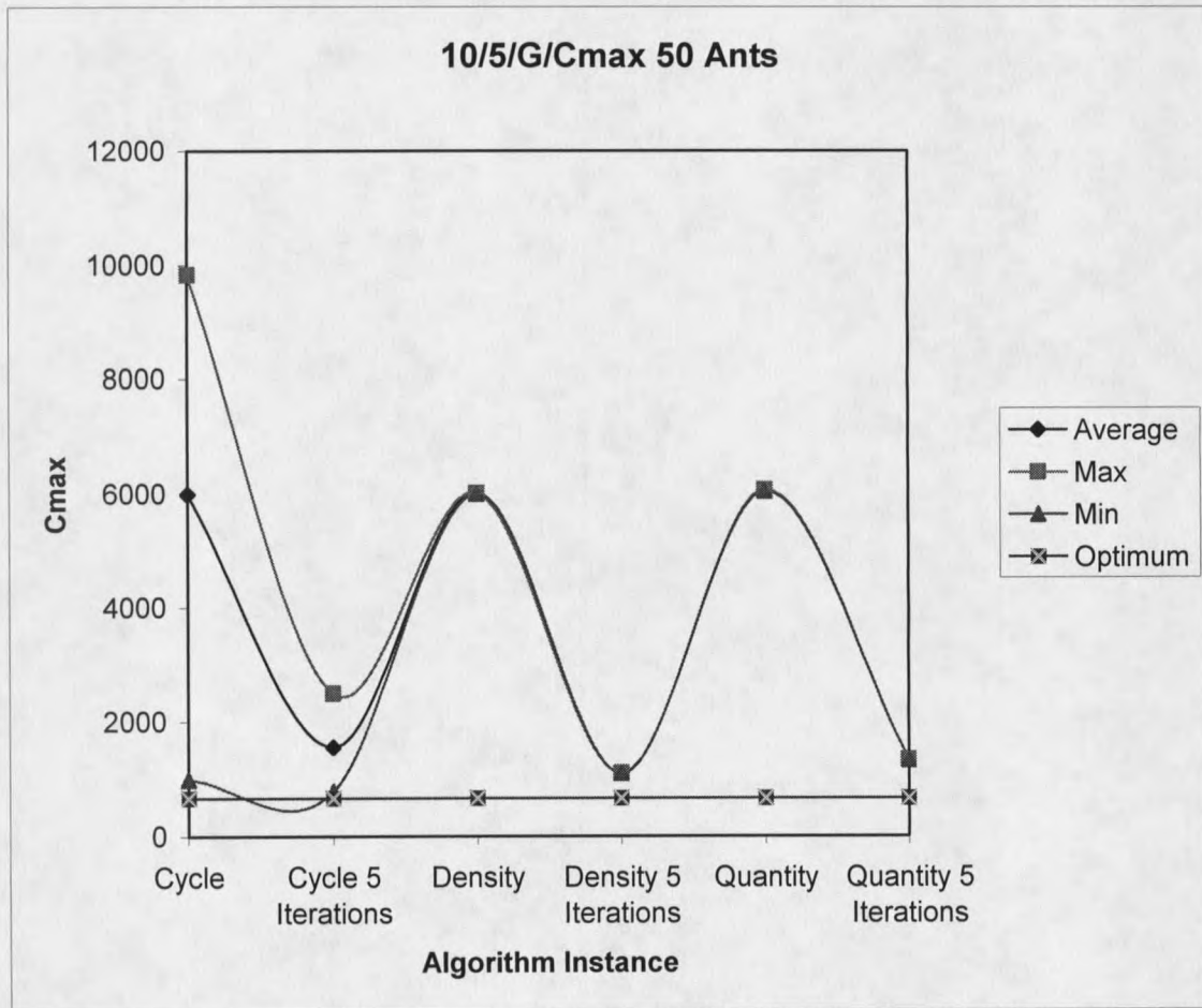
Figure 10: la01 problem instance with 50 ants
