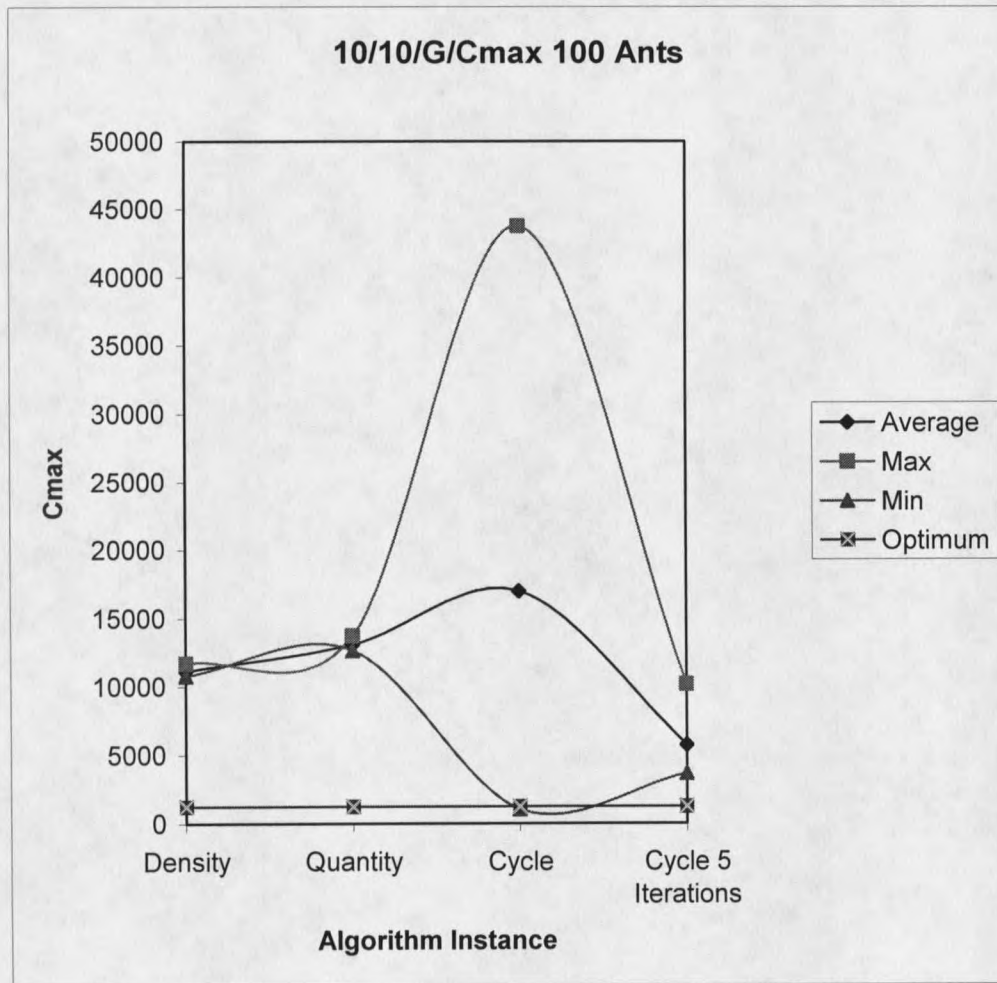
Figure 12: abz5 problem instance with 100 ants
