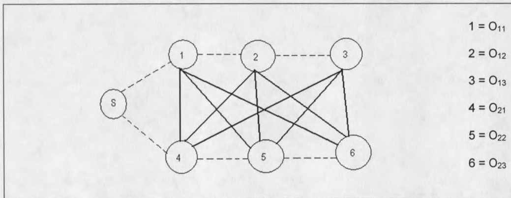
Figure 8: The AS representation of the JSP in Figure 7.
