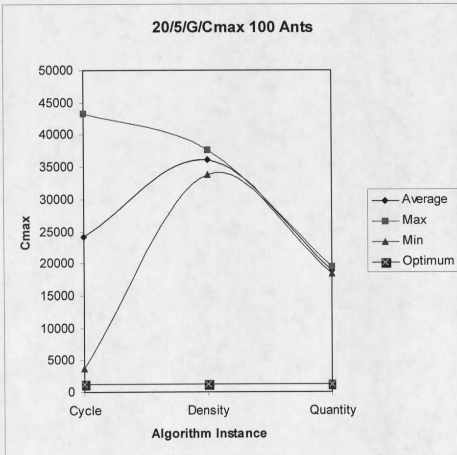
Figure 14: ft20 problem instance with 100 ants
