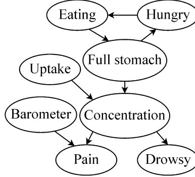
Fig. 1. Example CTBN drug network.
