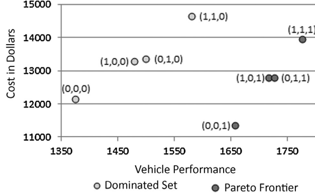
Fig. 11. Performance estimates of Cost displayed as a function of VehiclePerformance. Each datapoint is labeled with the assignment of technicians in the form (Technician1, Technician2, Technician3).
