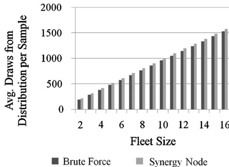
Fig. 6. Average number of draws from an exponential or multinomial distribution per sample of the brute force and synergy node approaches.
