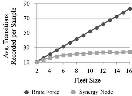
Fig. 5. Average number of transitions per sample of the brute force and synergy node approaches.
