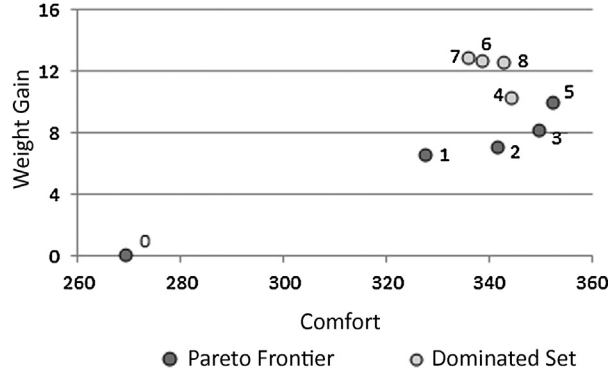
Fig. 9. Performance estimates of WeightGain displayed as a function of Comfort. Each datapoint is labeled with the number of dose applications.
