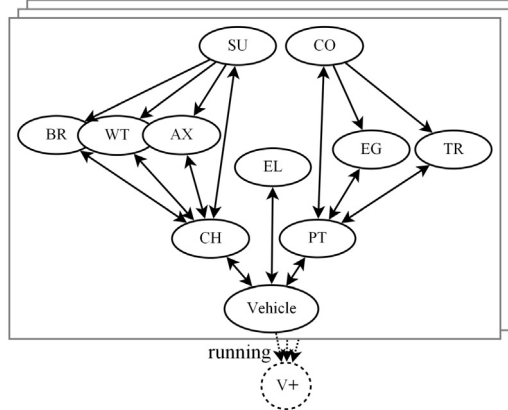
Fig. 3. CTBN for fleet of vehicles with synergy node.
