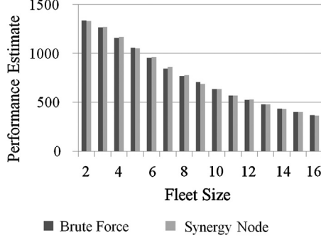
Fig. 4. Performance estimates of the brute force and synergy node approaches.
