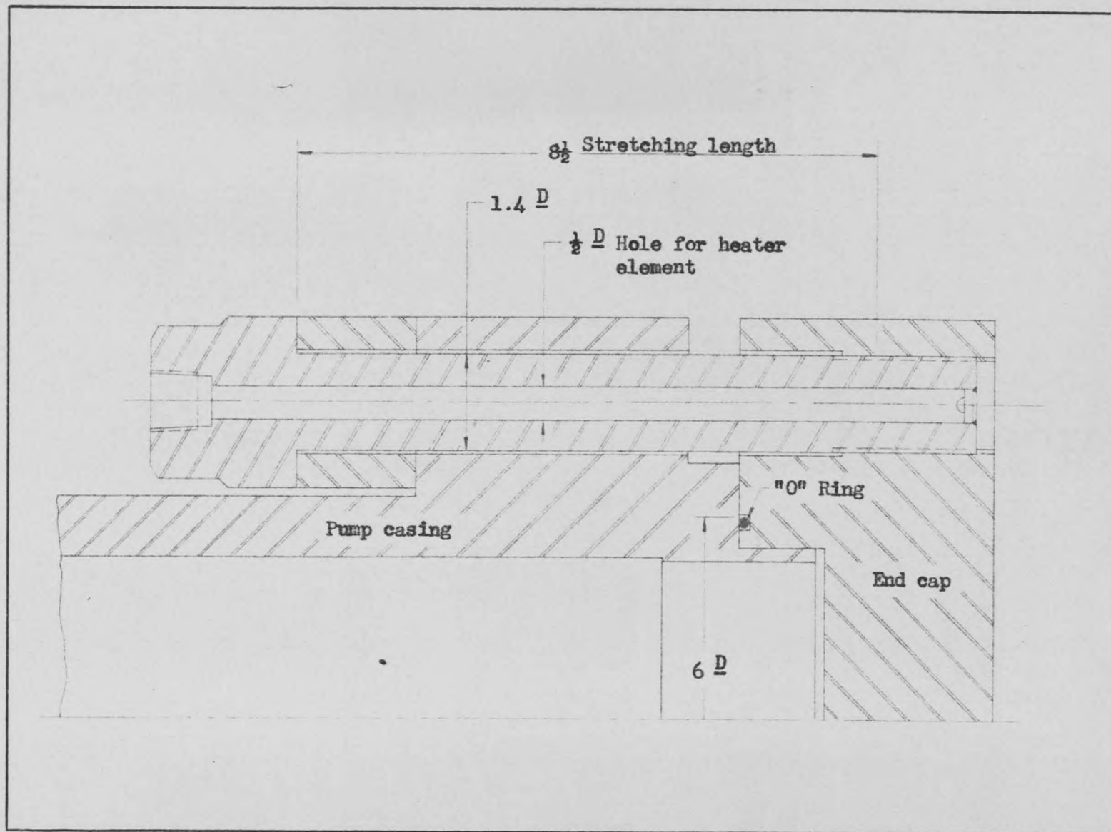
Fig. 50 - Pump casing flange assembly.
