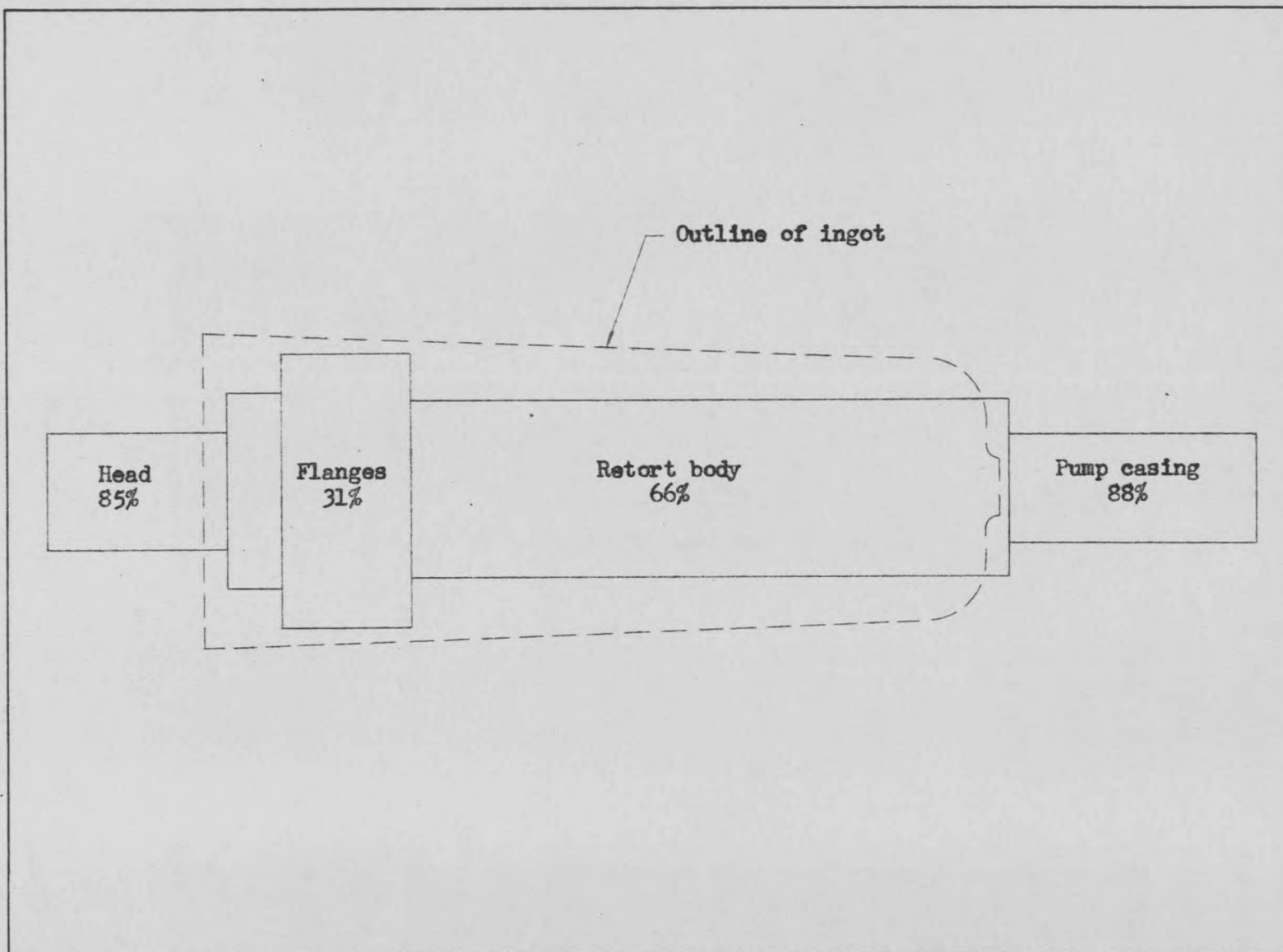
Fig. 2 - Per cent reduction of area by forging.
