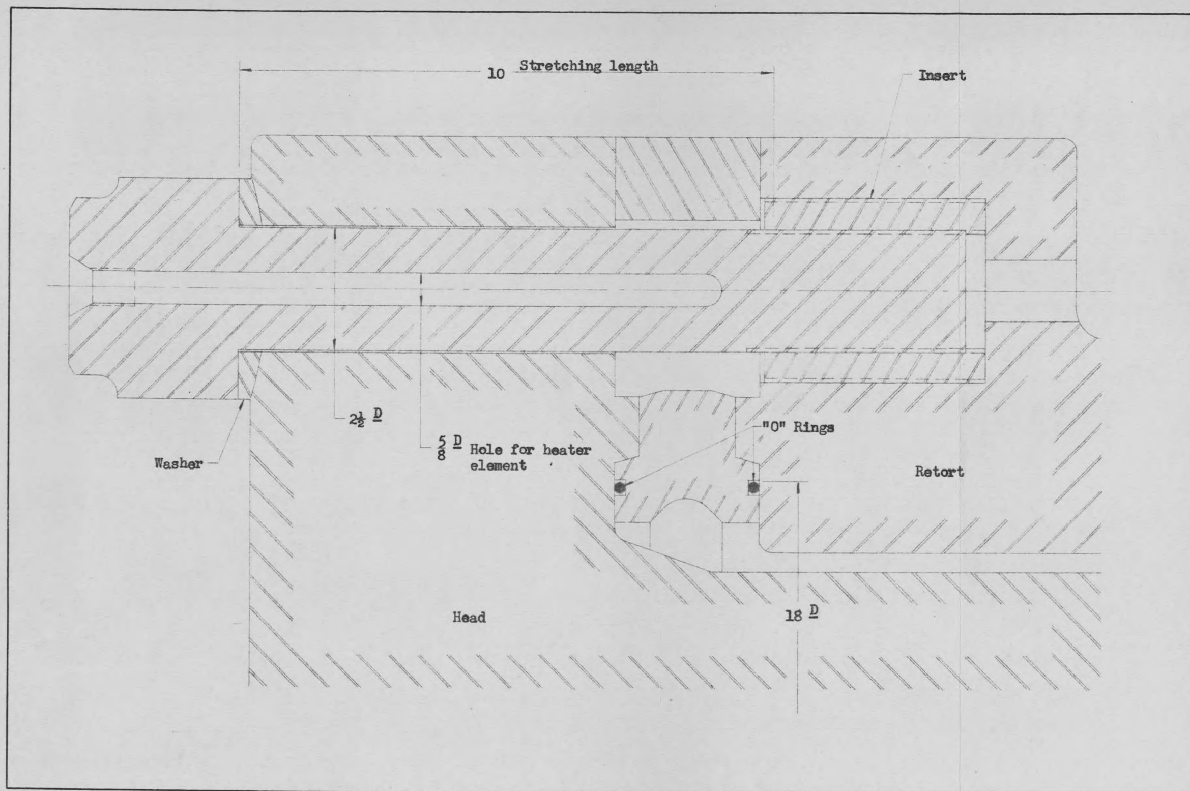
Fig. 49 - Head flange assembly.
