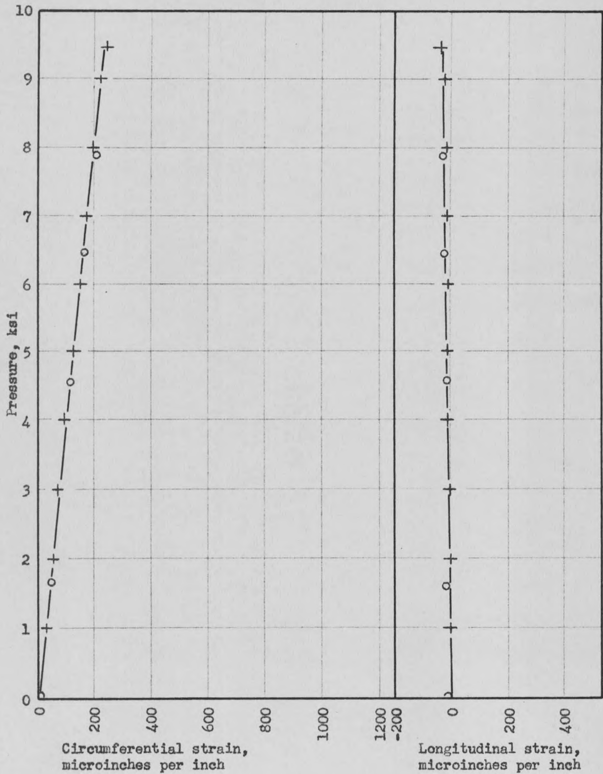
Fig. 41 - Pressure vs strain at section J, test #3.
