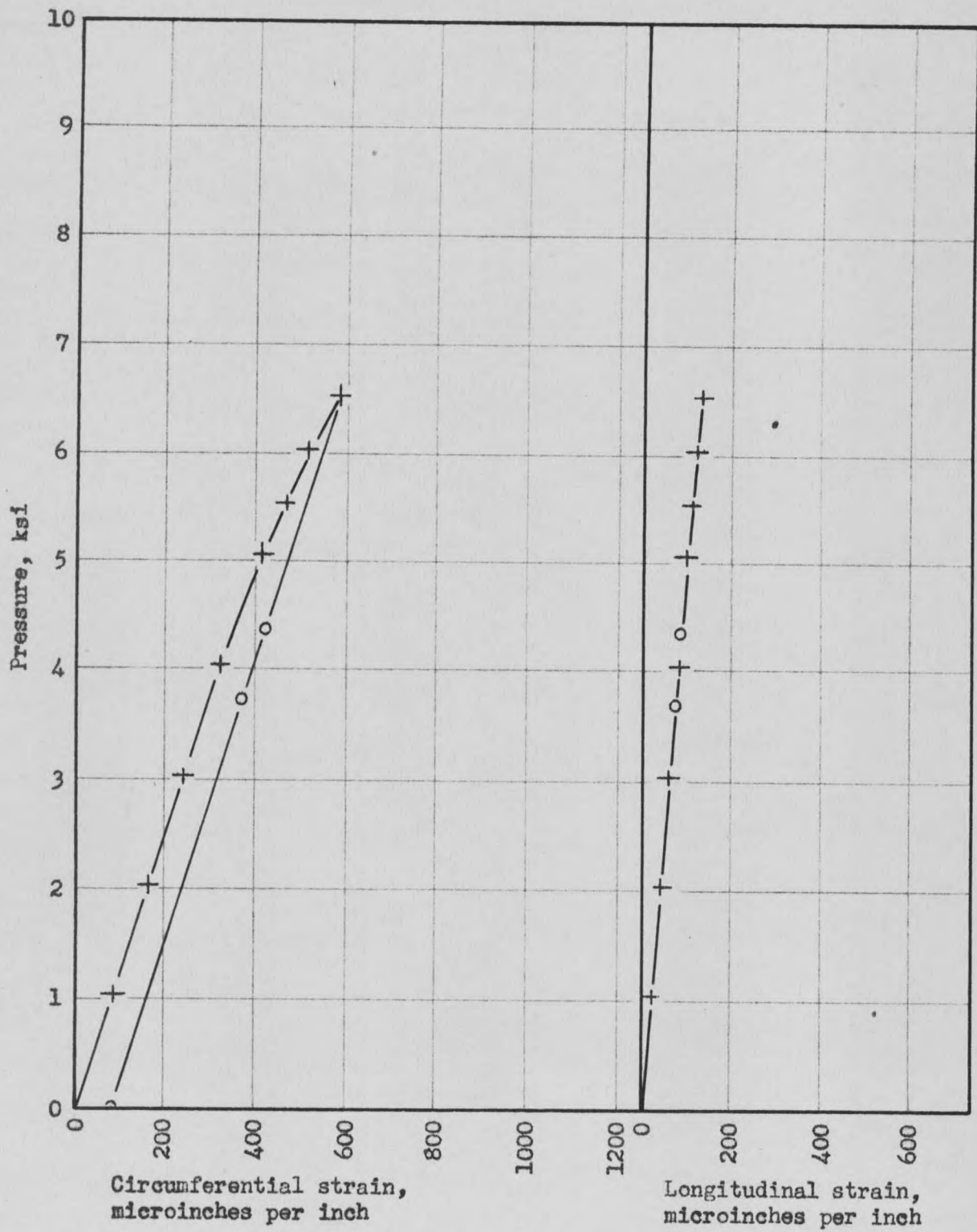
Fig. 45 - Pressure vs strain at section L, test #1.
