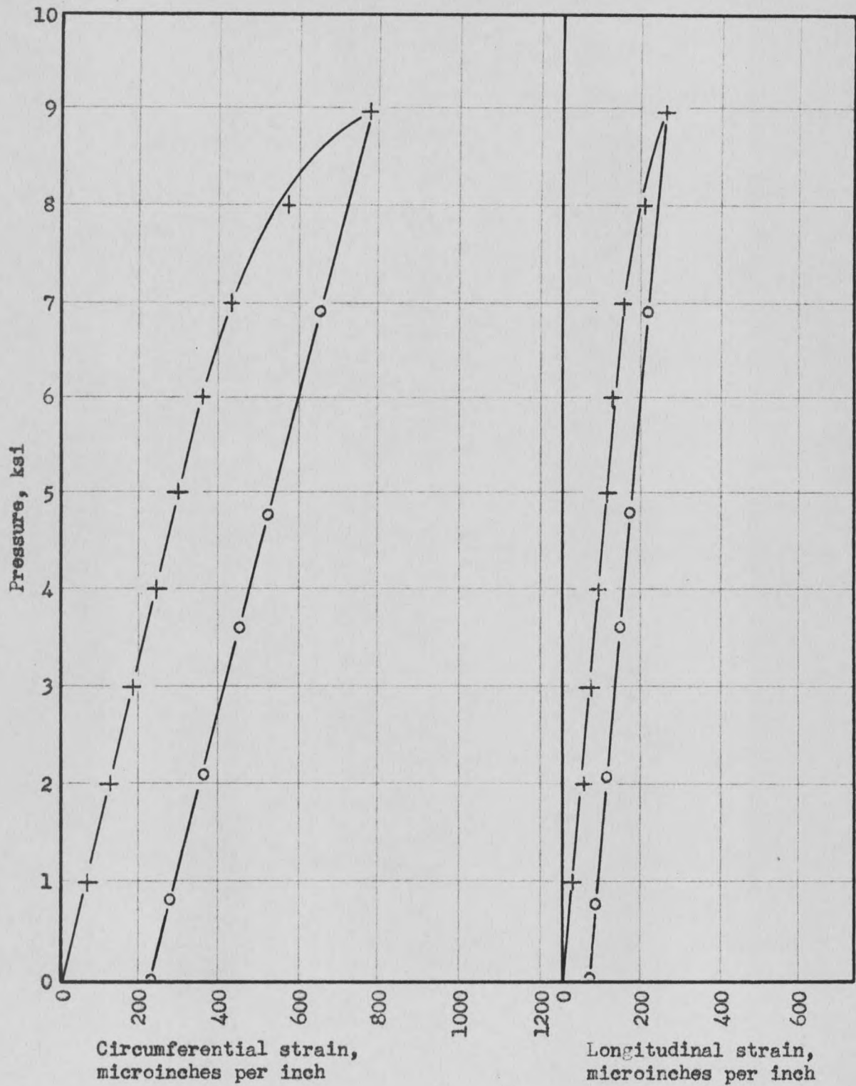
Fig. 47 - Pressure vs strain at section M, test #2.
