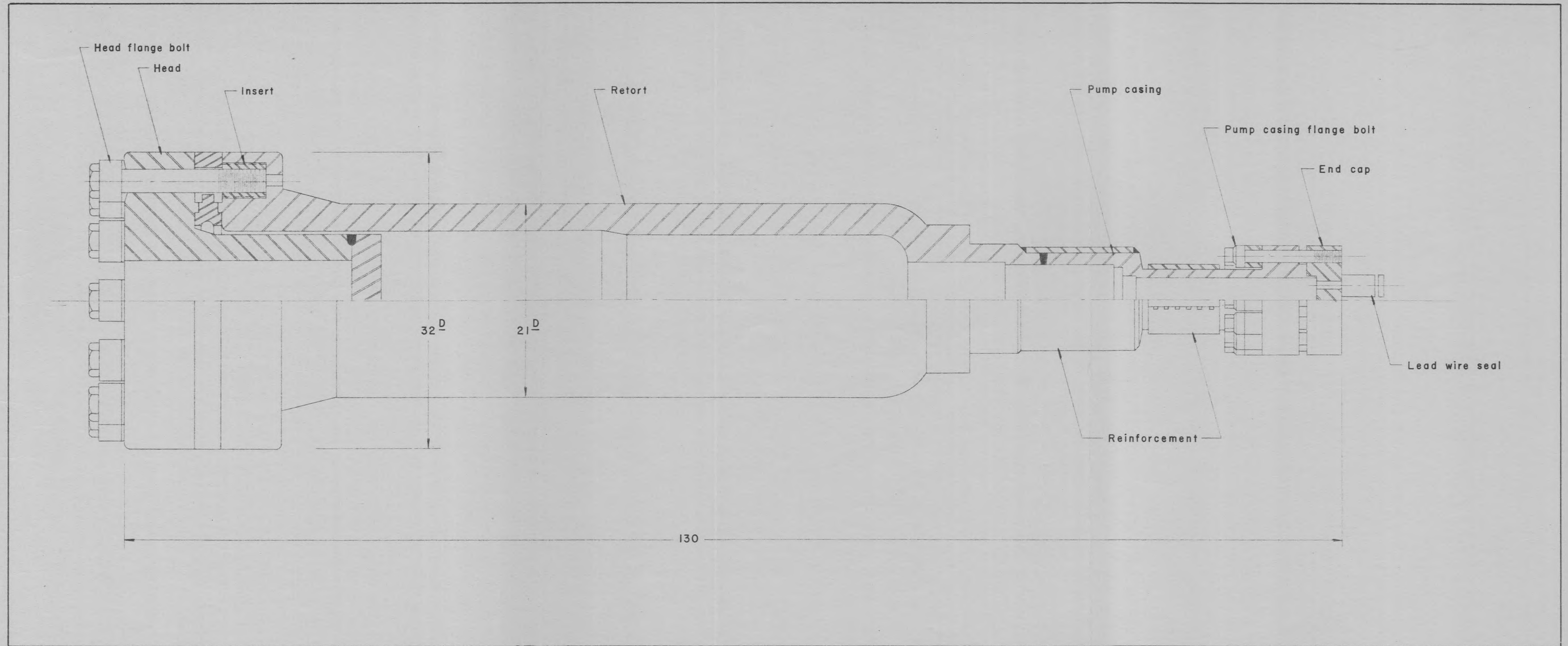
Fig. 1 — Reactor assembly.
