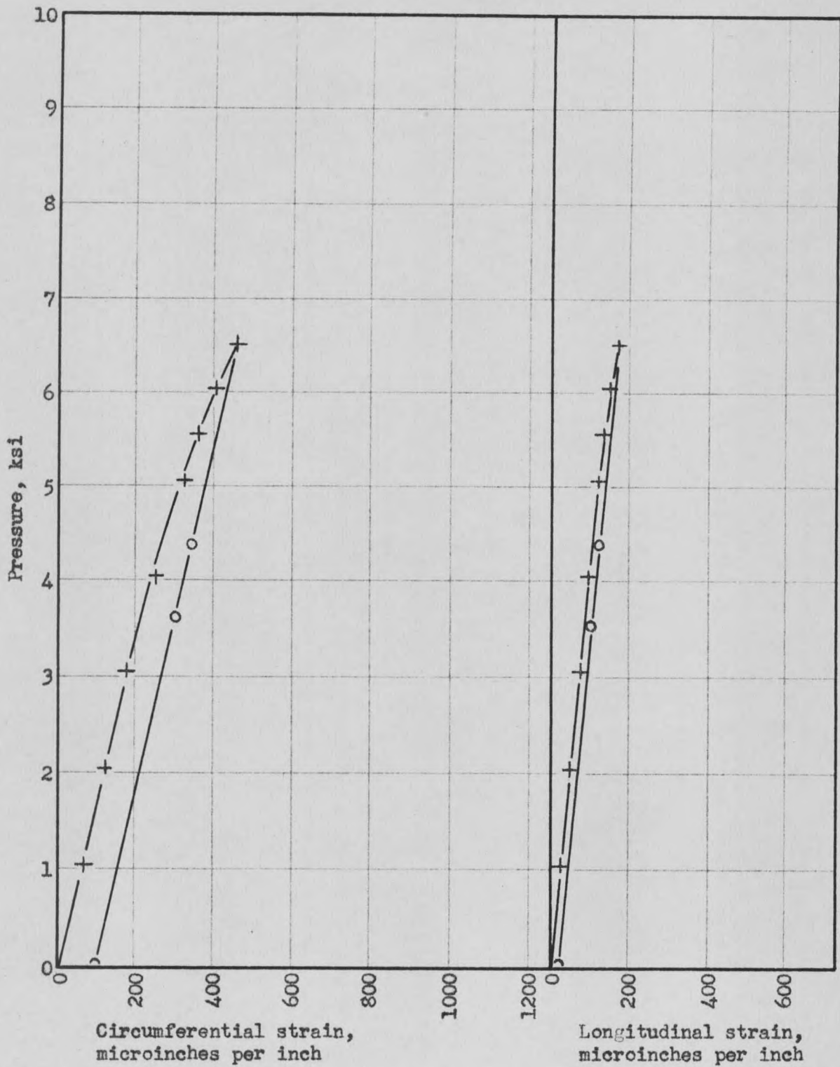
Fig. 46 - Pressure vs strain at section M, test #1.
