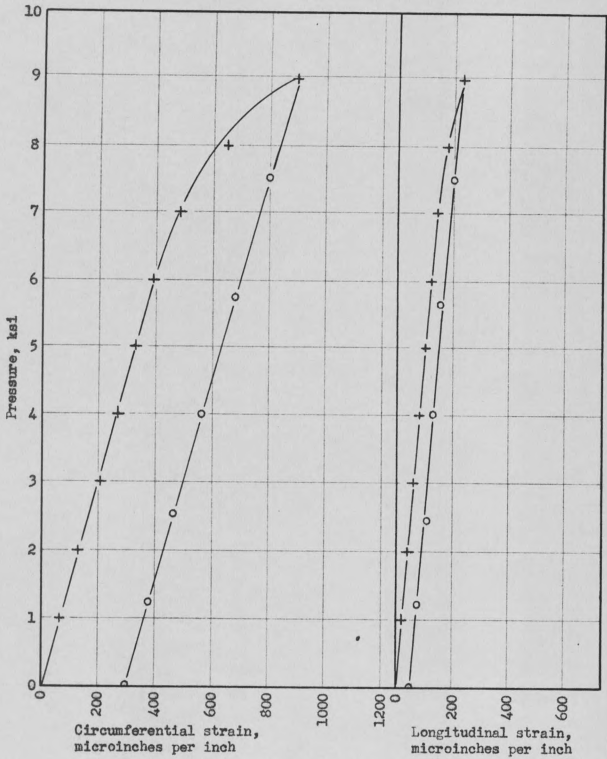
Fig. 19 - Pressure vs strain at section C, test #2.
