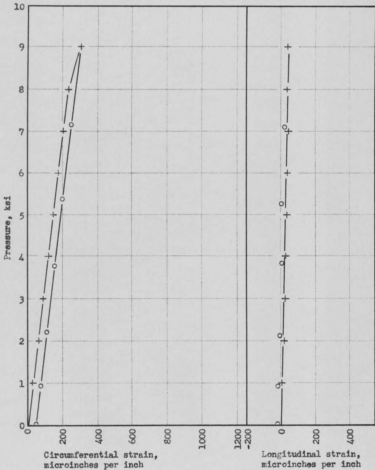
Fig. 37 - Pressure vs strain at section I, test #2.
