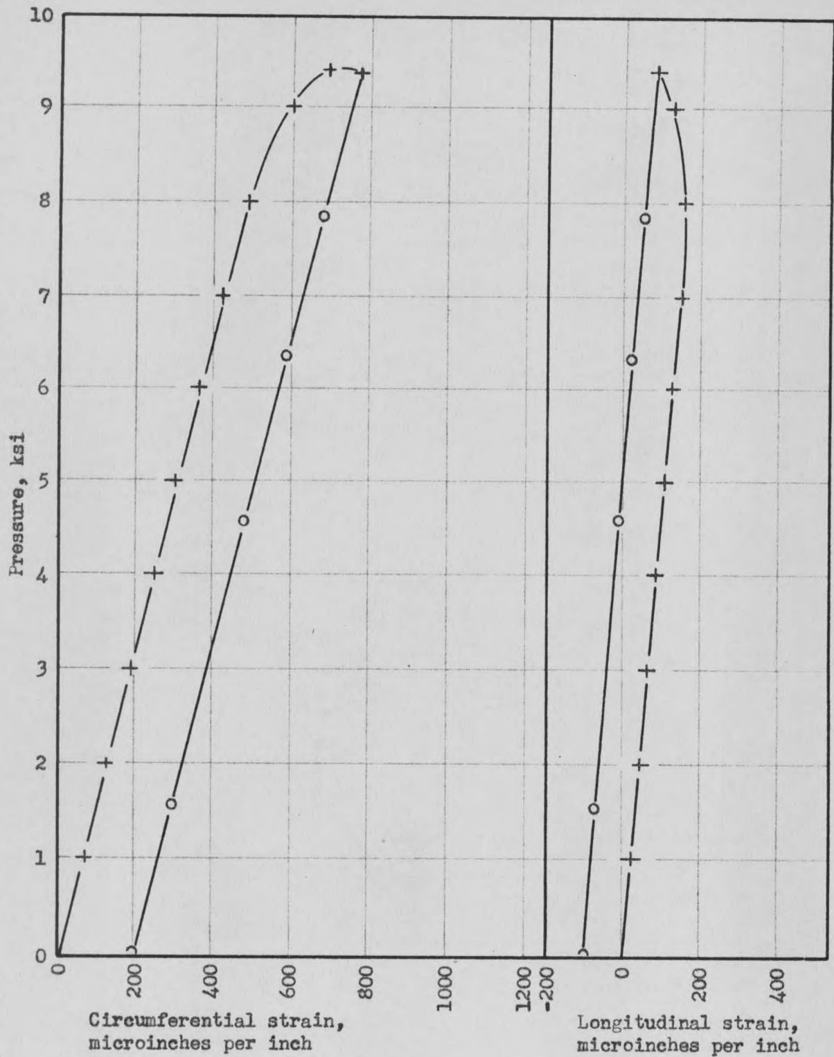
Fig. 48 - Pressure vs strain at section M, test #3.
