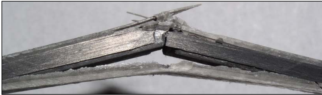
Figure 36: Three-point bending test result showing that the secondary resin had peeled off the pultrusion
