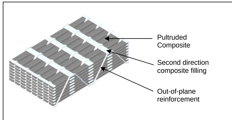
Figure 16: Schematic showing 3-D fabric
