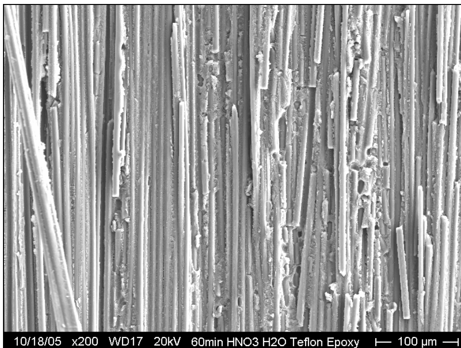
Figure H-36: Magnified view of post-tested secondary epoxy interface surface from washed 60 min \text{HNO}_3 treated rod with Teflon spacing
