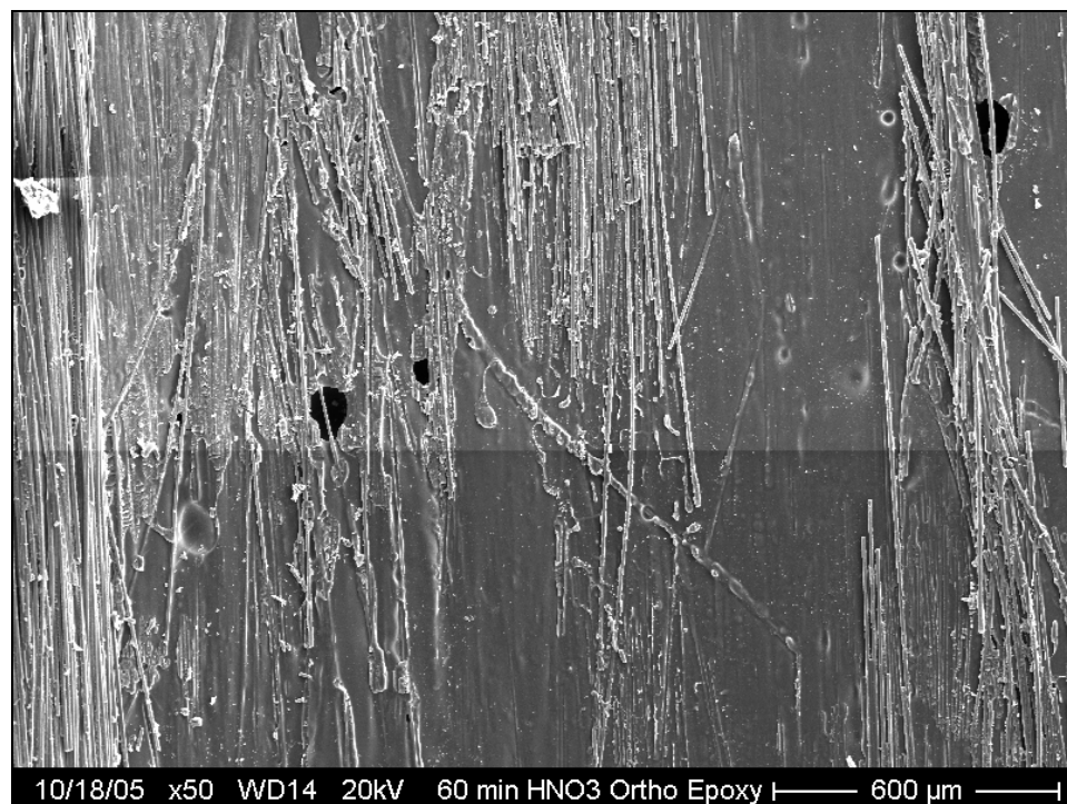
Figure H-30: Post-tested secondary epoxy interface surface from unwashed 60 min \text{HNO}_3 treated rod with ortho spacing
