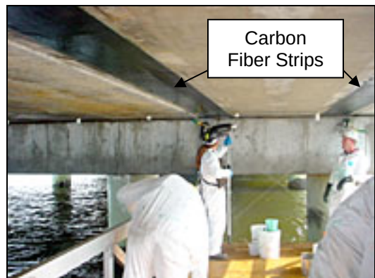
Figure 21: Bridge Strengthening [33]
