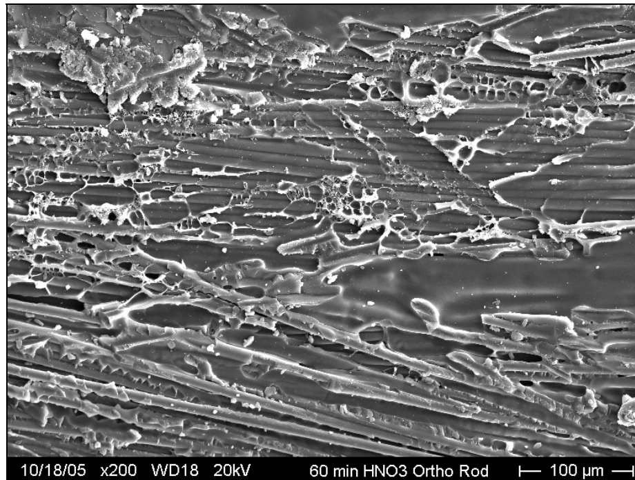
Figure H-31: Post-tested unwashed 60 min \text{HNO}_3 treated rod surface with ortho spacing
