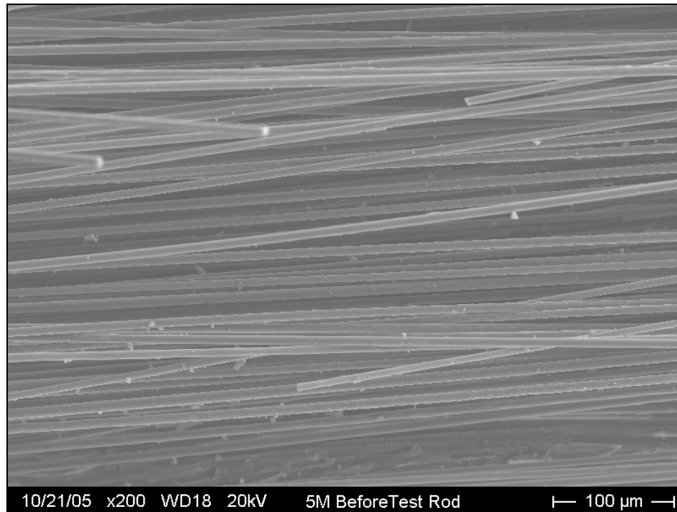
Figure 118: Pre-interface tested 60 min \text{HNO}_3 / 5M NaOH treated rod surface
