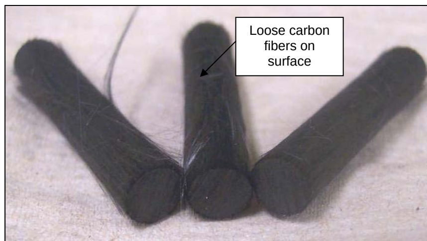
Figure 65: Rods after 30 seconds in 5M NaOH, five days distilled \text{H}_2\text{O} soak, and atmosphere drying
