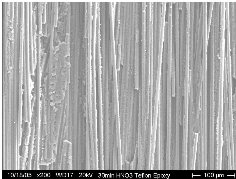
Figure H-28: Magnified view of post-tested secondary epoxy interface surface from 30 min \text{HNO}_3 treated rod
