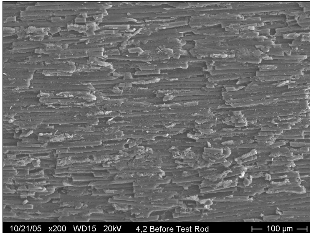
Figure 108: Pre-interface tested rod surface after the 4 kg/cm 2 , 2 revolutions erosion treatment
