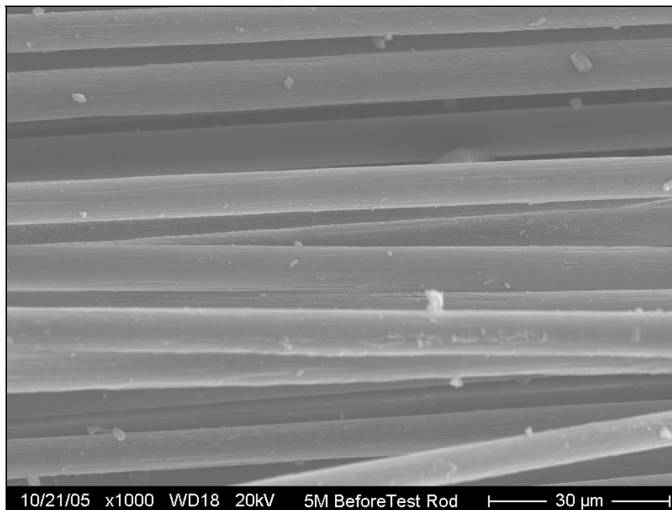
Figure 119: Magnified view of 60 min \text{HNO}_3 / 5M NaOH treated rod surface
