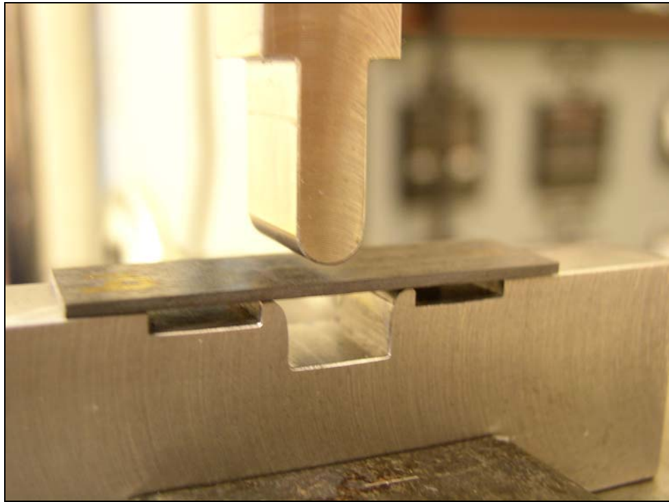
Figure 81: SBS coupon about to undergo loading
