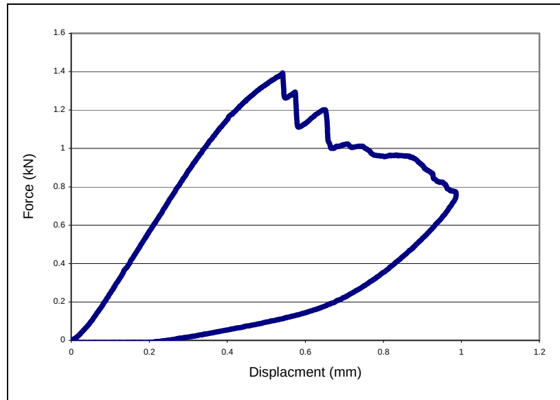
Figure 156: Typical force vs. displacement curve for a pultruded flat in short beam shear
