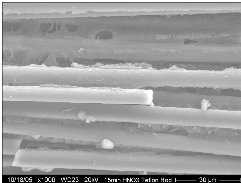
Figure 140: Close up view of 15 min \text{HNO}_3 post tested rod surface
