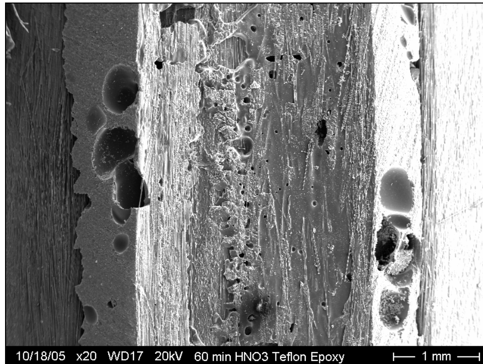
Figure H-29: Post-tested secondary epoxy interface surface from unwashed 60 min \text{HNO}_3 treated rod with Teflon spacing
