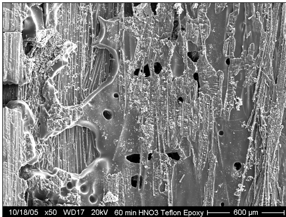
Figure 144: Post tested unwashed 60 min \text{HNO}_3 epoxy interface
