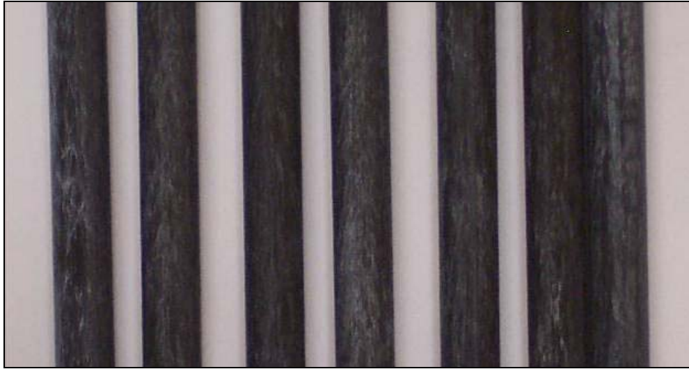
Figure 68: 15 min HNO 3 treated rod surfaces before secondary epoxy infusion
