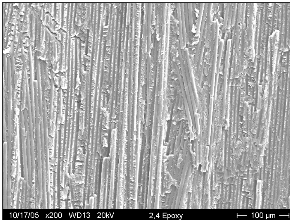
Figure 131: Post-tested secondary epoxy interface surface from (2, 4) erosion treated rod
