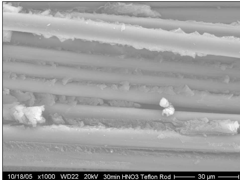
Figure H-27: Magnified view of post-tested 30 min \text{HNO}_3 treated rod surface
