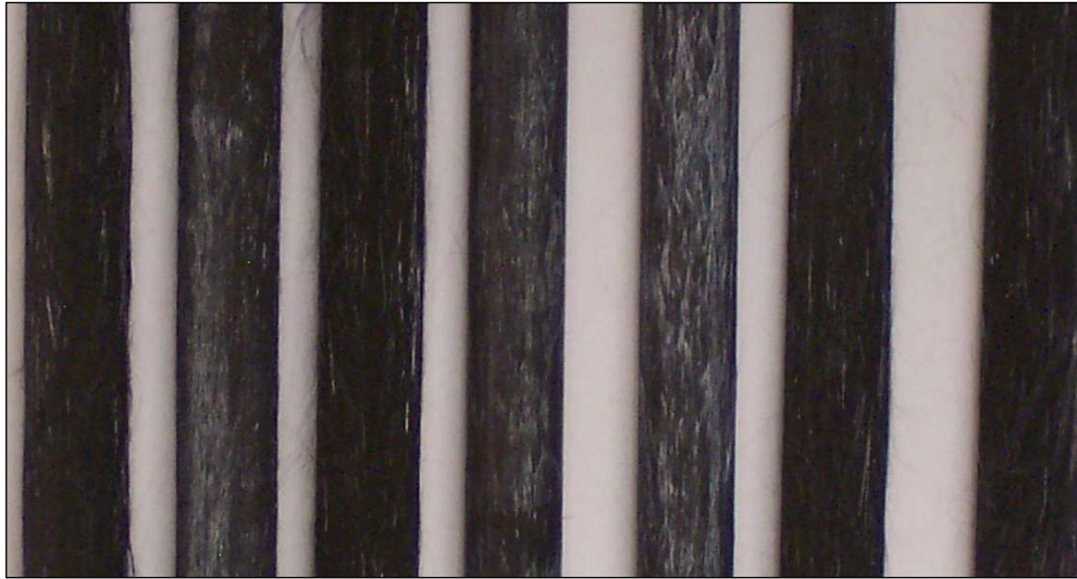
Figure 70: 60 min \text{HNO}_3 treated rod surfaces before secondary epoxy infusion
