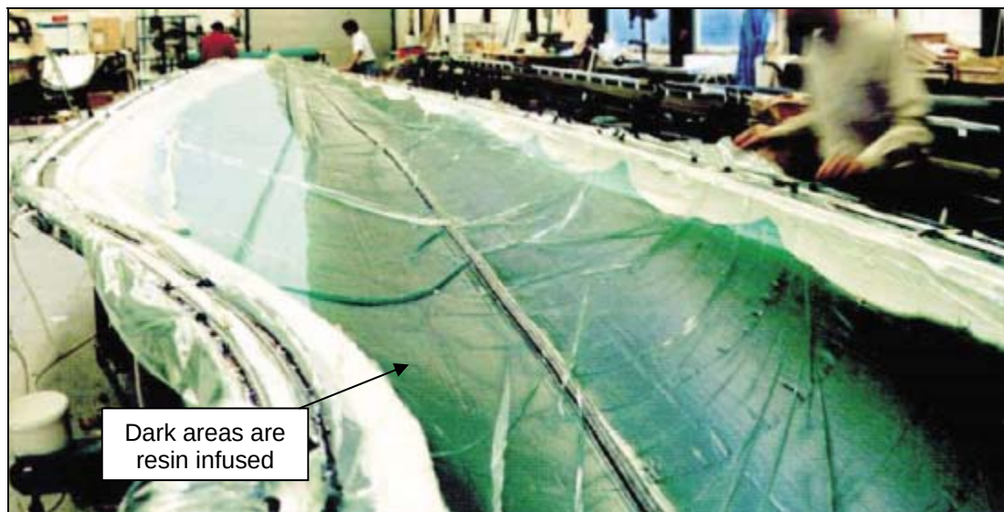
Figure 4: One half outer rotor blade skin during vacuum injection [8]
