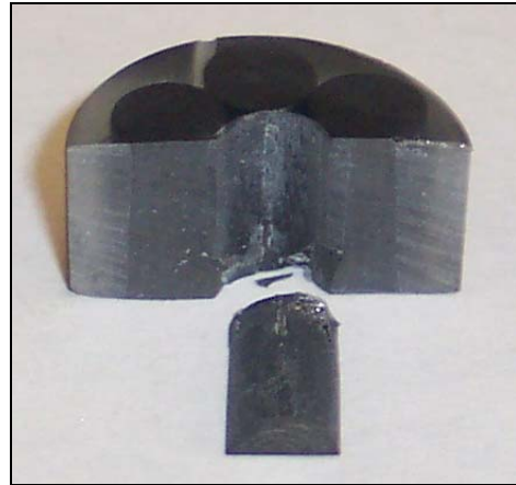
Figure 121: A closer view of the failed interface
