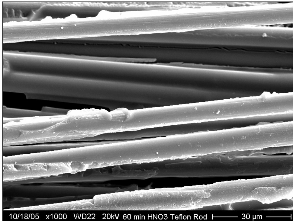
Figure 143: Magnified view of unwashed 60 min \text{HNO}_3 rod
