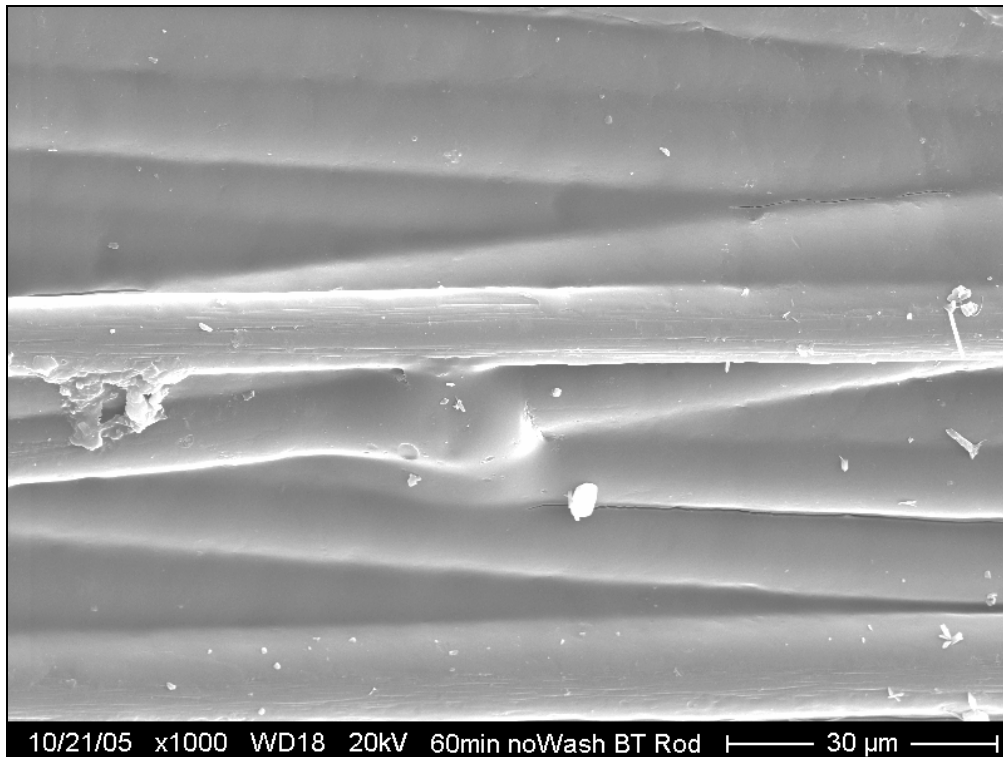
Figure 115: Magnified of the unwashed 60 min \text{HNO}_3 treated rod surface
