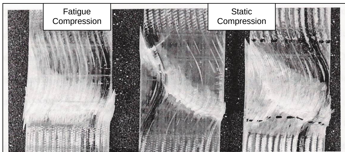
Figure 12: Static compression failure and fatigue compression failure [20]
