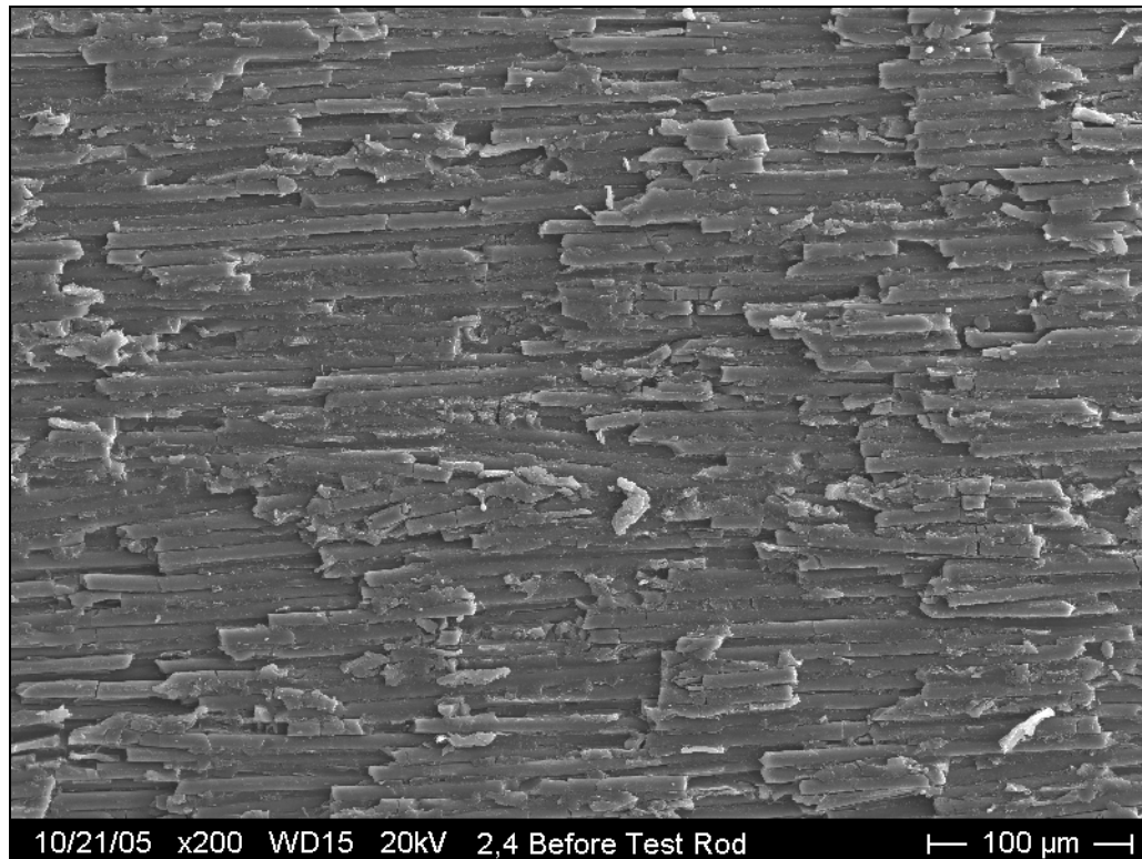
Figure 102: Pre-interface tested rod surface after the 2 \text{ kg/cm}^2 , 4 revolutions erosion treatment
