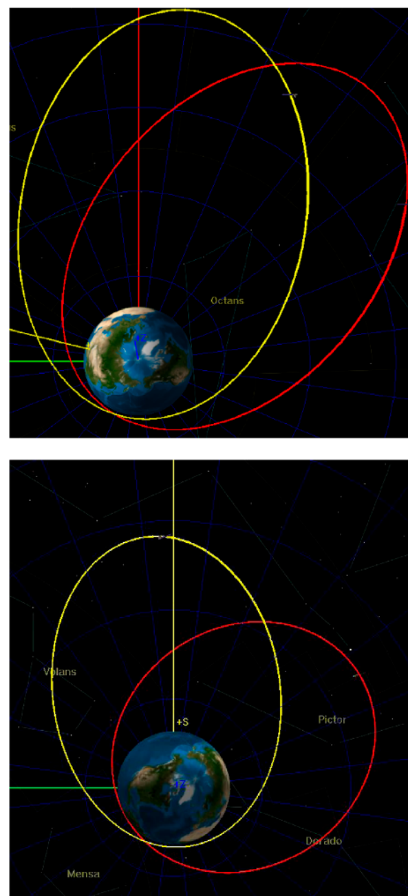
FIGURE 3 Images depicting the initial orbit configuration for the two possibilities described in this study. (Top panel) This orbit is separated by 30°, with an apogee near 6 Re, and maintains this separation for an entire precession. (Bottom panel) This orbit is separated by 30° 4 months after launch and 60°, the maximum separation, at 8 months.
