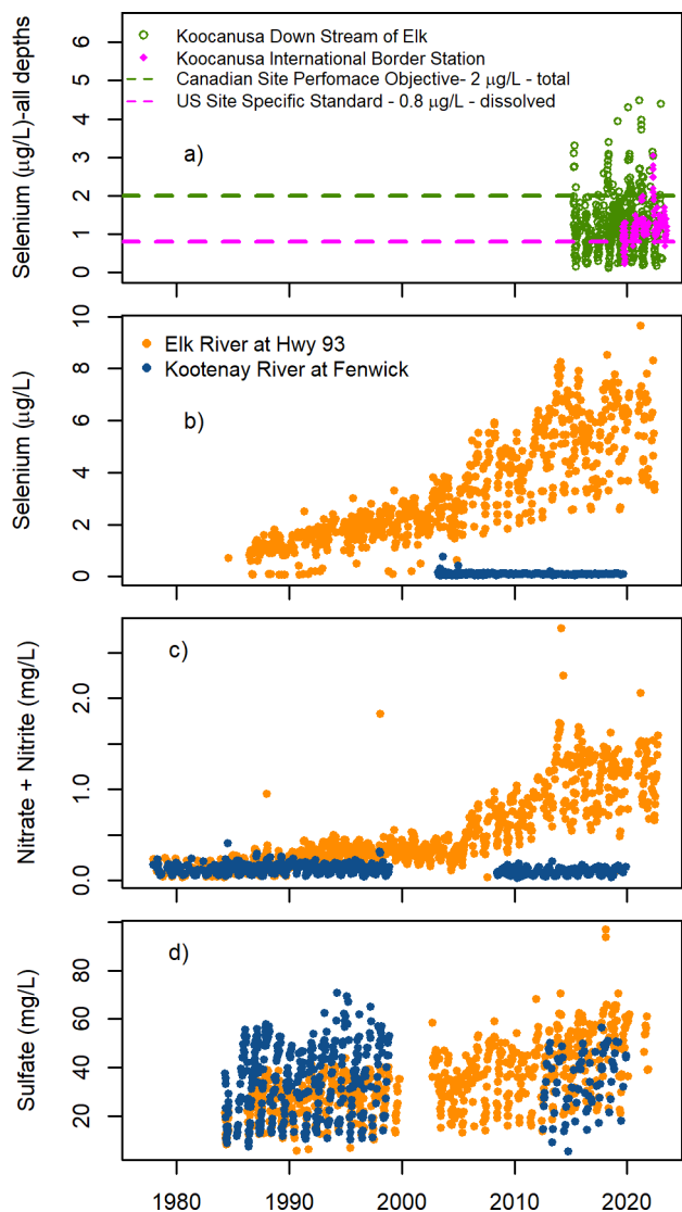
Figure 3. Solute concentration measurements in Koocanusa Reservoir, the Elk River at Highway 93 and the Kootenay River at Fenwick. 22 (a) Koocanusa Reservoir total Se concentrations measurements at a Canadian compliance point (Lake Koocanusa South of Elk River, green) 46 and dissolved Se on the United States side of the international boarder (U.S. Geological Survey Site ID 12300110, magenta) 24 with their respective regulatory criteria. 45,46 Concentration measurements of total Se (b), \text{NO}_3^- (c), and \text{SO}_4^{2-} (d) at the Elk River at Highway 93 (orange) and the Kootenay River at Fenwick (blue). 22
