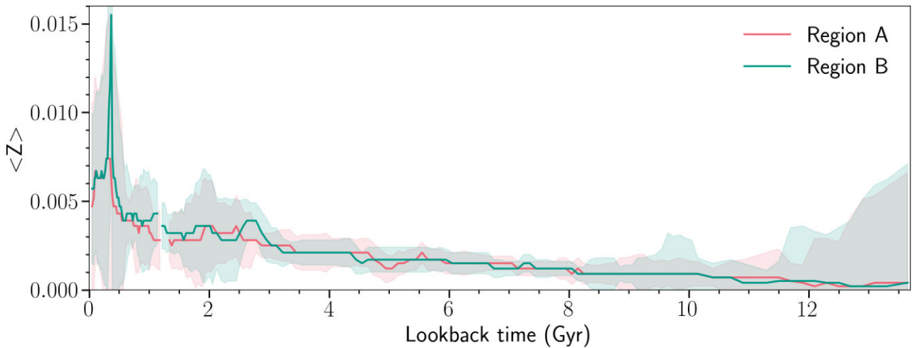
Figure 7. AMRs displaying the mean metallicity (depicted as \langle Z \rangle ) over lookback time for region A and region B after accounting for the line-of-sight depth during the SFH derivation process. Shaded areas also represent uncertainties. Here, we mask the age bins in which SFR is less than 5% of the maximum SFR for the region to avoid uncertain metallicity determinations driven by the lack of stars of such ages.
