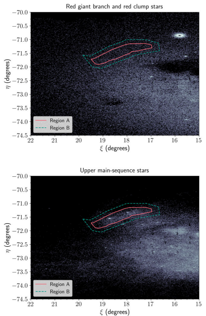
Figure 1. Top panel: spatial distribution of selected intermediate-age and older populations (red giant branch and red clump stars) across the SMC with \sim 655\,558 stars. Bottom panel: density map of the younger populations (upper MS stars) with \sim 324\,535 stars. The region containing the northeastern shell (region A) is outlined in pink, and the region used to estimate the contribution of SMC field stars to Region A is in a dashed green line (region B).
