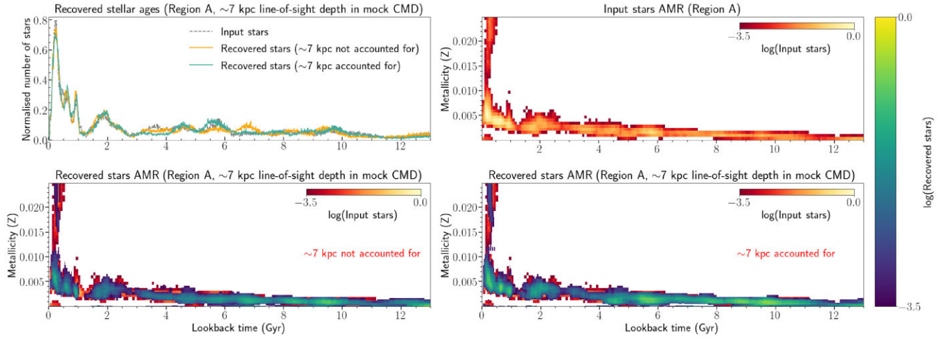
Figure A3. Age-resolution tests for a mock CMD with a ‘realistic’ SFH. The mock CMD used is region A’s solution SFH. The solution is post line-of-sight depth simulation, hence the CMD contains a line-of-sight depth of 7 kpc. To ease interpretation, we have masked AMR that is less than 3% of the maximum AMR. Top, left panel: In grey are the ages of the stars inputted into THESTORM. In yellow is the result when the 7 kpc line-of-sight depth is not accounted for in the fitting process. In green is the result when the line-of-sight depth is accounted for. Top, right panel: input AMR of mock CMD. Bottom, left panel: recovered AMR of mock CMD when line-of-sight depth of 7 kpc is not accounted for. In the background we show the input AMR of the mock CMD (from the top right panel), however, we show it in a red/yellow colour scheme to help the reader distinguish between the input and output stars. Bottom, right panel: recovered AMR when line-of-sight depth of 7 kpc is accounted for.
