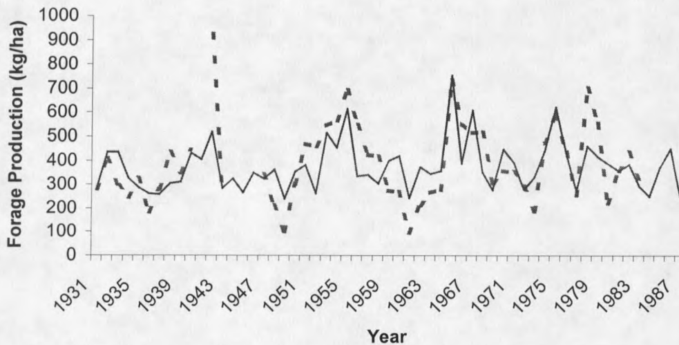
Figure 8. Plot of the residuals for Lethbridge, Alberta. The actual forage production (dashed line) vs predicted forage production (solid line) forage production data.
