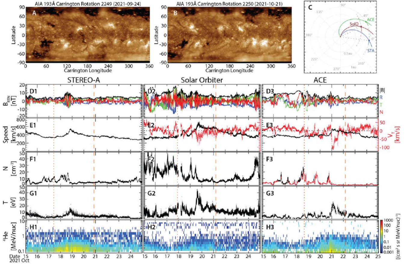
Figure 1. Example of an SIR observed by STEREO-A, Solar Orbiter, and ACE. (A)–(B) SDO/AIA synoptic maps for the two Carrington rotations that correspond to the time period of 2021 October 15–25. (C) Spacecraft locations in the Solar Ecliptic coordinate system with STEREO-A, Solar Orbiter, and ACE in blue, red, and green, respectively. Dashed curves indicate the orbit of the spacecraft for the full duration of the two Carrington rotations in (A) and (B), with the solid curves denoting the spacecraft orbit during the 10 day period shown in rows (D)–(H). For reference, the circles illustrate the spacecraft location on 2021 October 25, with dashed radial lines and Parker Spirals calculated using observed solar wind speeds at each spacecraft. (D1)–(D3) Magnetic field observations in RTN coordinates, (E1)–(E3) solar wind speed (in black) with the tangential solar wind flow, where measured (in red), (F1)–(F3) solar wind density, (G1)–(G3) solar wind temperature, (H1)–(H3) 4 He spectrograms. Note that panel (F3) shows both the high-quality data (in black) and the low-latency data (in red) from ACE SWEPAM to provide context to the more sparse high-quality solar wind density data. The dotted (dashed) lines in each column denote the start (stop) time of the suprathermal ion enhancements for that spacecraft.
