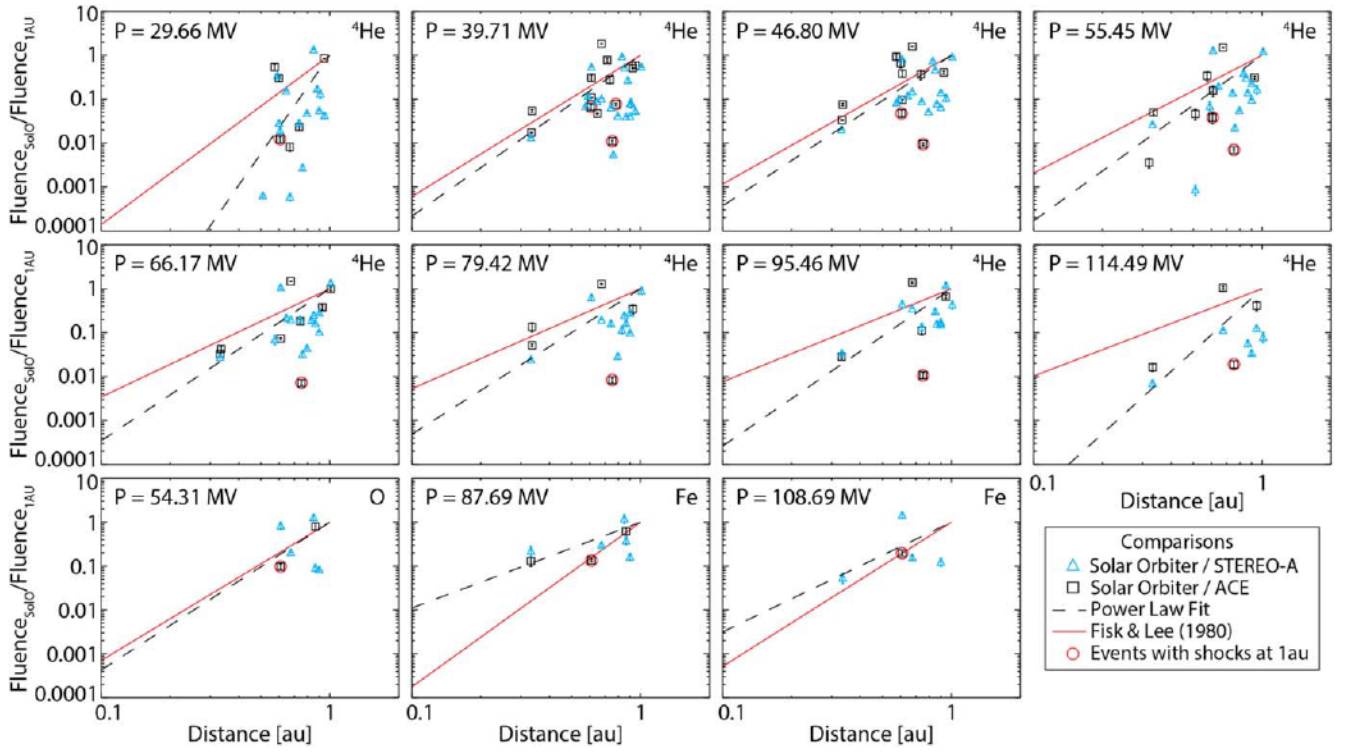
Figure 3. Normalized fluence decrease ( J_{\text{obs}}/J_{1\text{ au}} ) as a function of Solar Orbiter radial distance for different bins of rigidity for ^4\text{He} (top and middle rows), O, and Fe (bottom row). Comparisons between Solar Orbiter and ACE are shown as black squares, while those between Solar Orbiter and STEREO-A are shown as blue triangles. Events with an observed shock at 1 au are circled in red. Power-law fits are shown with the dashed black line for each rigidity bin, and the expected slope from L. A. Fisk & M. A. Lee (1980), assuming a shock beyond 1 au, is shown in red.
