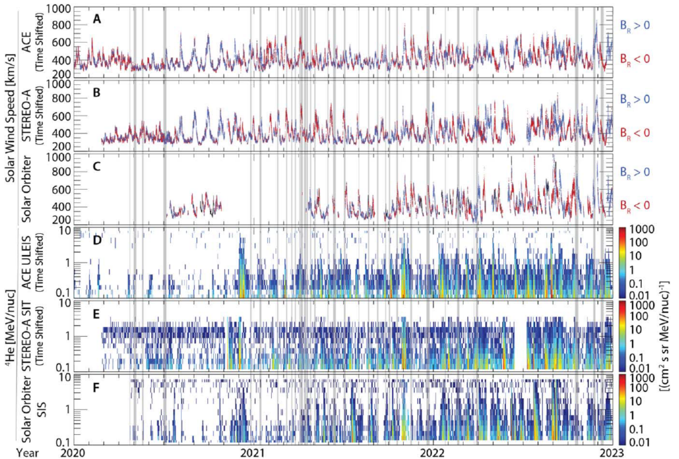
Figure 2. Three years of observations from ACE, STEREO-A, and Solar Orbiter, averaged down to 30 minute resolution, showing ((A)–(C)) solar wind speed colored by magnetic polarity (blue is positive B_R , red is negative B_R , and black indicates time without public magnetic field data at time of publication), and ((D)–(F)) 1 hr averaged suprathermal ^4\text{He} flux. Data resolution was reduced solely for the purpose of displaying three years of observations. Gray vertical bars denote the 33 intervals of SIR-associated suprathermal ion flux increases at Solar Orbiter that corresponded to suprathermal flux increases at ACE and STEREO-A, meeting all criteria defined in the text. Note, the apparent gap in STEREO-A observation from mid-June through early 2022 July is an artifact from time-shifting.
