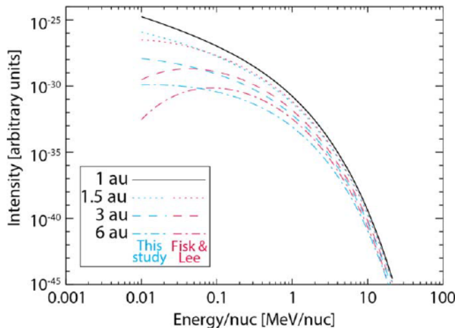
Figure 5. Comparison of the spectral modulation from L. A. Fisk & M. A. Lee (1980) (in red) with the empirically derived spectra in this study (in blue) for shocks at various radial distances when viewed from 1 au.
