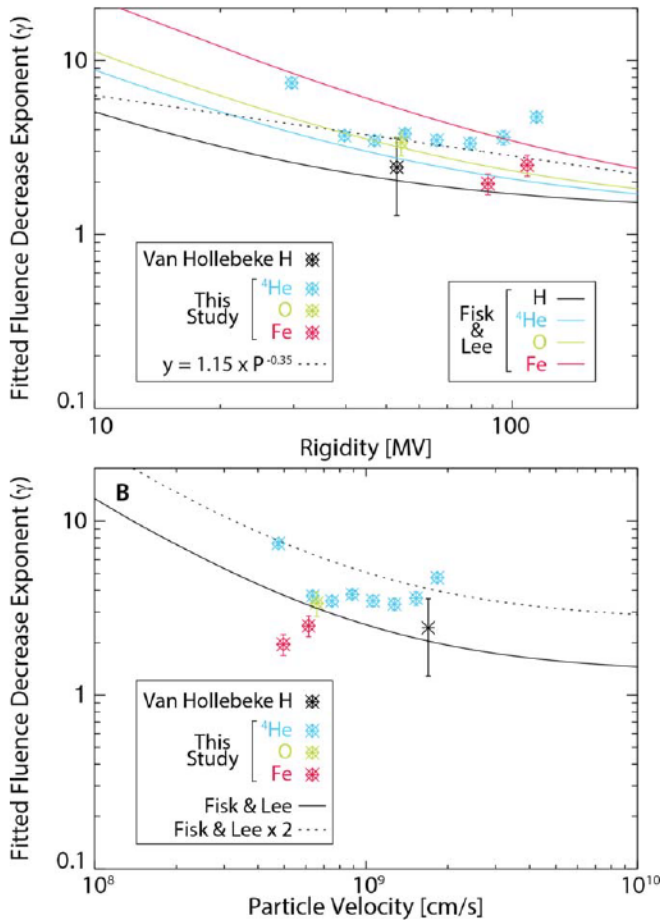
Figure 4. (A) Power-law exponents of normalized fluence vs. radial separation from the fits in Figure 3 as a function of rigidity (blue, green, and red points for ^4\text{He} , O, and Fe, respectively), including the power-law exponent of normalized peak proton intensity vs. radial separation from observations in M. A. I. Van Hollebeke et al. (1978) at less than 1 au (black point). The dashed line is the power-law fit through all data points shown. The solid curves are the expected values derived from the L. A. Fisk & M. A. Lee (1980) formulation for each species noted. (B) Same as in panel (A), but as a function of particle velocity. The solid black curve shows the expected values of power-law exponents as a function of particle velocity from L. A. Fisk & M. A. Lee (1980), which does not include species-dependent terms.
