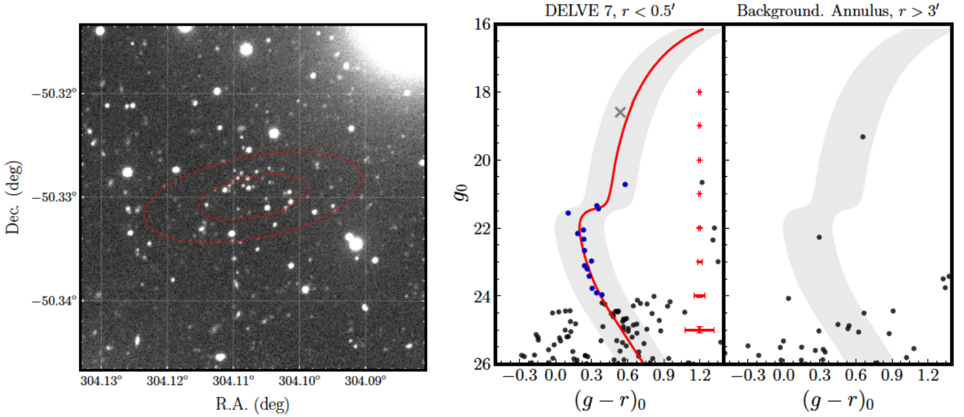
Figure 3. Follow-up imaging of DELVE 7 performed with Magellan/IMACS. Left panel: 2' \times 2' g -band cutout image centered on DELVE 7, which can be seen as a clear overdensity of faint pointlike sources. We overlay red ellipses demarcating r_h and 2r_h . Right panel: color-magnitude diagrams for pointlike sources in the vicinity of DELVE 7. The left panel shows a circular region with r < 0.5' , while the right panel shows an equal-area background annulus with inner radius r = 3' . Stars used for the isochrone fit are shown in blue; the best-fit isochrone (shown in red) was found to be \tau = 10 Gyr, Z = 0.00061 , (m - M)_0 = 18.1 . The median Magellan photometric uncertainties for stars around DELVE 7, as a function of g -band magnitude, are indicated by red error bars. Although one bright candidate RGB member falls close to the isochrone, this star has a Gaia parallax of \varpi = 0.71 \pm 0.15 mas that places it well in the foreground of DELVE 7; we mark it here with an “x” to emphasize its nonmembership. The shaded regions show \pm 0.2 in color about the best-fit isochrone.
