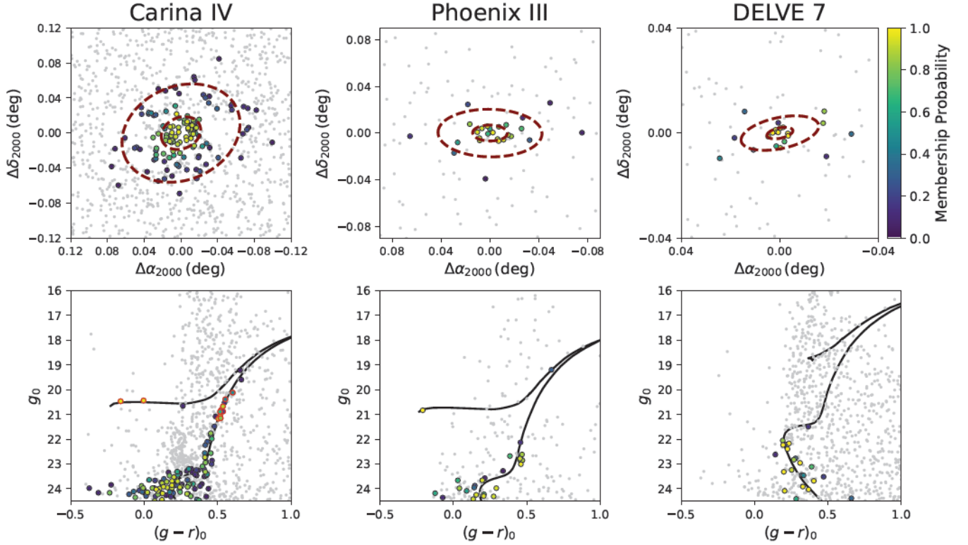
Figure 2. The spatial distributions (top panels) and color–magnitude diagrams (bottom panels) for likely member stars in Carina IV (left panels), Phoenix III (center panels), and DELVE 7 (right panels). Stars are colored by their membership probabilities derived as part of our ugali characterization analysis, which incorporates the spatial, photometric, and color information of each star. Stars with a lower ugali membership probability ( p_{\text{ugali}} < 0.05 ) are shown in gray. The top panels also show ellipses representing the ugali best-fit half-light radius, r_h , and 3 times this half-light radius, 3r_h , for each system. For Carina IV, we highlight with red outlines the stars in the color–magnitude diagram that have both a high ugali membership probability ( p_{\text{ugali}} > 0.20 ) and a Gaia detection. These stars are discussed further in Section 5.1 and Appendix A. Carina IV is the best-populated of the three systems, featuring a clear main-sequence turn-off (MSTO), red giant branch (RGB), and blue horizontal branch (BHB). Phoenix III is at a similar distance, but it is fainter with only a handful of likely member stars. DELVE 7 is substantially fainter, featuring no highly probable RGB members and is potentially only composed of main-sequence stars. This lack of RGB stars is consistent with other faint Milky Way satellites at M_V > 0 (e.g., DELVE 5, Kim 3, and Ursa Major III/UNIONS 1).
