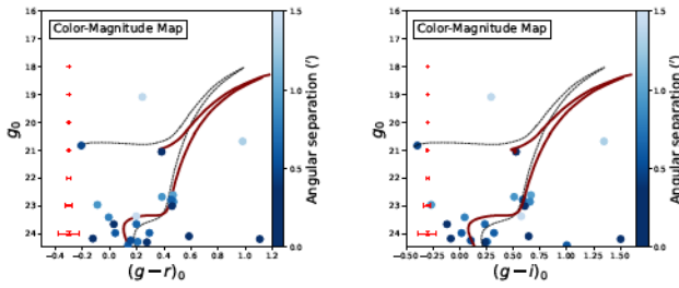
Figure 7. Color-magnitude diagrams for both g-r (left panel) and g-i (right panel) band pairs for stars within 1.5 of Phoenix III. Stars are colored by separation from each system's centroid, with darker colors representing smaller separations. We overlay PARSEC isochrones corresponding to the intermediate-age 7 Gyr solution (solid maroon lines) and the old 12 Gyr solution (black dotted lines) for comparison. The median photometric uncertainties for stars around Phoenix III, as a function of g -band magnitude, are indicated by red error bars.
