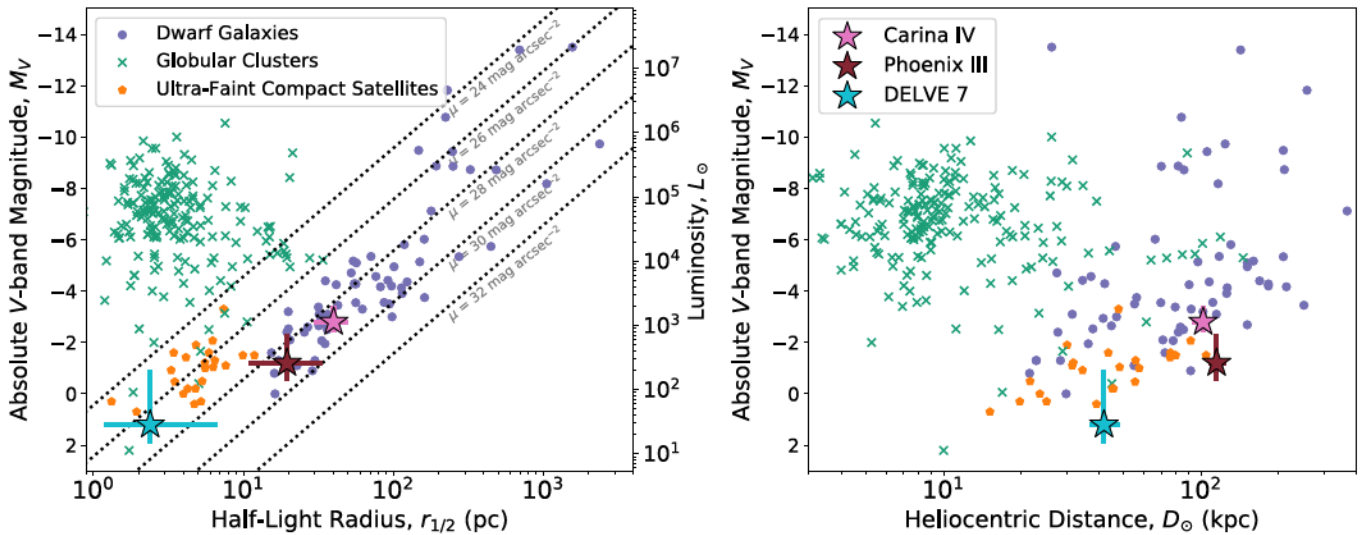
Figure 6. Left panel: absolute V-band magnitude ( M_V ) vs. azimuthally averaged physical half-light radius ( r_{1/2} ) for the three new Milky Way satellites and the population of known Local Group globular clusters and dwarf galaxies. Right panel: the same diagram, but showing M_V vs. heliocentric distance ( D_{\odot} ). Spectroscopically confirmed dwarf galaxies and likely galaxy candidates are shown in purple circles, while Milky Way globular clusters are shown with green “x” symbols. Ambiguous ultra-faint compact satellites are shown with orange pentagon symbols. The three systems discovered in this work are shown as colored stars with bars representing 68% posterior uncertainty intervals. Data on the Milky Way satellite population were compiled by A. B. Pace (2025), and we adopt the same classifications as C. Y. Tan et al. (2025a).
