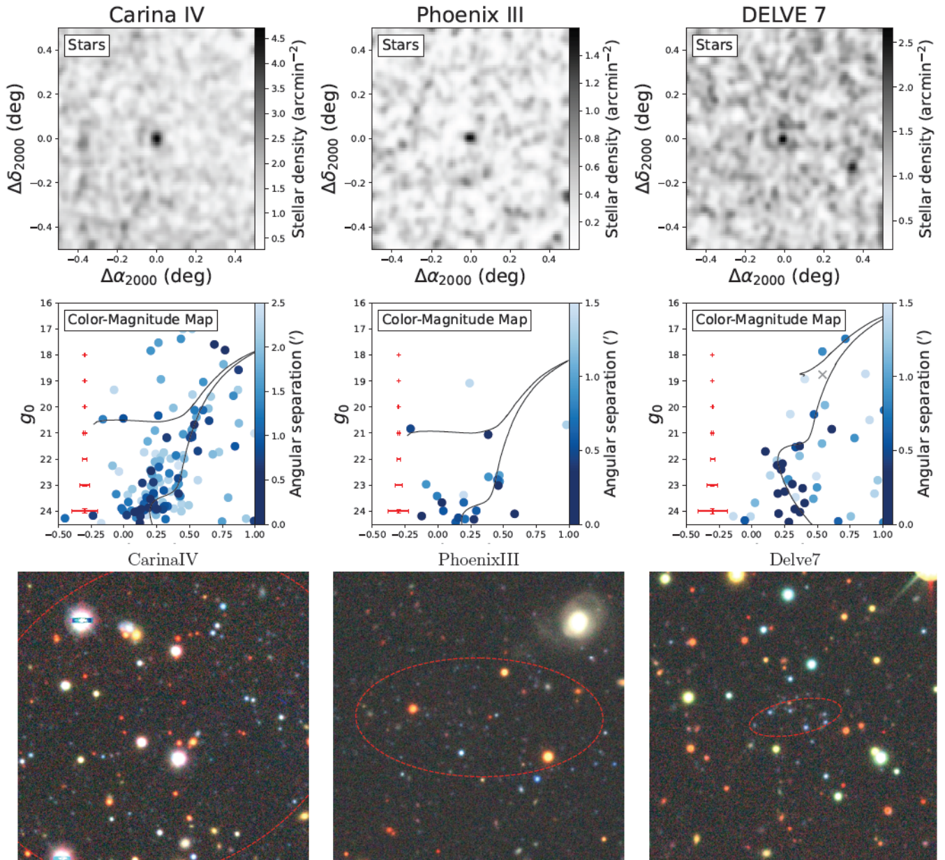
Figure 1. Diagnostic plots for each of the three newly discovered satellites, closely matching those used to identify the systems in our search. Top panels: isochrone-filtered stellar density maps for a 1^\circ \times 1^\circ region centered on each candidate, smoothed with a 0.5 Gaussian kernel. Middle panels: color-magnitude diagrams for stars within 2/5 of Carina IV and 1/5 of Phoenix III and DELVE 7, centered on each candidate system. Stars are colored by separation from each system’s centroid, with darker colors representing smaller separations. Also overlaid is the best-fit old, metal-poor PARSEC isochrone, with parameters taken from the best-fit ugal results in Table 1. The median photometric uncertainties for stars around each satellite, as a function of g -band magnitude, are indicated by red error bars. The “x” marker indicates a confirmed nonmember star of DELVE 7 with a Gaia parallax of \varpi = 0.71 - 0.15 mas, clearly placing it in the foreground of the system. Bottom panels: false-color coadded images ( \sim 2' \times 2' , 0.03 \times 0.03 ) of Carina IV, Phoenix III, and DELVE 7 from the Legacy Surveys Sky Viewer DR10. Each cutout has been artificially brightened by a factor of 1.8 to highlight faint sources. We also overlay red ellipses on the coadded images demarcating the half-light radius, r_h , of the satellites.
