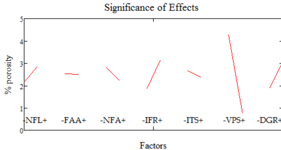
Figure 57: ANOVA plot of the significance of the different process parameters with respect to porosity.
