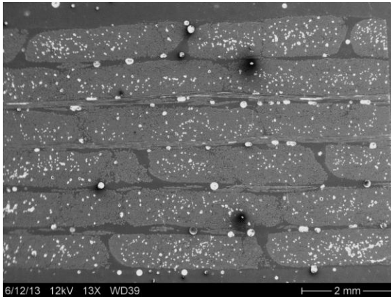
Figure 68: Micrograph of a laminate infused with a high flow rate.
