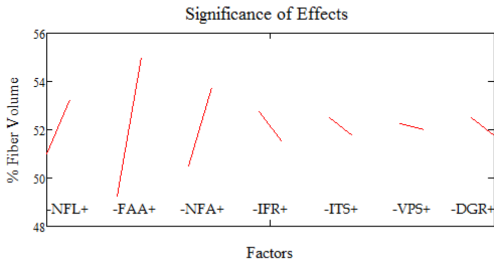
Figure 61: ANOVA plot of the significance of the different process parameters with respect to fiber volume fraction.
