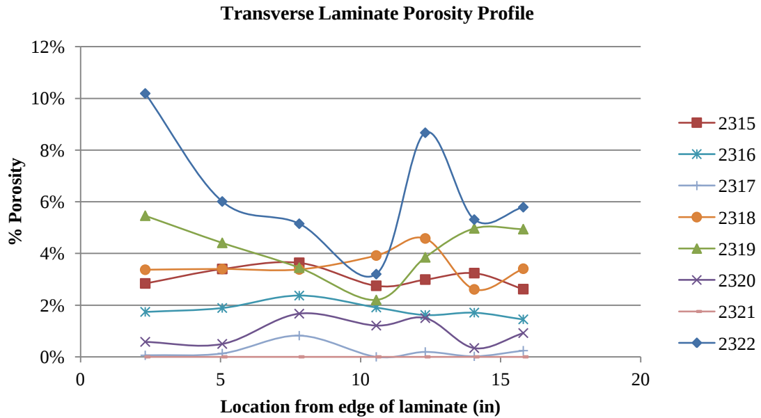
Figure 49: Representation of porosity across the width of the laminate.
