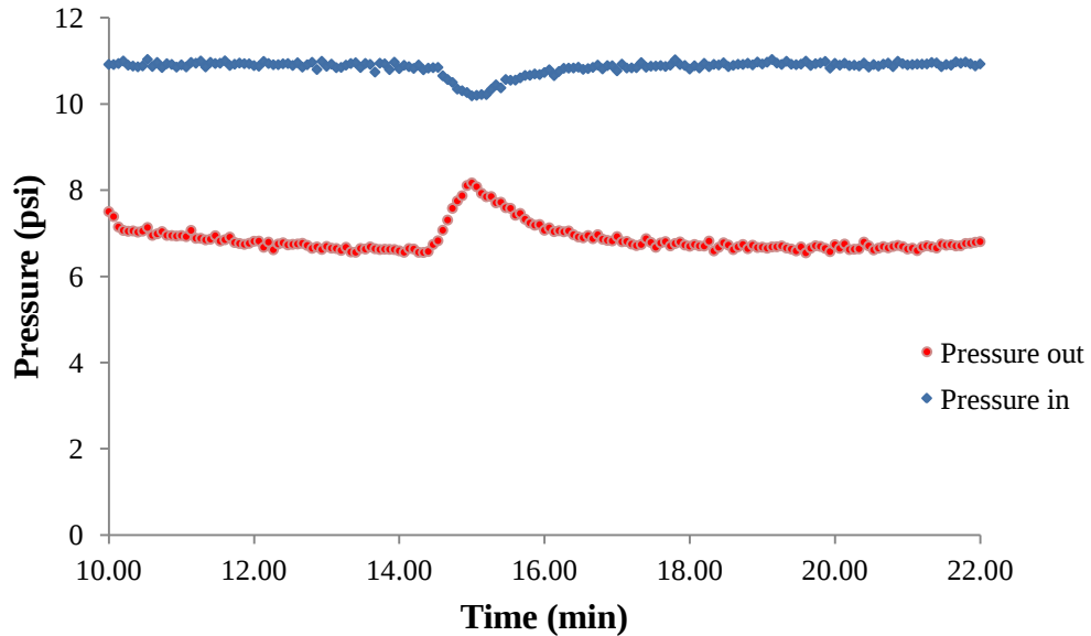
Figure 72: Spike in mold pressure for plate 2318.
