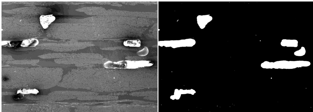
Figure 43: The left micrograph was created using the SEM; the right image is the binarized image.
