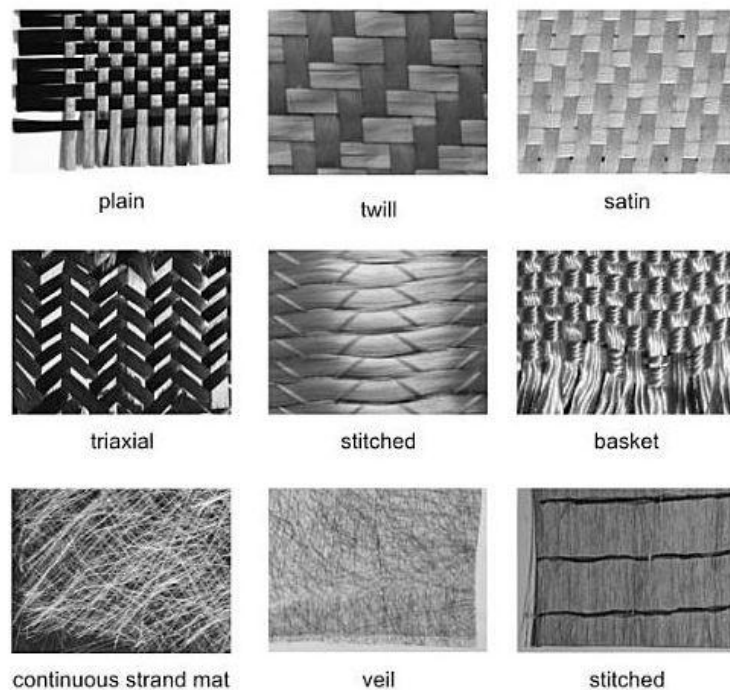
Figure 3: Fabric architecture [23].
