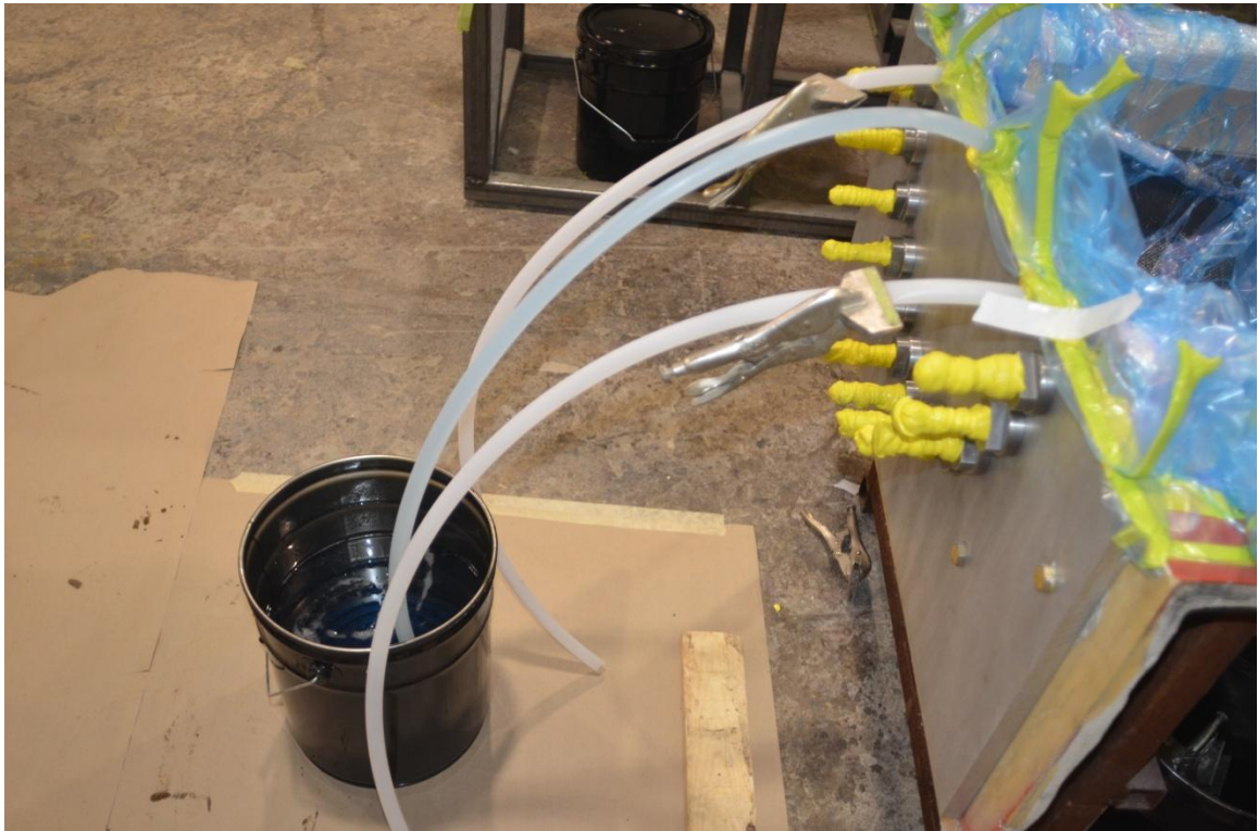
Figure 11: Resin is mixed in large pails, and then transferred to 5-gallon buckets during the injection process. Modified, vise-grip clamps are used to control the flow of resin and to seal the vacuum and injection tubes when not in use.
