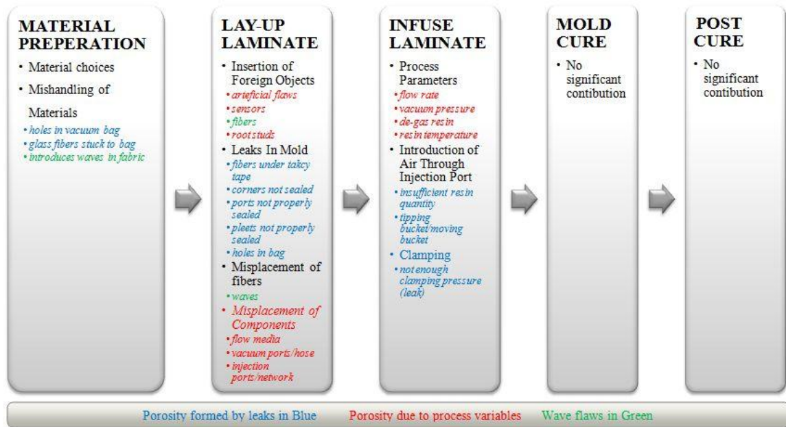
Figure 65: Laminate work flow and flow introduction model.
