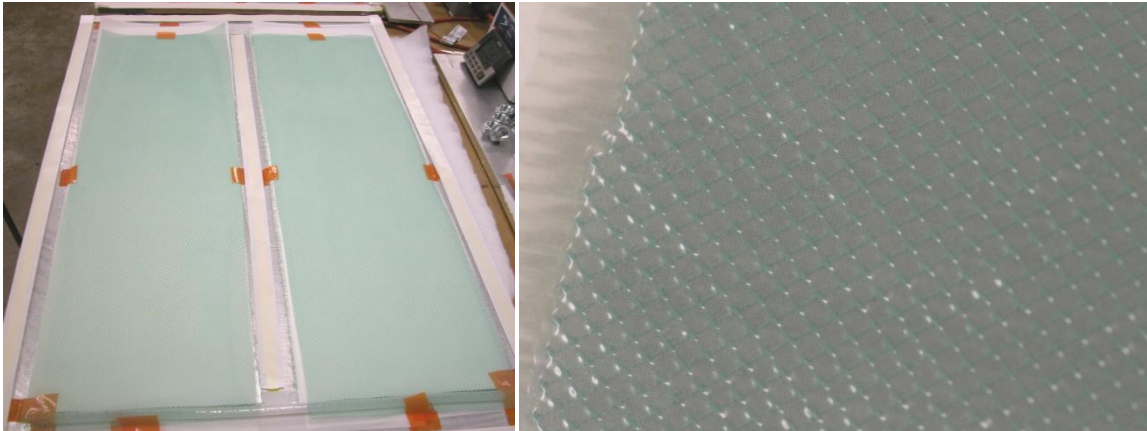
Figure 20: Left is flow media being used in the construction of a glass laminate. Right is a close up view of resin flowing through the open mesh of the flow media.
