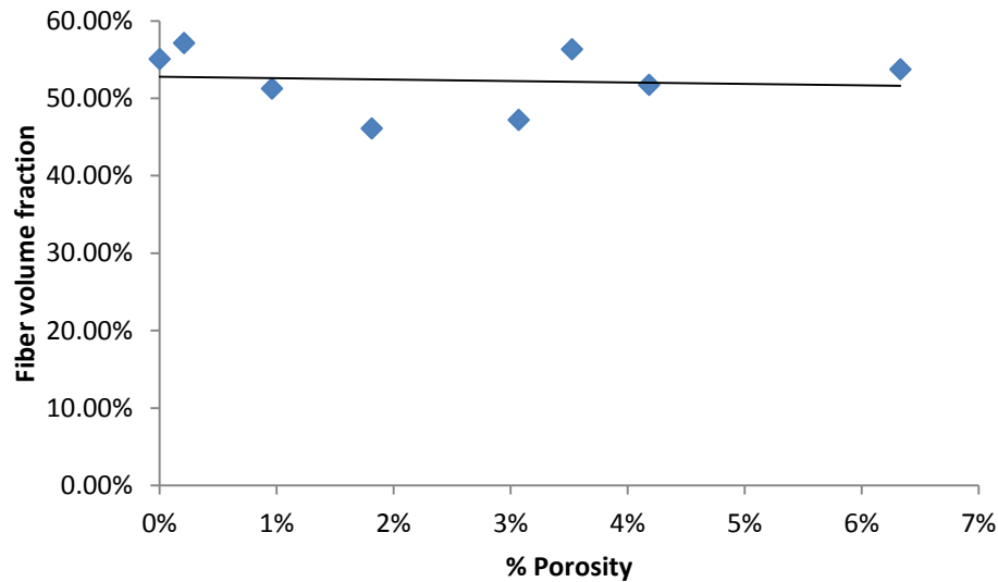
Figure 50: Fiber volume as a function of porosity.
