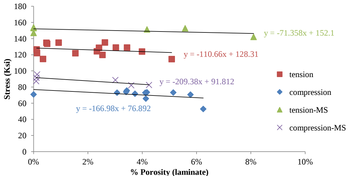
Figure 55: Ultimate strength comparison with porosity content for uni-directional laminates. Strength values were compared with samples manufactured for J. Nelson and T. Riddle.
