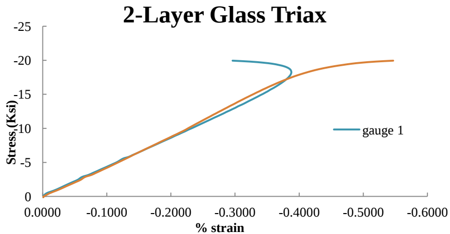
Figure 54: Compression test of 2-layer triax which shows buckling effects.
