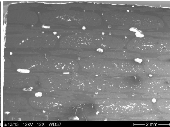
Figure 69: Micrograph of a laminate infused with a low flow rate.
