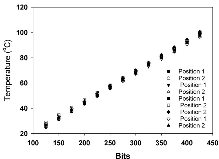
Figure SI1: Calibration of the temperature control system thermocouples. Thermocouples attached to an external thermometer (both type T and K) were placed next to the thermocouples attached to the device. The number of bits read by the MAX6675 was correlated to the temperature measured by the external thermocouple/thermometers to determine the number of bits per °C given by the MAX6675. Data shown for 9 different measurements at the two thermocouple positions.
