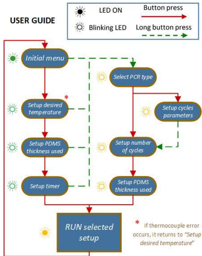
Figure SI2: The user guide demonstrating how to navigate through the menus programmed into the microcontroller.
