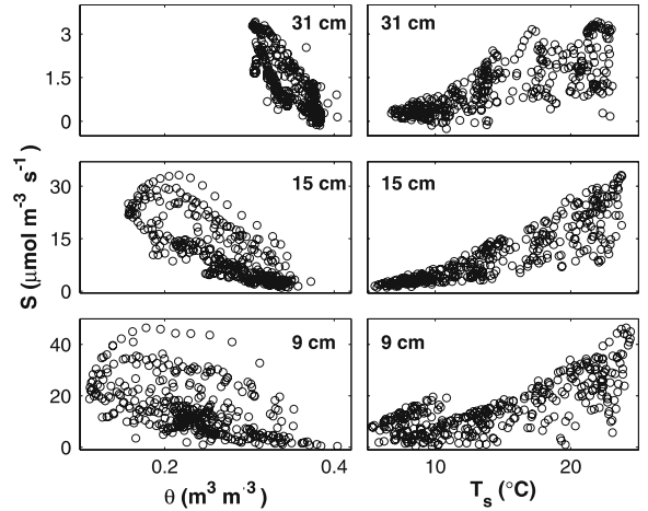
Fig. 8 Soil CO 2 production ( S ) as a function of local soil moisture ( \theta ) and local soil temperature ( T_s ) at three different depths in the plot AF1 (Table 1) during the year 2006
