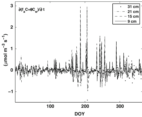
Fig. 6 Rate of change of daily CO 2 storage in both aqueous and gas phase at different soil depths in the plot AF1 during 2006
