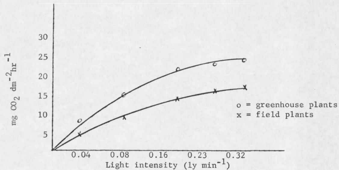
Figure 1. Average light saturation of photosynthesis in leaves of four sainfoin clones grown in the field and greenhouse.
