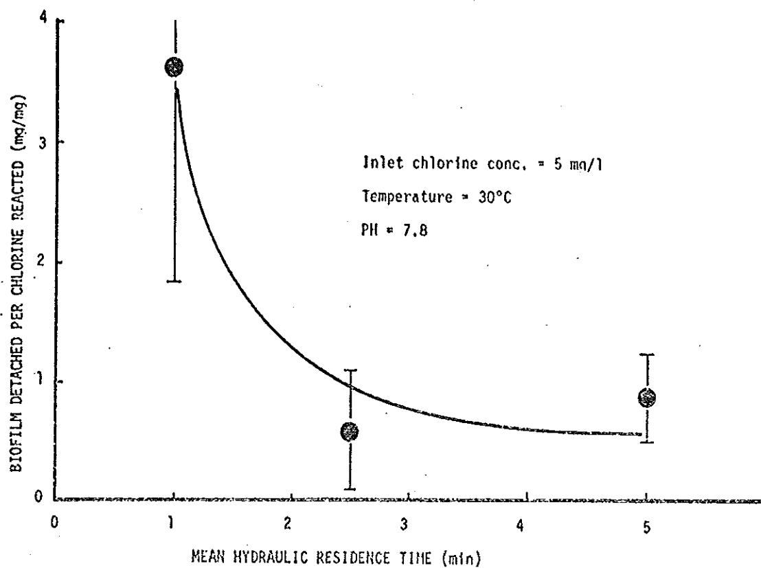
Figure 6a. Effect of reactor mean residence time on biofilm detached per chlorine reacted.
