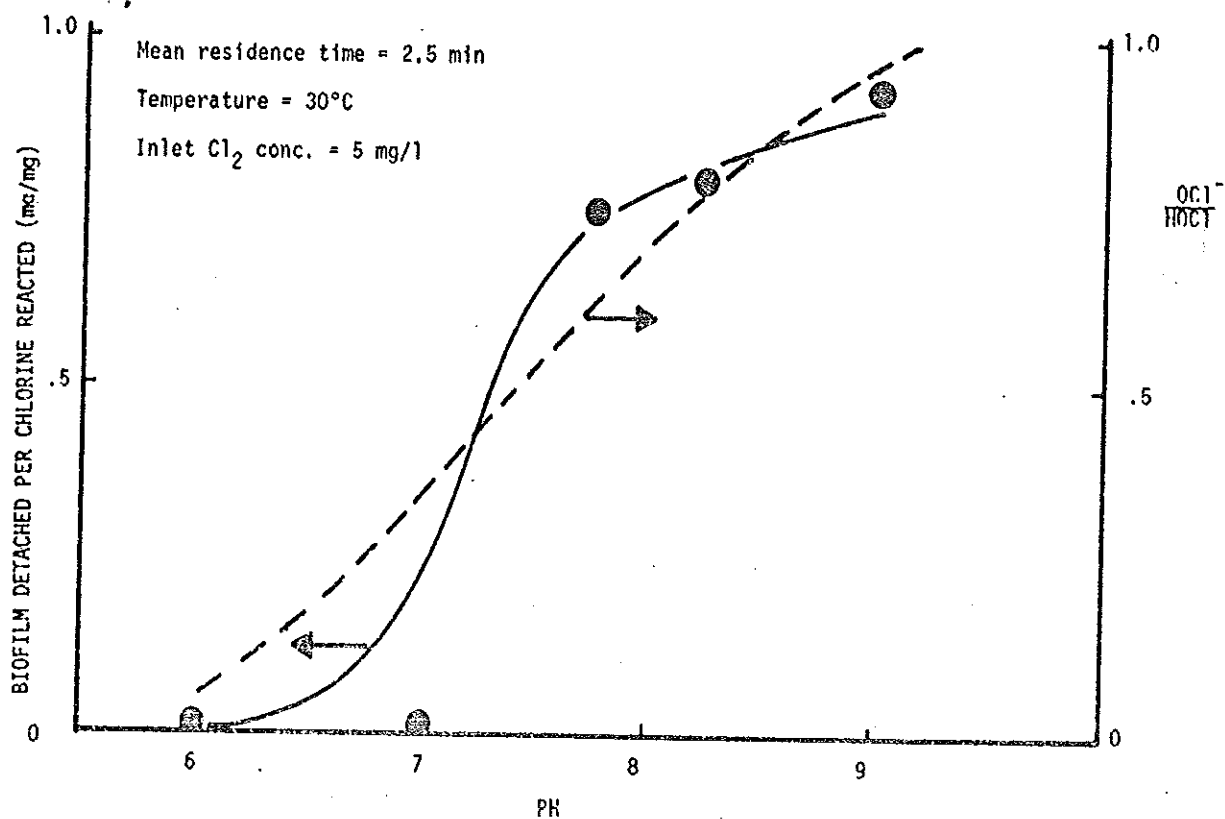
Figure 6c. The influence of PH on biofilm detached per chlorine reacted.
