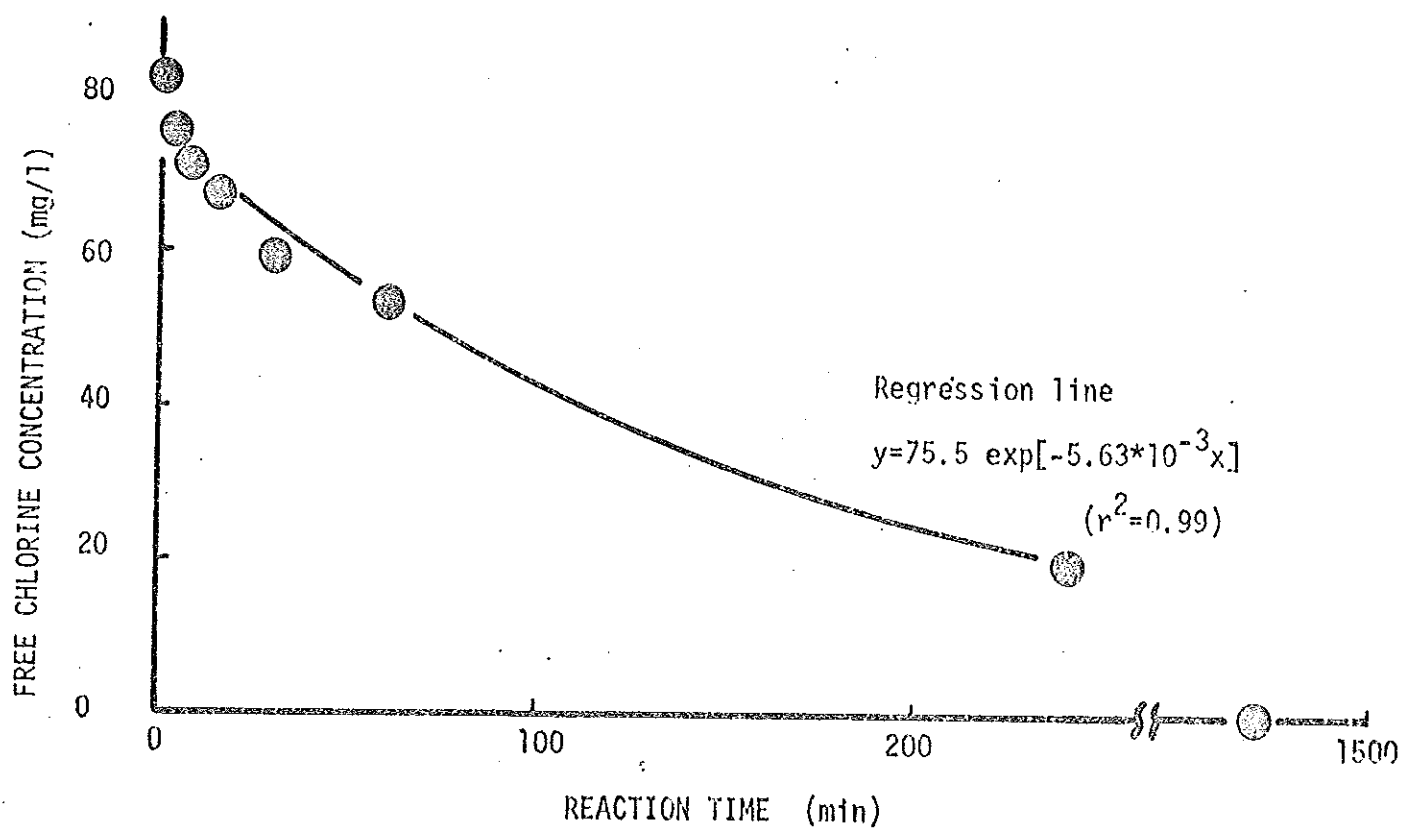
Figure 3. Decrease in chlorine concentration with time due to reaction with dispersed biofilm in a batch reactor at 37°C. Initial biomass conc. was 88.6 mg/l.
