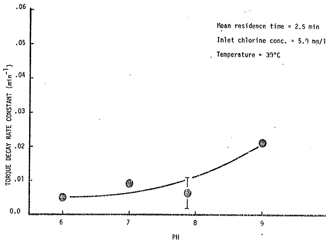
Figure 8b. The influence of PH on the torque decay rate constant.
