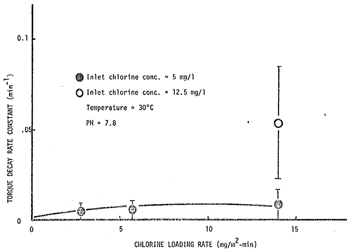
Figure 7c. The influence of chlorine loading rate on torque reduction.
