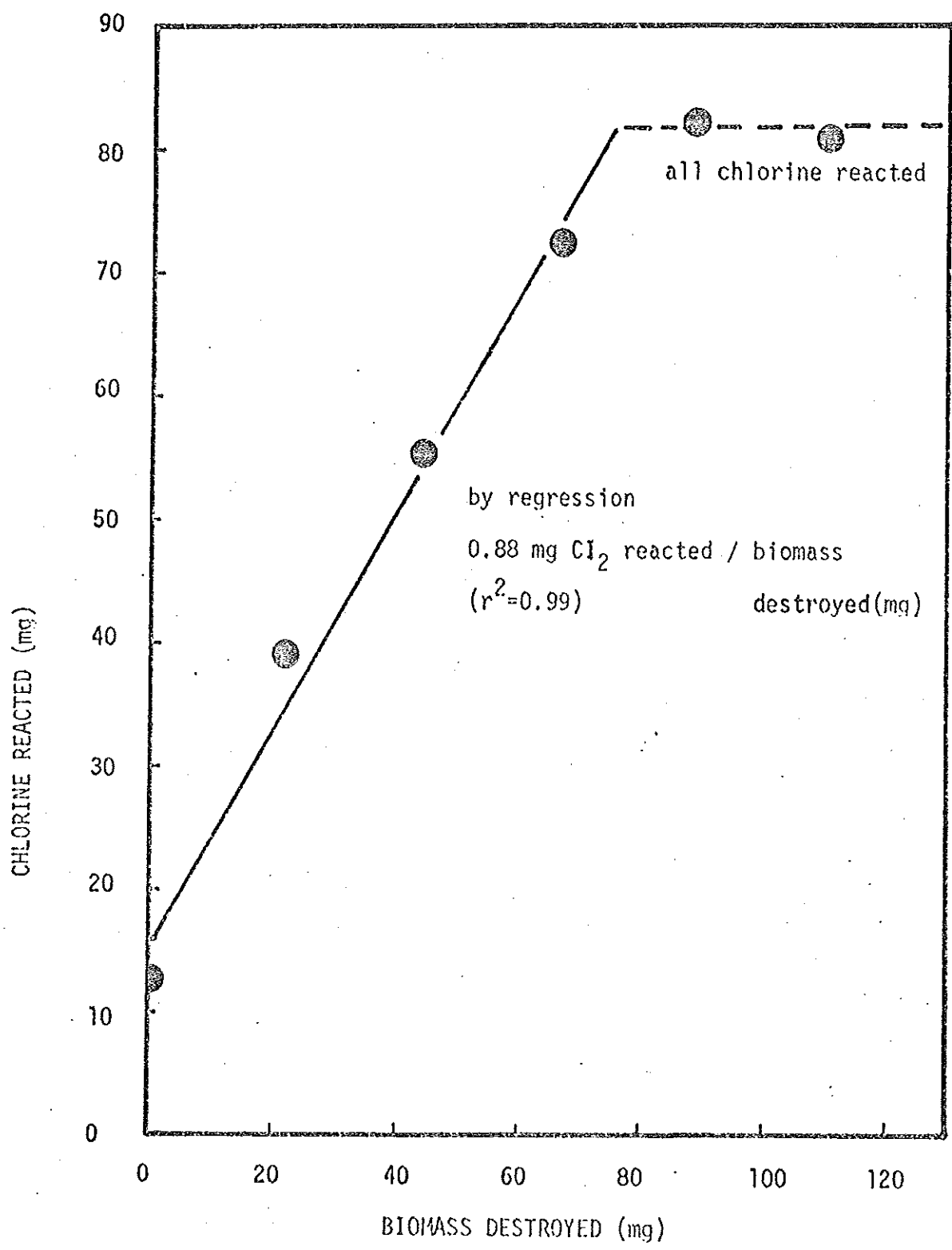
Figure 4. The relationship between chlorine reacted and dispersed biofilm destroyed in a batch reaction test.
