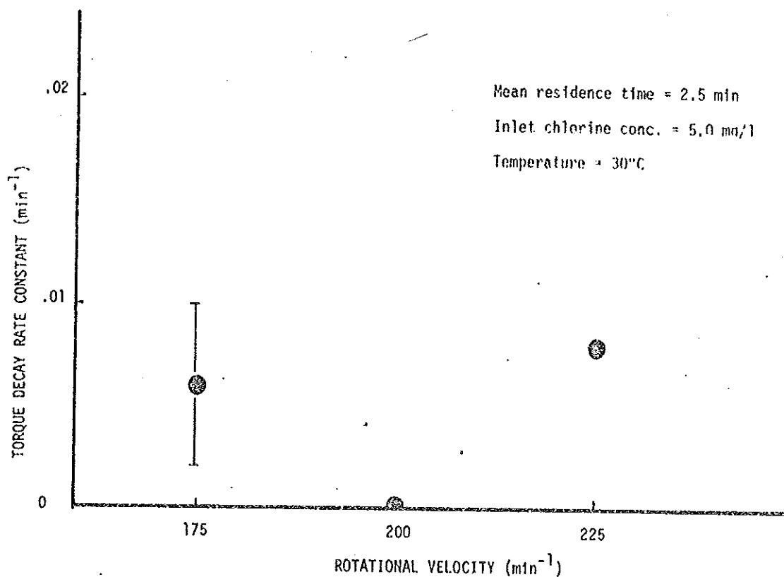
Figure 8c. The influence of rotational velocity on the torque decay rate constant.
