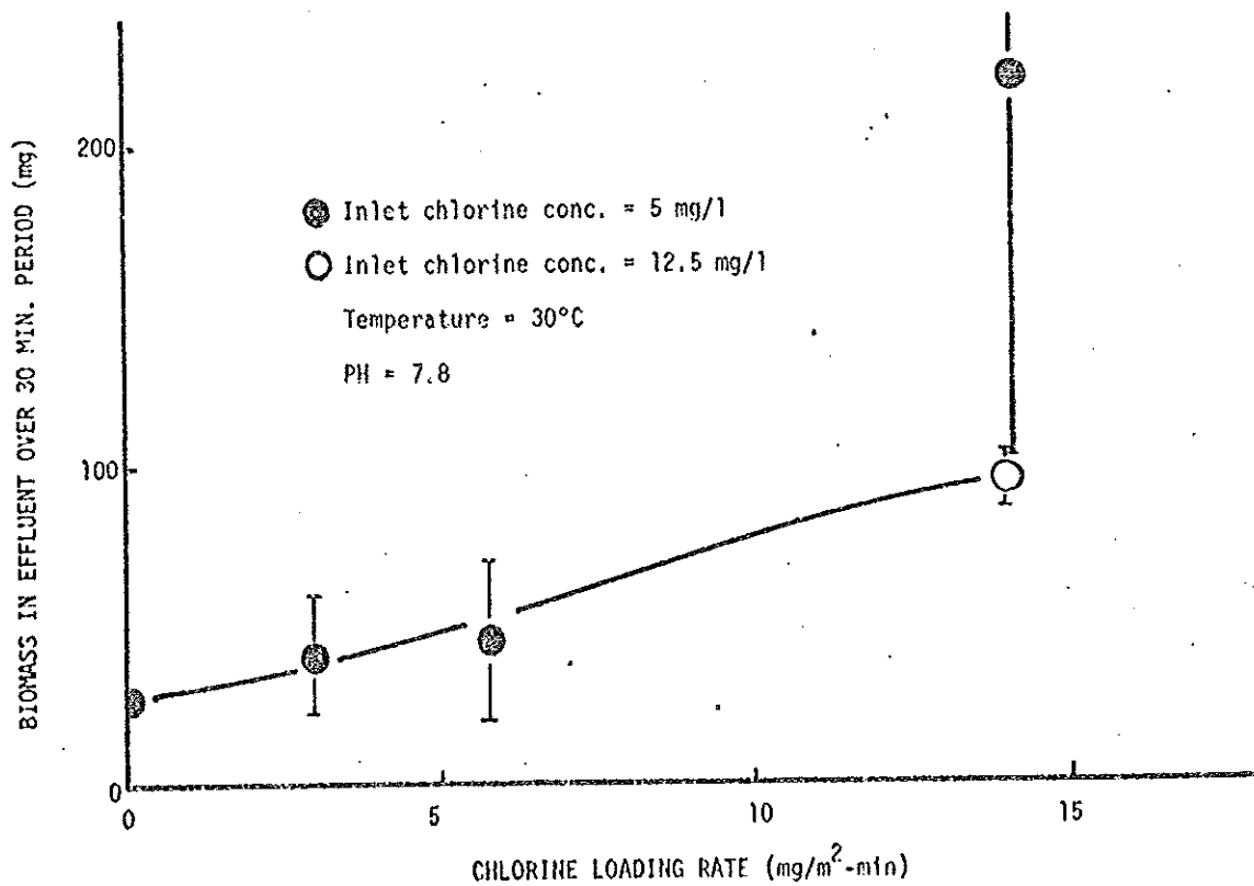
Figure 7b. The influence of chlorine loading rate on biomass exiting the reactor.
