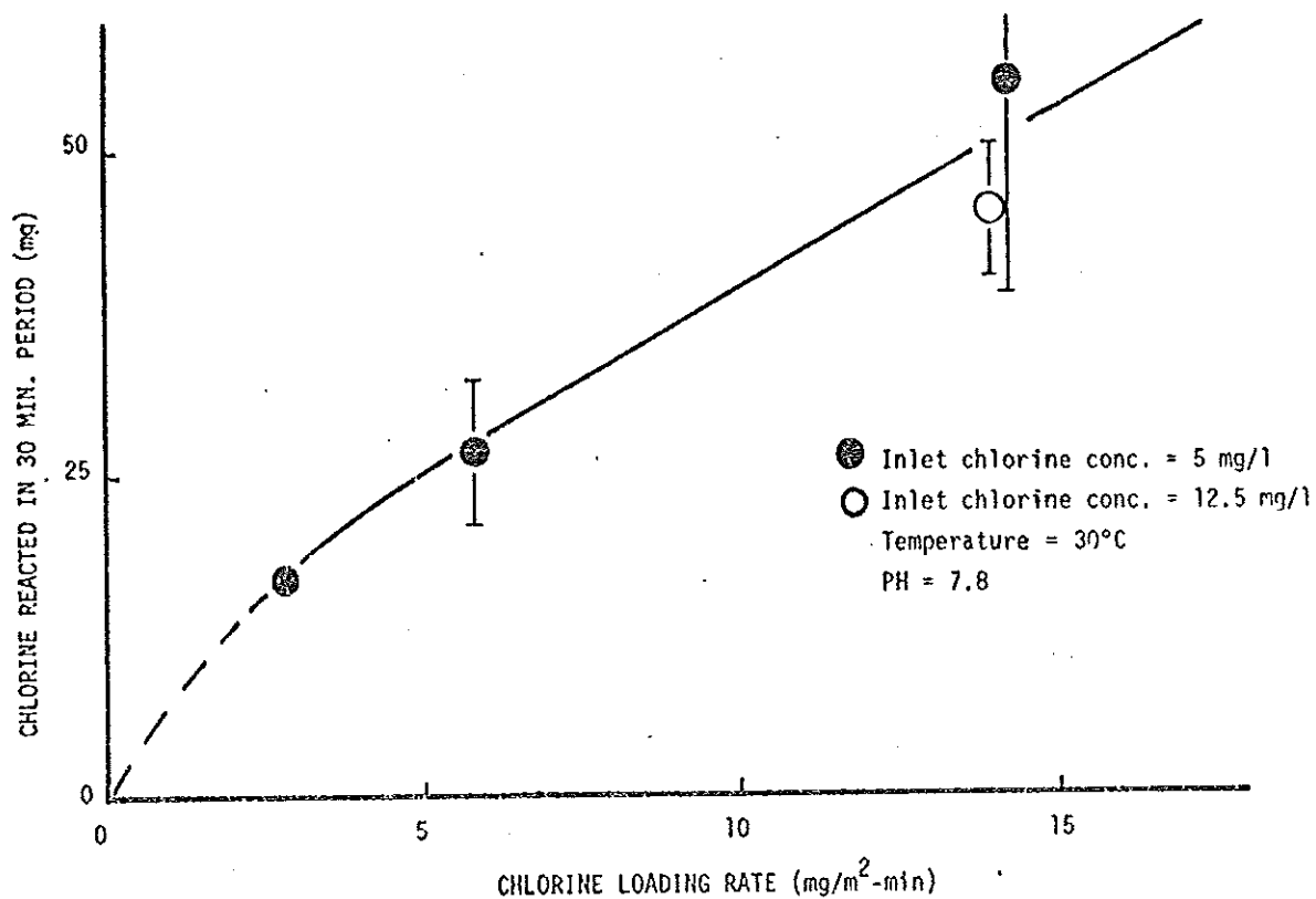
Figure 7a. The influence of chlorine loading rate on chlorine reacted in biofilm.
