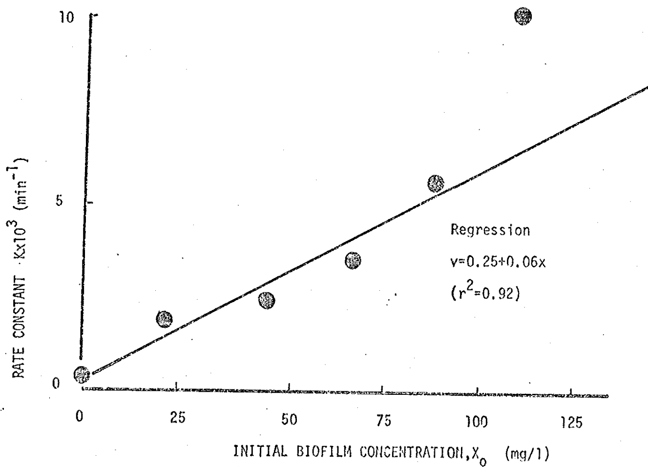
Figure 5. Influence of initial biomass concentration on rate constant, k .
