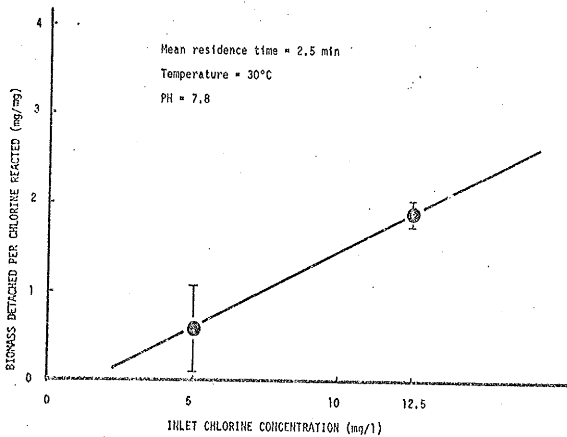
Figure 6b. The influence of inlet chlorine conc. on biofilm detached per chlorine reacted.
