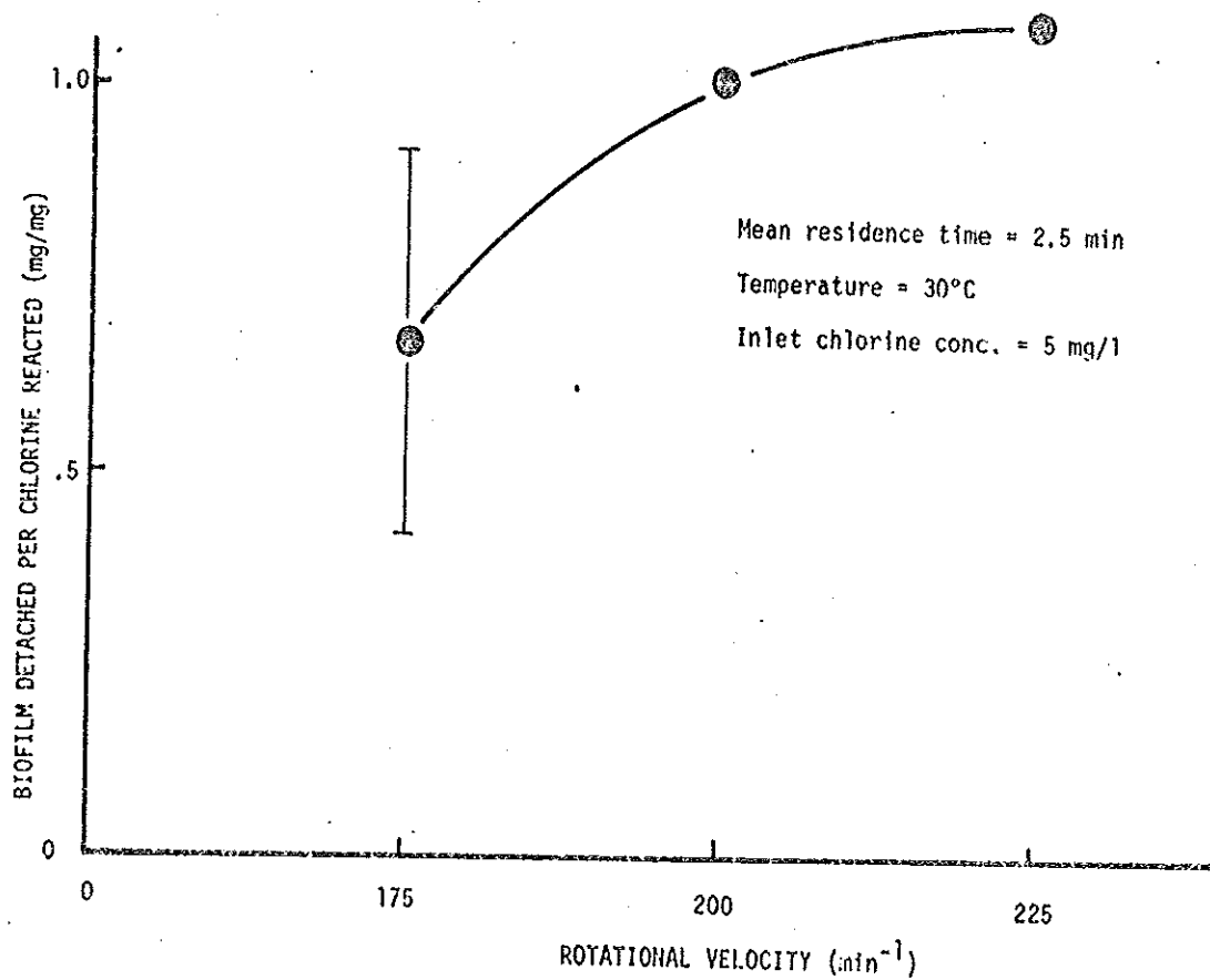
Figure 6d. The influence of rotational velocity on biofilm detachment per chlorine reacted.
