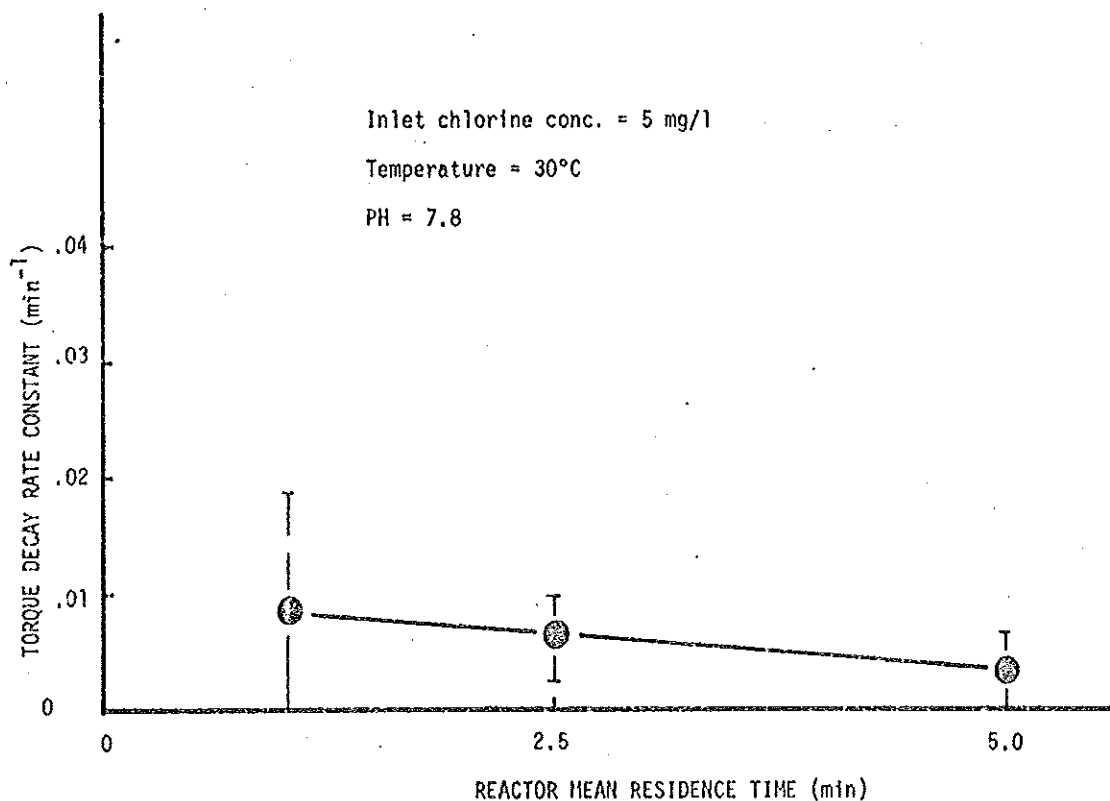
Figure 8a. The influence of reactor mean residence time at constant inlet chlorine concentration (i.e., surface chlorine loading rate) on the torque decay rate constant.
