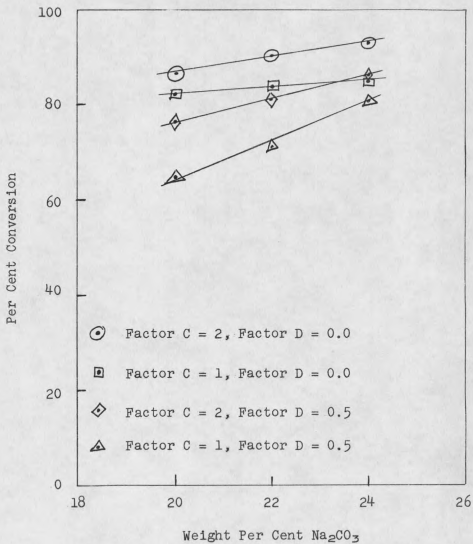
Figure 4. Plot of Per Cent Conversion vs. Weight Per Cent \text{Na}_2\text{CO}_3 for Samples Roasted at 2200°F.
