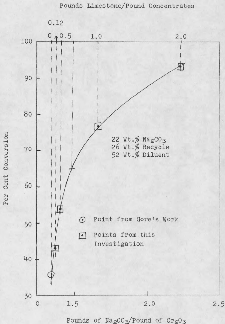
Figure 7. Plot of Per Cent Conversion vs. Weight Ratio of \text{Na}_2\text{CO}_3 for Mixtures in which Recycle is Replaced by Limestone.
