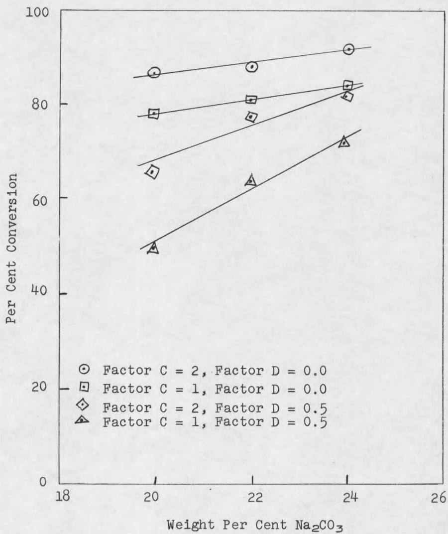
Figure 3. Plot of Per Cent Conversion vs. Weight Per Cent \text{Na}_2\text{CO}_3 for Samples Roasted at 1900°F.
