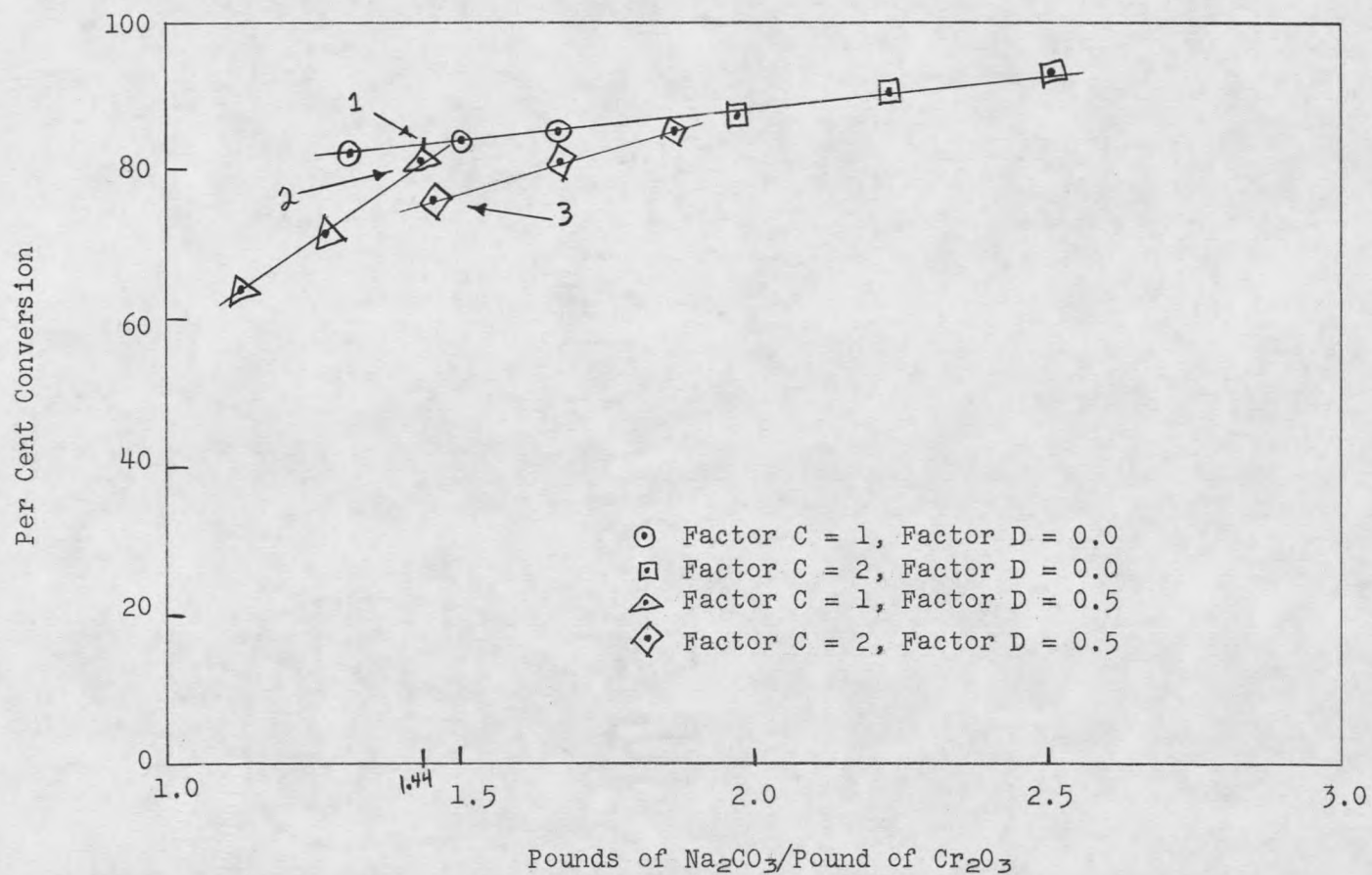
Figure 6. Plot of Per Cent Conversion vs. Weight Ratio of \text{Na}_2\text{CO}_3 to \text{Cr}_2\text{O}_3 for Mixtures Roasted at 2200^\circ\text{F} .
