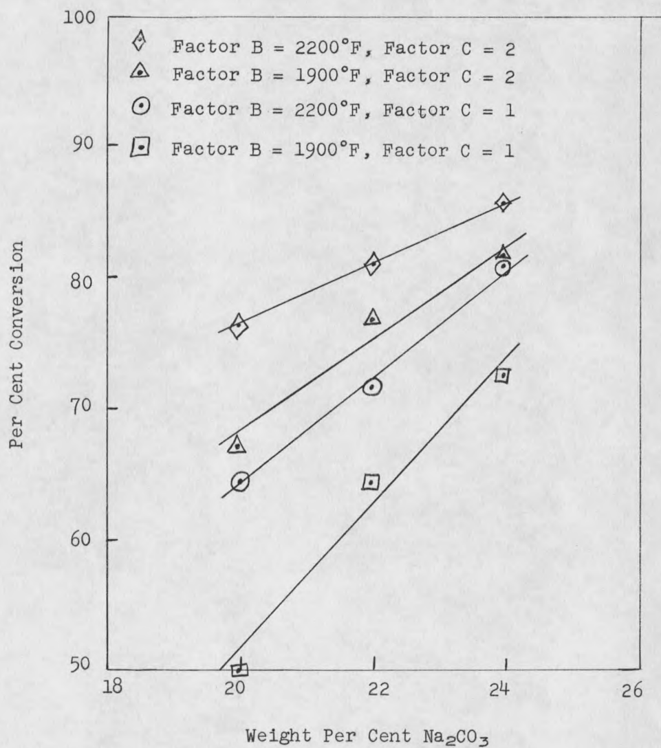
Figure 2. Plot of Per Cent Conversion vs. Weight Per Cent \text{Na}_2\text{CO}_3 for Mixtures Containing Recycle.
