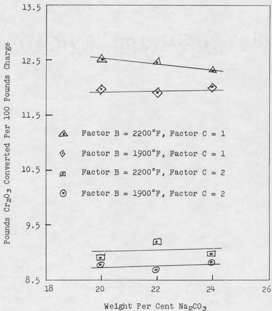
Figure 8. Plot of \text{Cr}_2\text{O}_3 Converted Per 100# Charge for Samples Not Containing Recycle.
