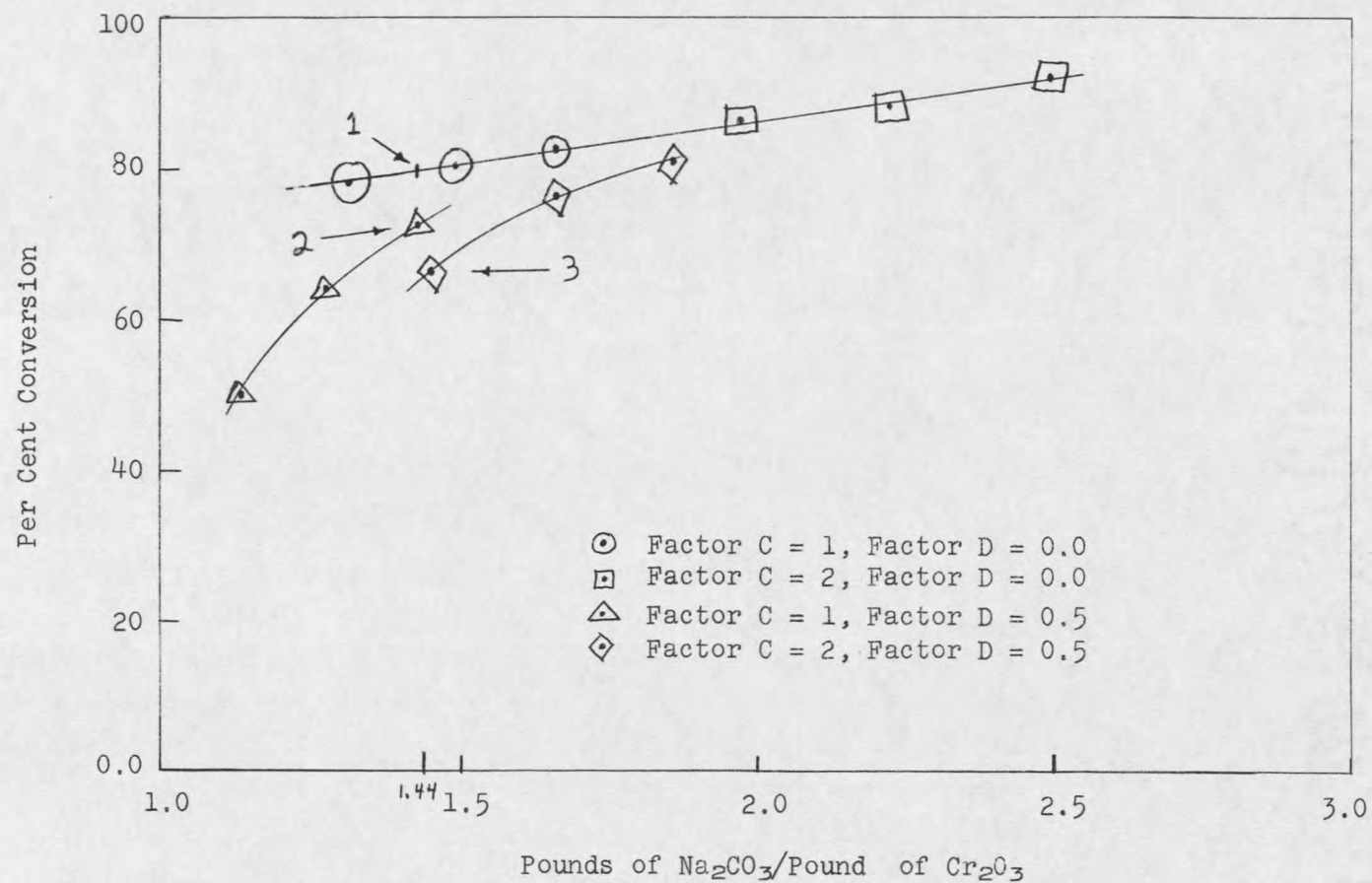
Figure 5. Plot of Per Cent Conversion vs. Weight Ratio of \text{Na}_2\text{CO}_3 to \text{Cr}_2\text{O}_3 for Mixtures Roasted at 1900^\circ\text{F} .
