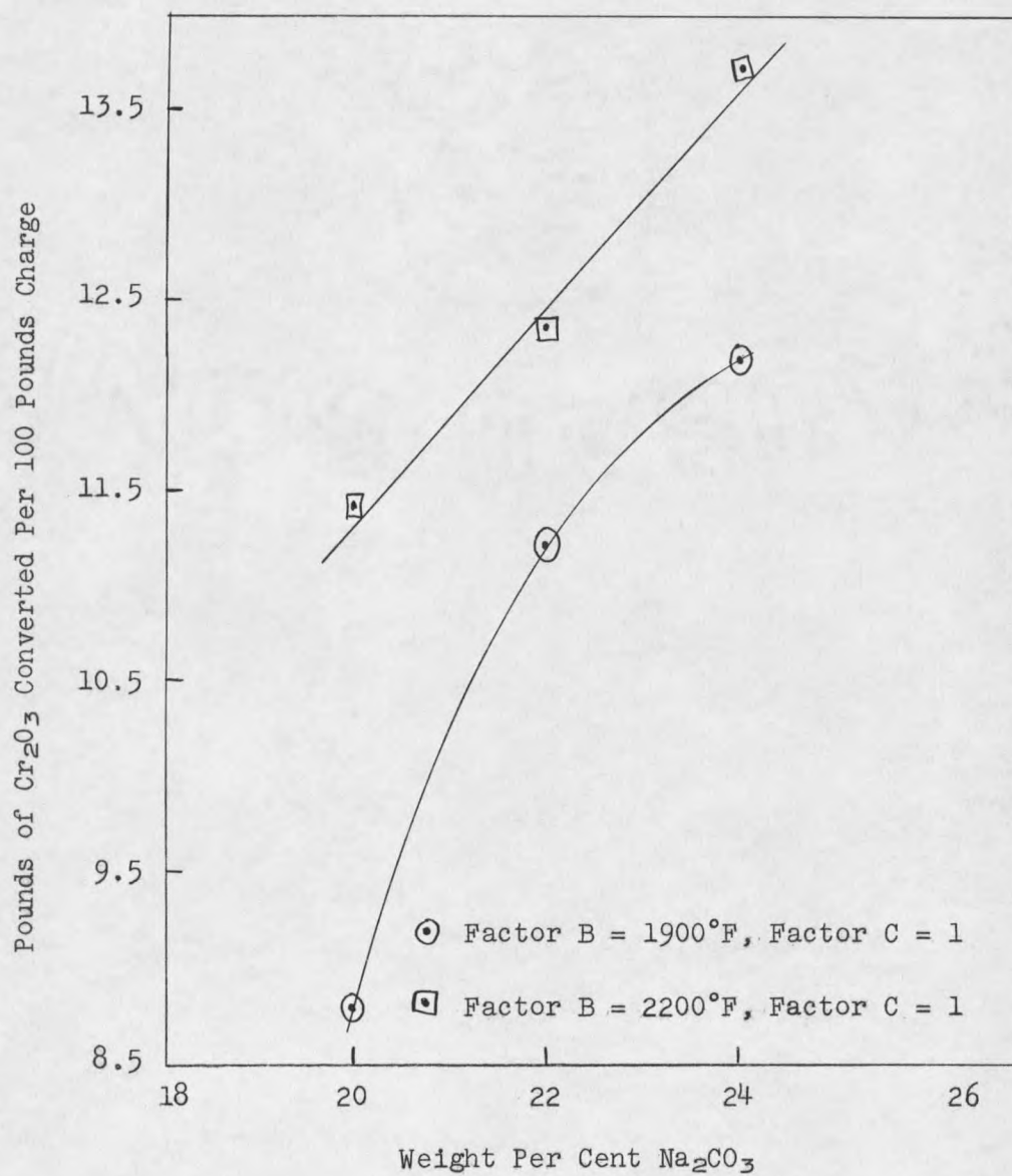
Figure 10. Plot of # \text{Cr}_2\text{O}_3 Converted Per 100# Charge for Samples Containing Recycle.
