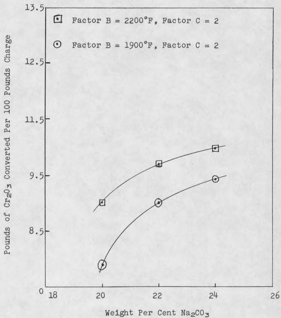
Figure 9. Plot of \text{Cr}_2\text{O}_3 Converted Per 100# Charge for Samples Containing Recycle.
