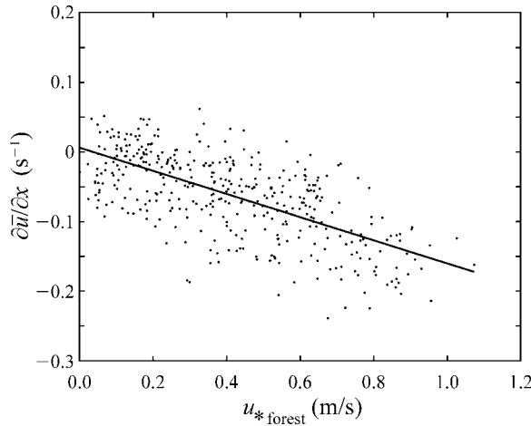
FIG. 9. The variation of \partial \bar{u} / \partial x at the forest edge with u_* above the pine forest canopy for northerly wind directions ( \text{WD} \in [0 \pm 45^\circ] ). Note that \partial \bar{u} / \partial x becomes increasingly negative with increasing u_* , consistent with the BFS analogy.
