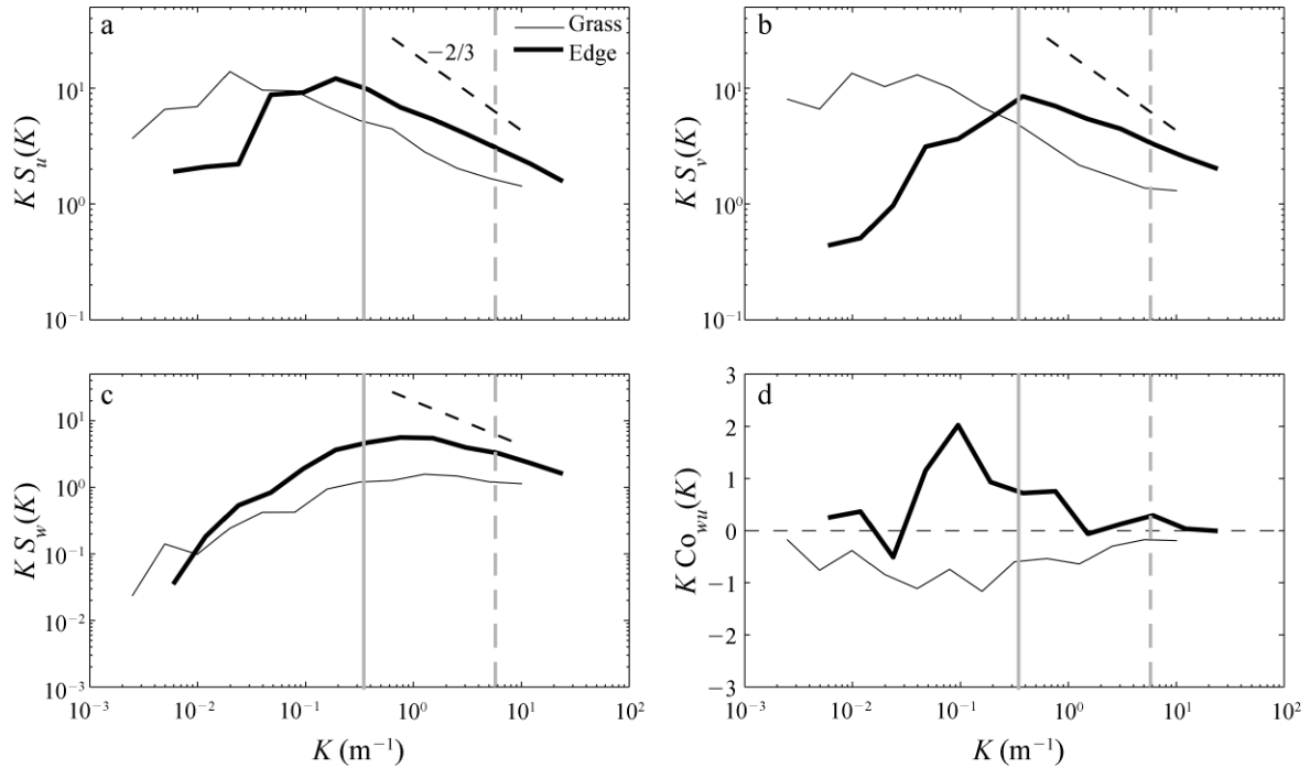
FIG. 13. The Haar wavelet energy spectra ( S ) at the edge and at the center of the grass clearing for (a) u'(S_u) , (b) v'(S_v) , and (c) w'(S_w) as a function of wave number ( K = 2\pi/R ), where R is a length scale. (d) Their co-spectral \text{Co}_{uw} variations. The two vertical gray lines represent wave numbers corresponding to R = k_v z (dashed line) and R = h_c (solid line). The inertial sub-range slope ( = -2/3 ) is shown for reference.
