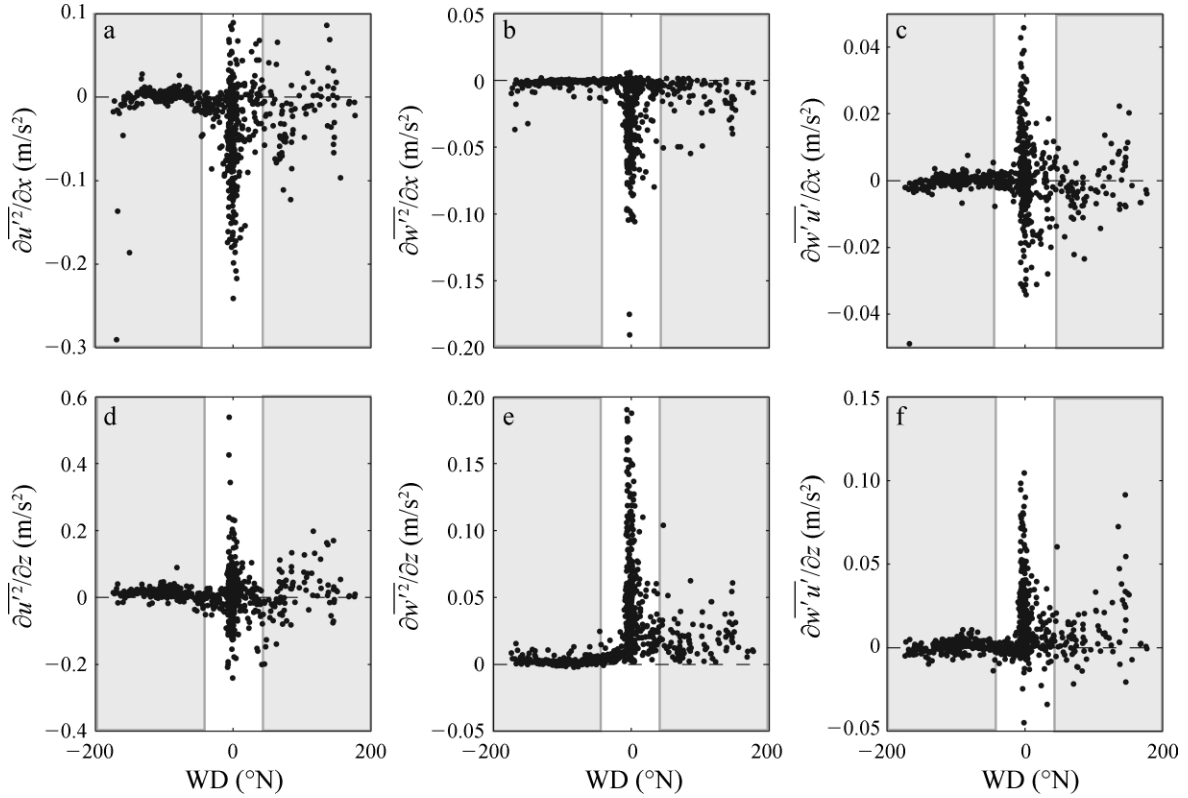
FIG. 7. Same as Fig. 5, but for the second-order statistics: (a) \partial \overline{u'^2}/\partial x , (b) \partial \overline{w'^2}/\partial x , (c) \partial \overline{w'u'}/\partial x , (d) \partial \overline{u'^2}/\partial z , (e) \partial \overline{w'^2}/\partial z , and (f) \partial \overline{w'u'}/\partial z .
