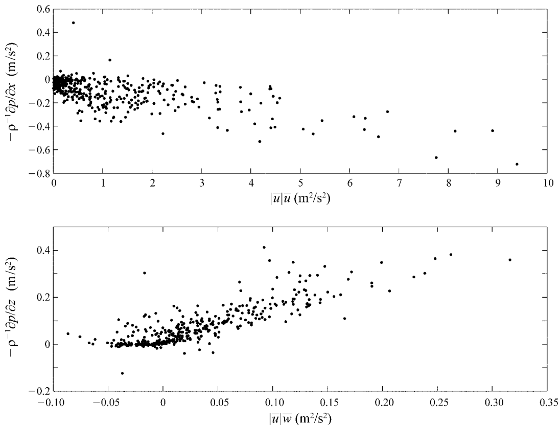
FIG. 10. The variation of -\rho^{-1} \partial \bar{p} / \partial x (top) and -\rho^{-1} \partial \bar{p} / \partial z (bottom) against local variations in |\bar{u}| \bar{u} and |\bar{u}| \bar{w} , respectively, are shown at the forest edge for northerly wind directions. Note that these pressure gradients are determined as residuals from the mean momentum balance.
