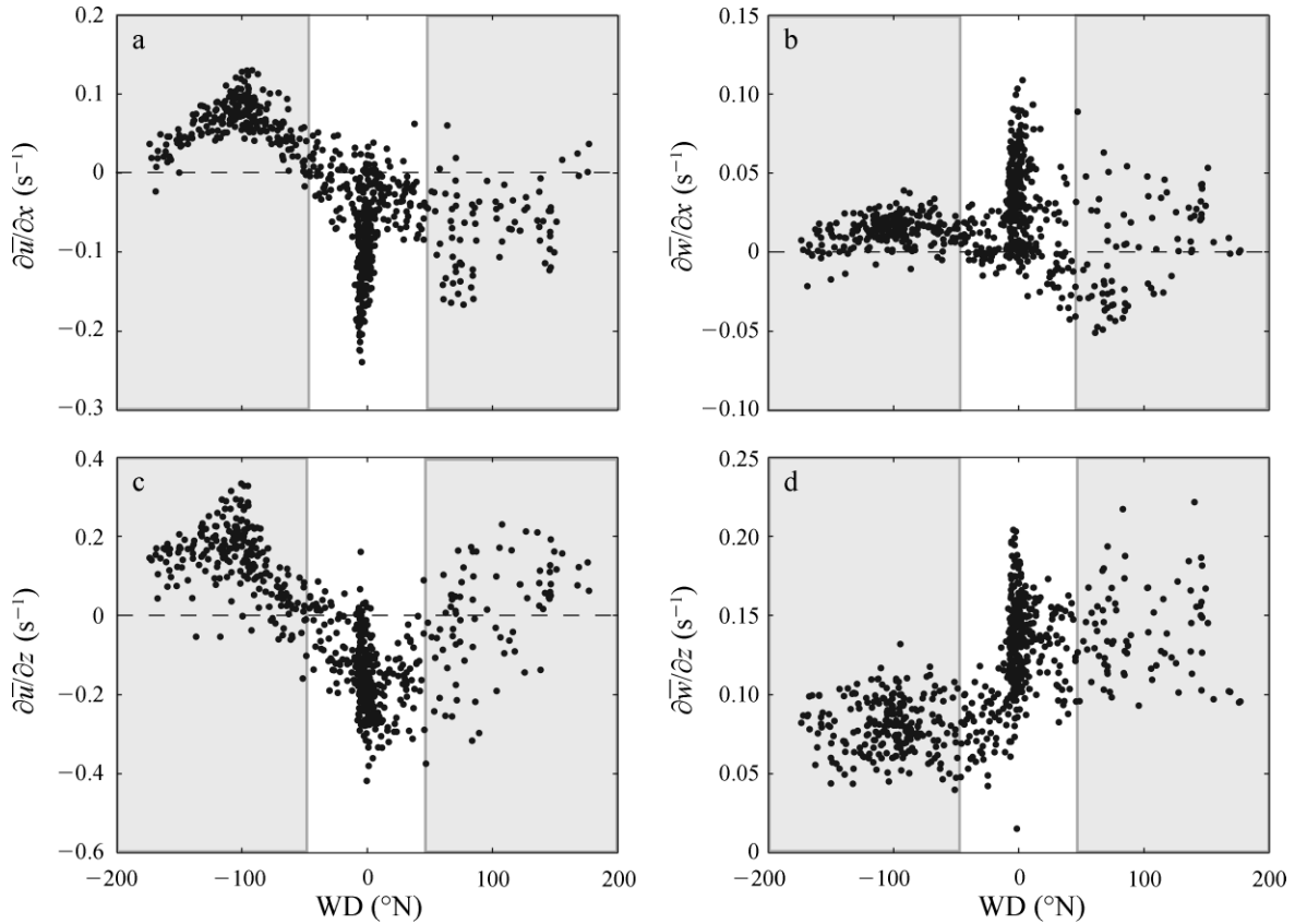
FIG. 6. Variations of (a) \partial \bar{u} / \partial x , (b) \partial \bar{w} / \partial x , (c) \partial \bar{u} / \partial z , and (d) \partial \bar{w} / \partial z with the mean wind direction (WD) evaluated at the center of the field. Flow originates from the forest into the clearing under northerly wind directions \in [0 \pm 45^\circ] . Data shown in gray shaded areas are for all other directions. Note that tower distortions and sonic anemometer overshadowing are significant for WD \in [50, 150] .
