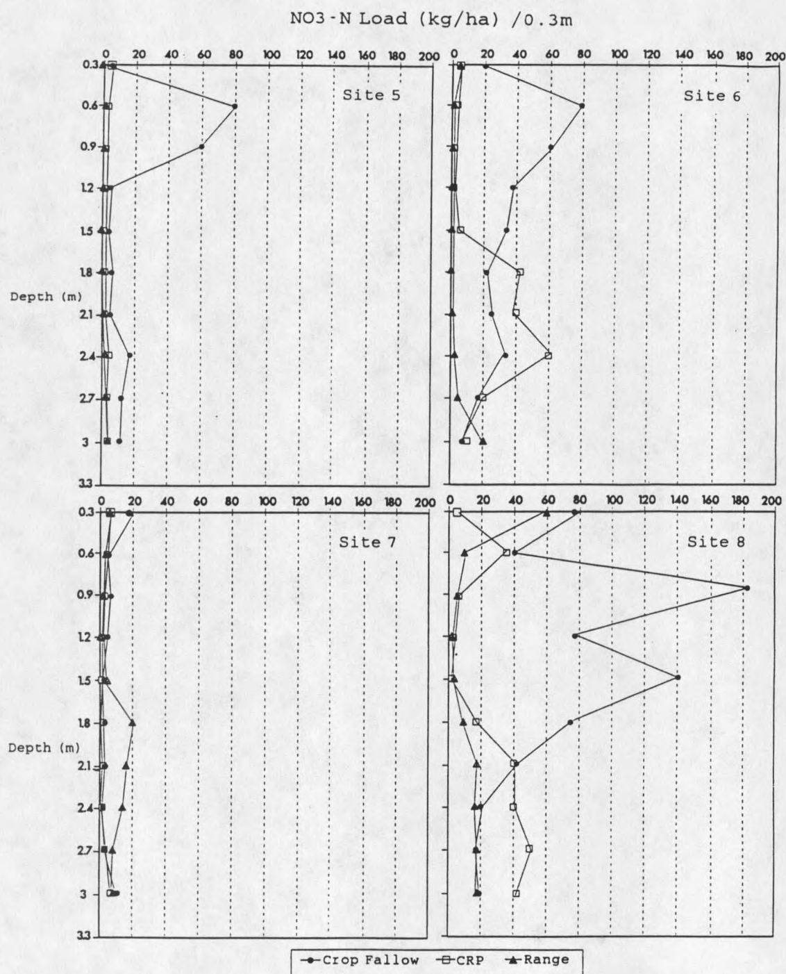
Figure 21. NO 3 - -N load (kg/ha 0.3m) for crop fallow, CRP, and range land use systems for sampled sites in Fergus County, MT.
