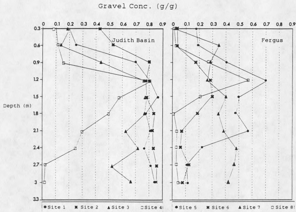
Figure 15. Gravel concentration (g/g) for sampled sites in Judith Basin and Fergus Counties, MT.
