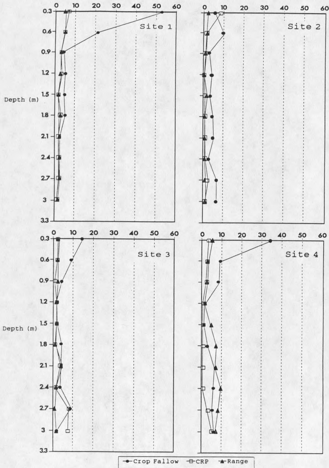
Figure 20. NO 3 - -N load (kg/ha 0.3m) for crop fallow, CRP, and range land use systems for sampled sites in Judith Basin County, MT.
