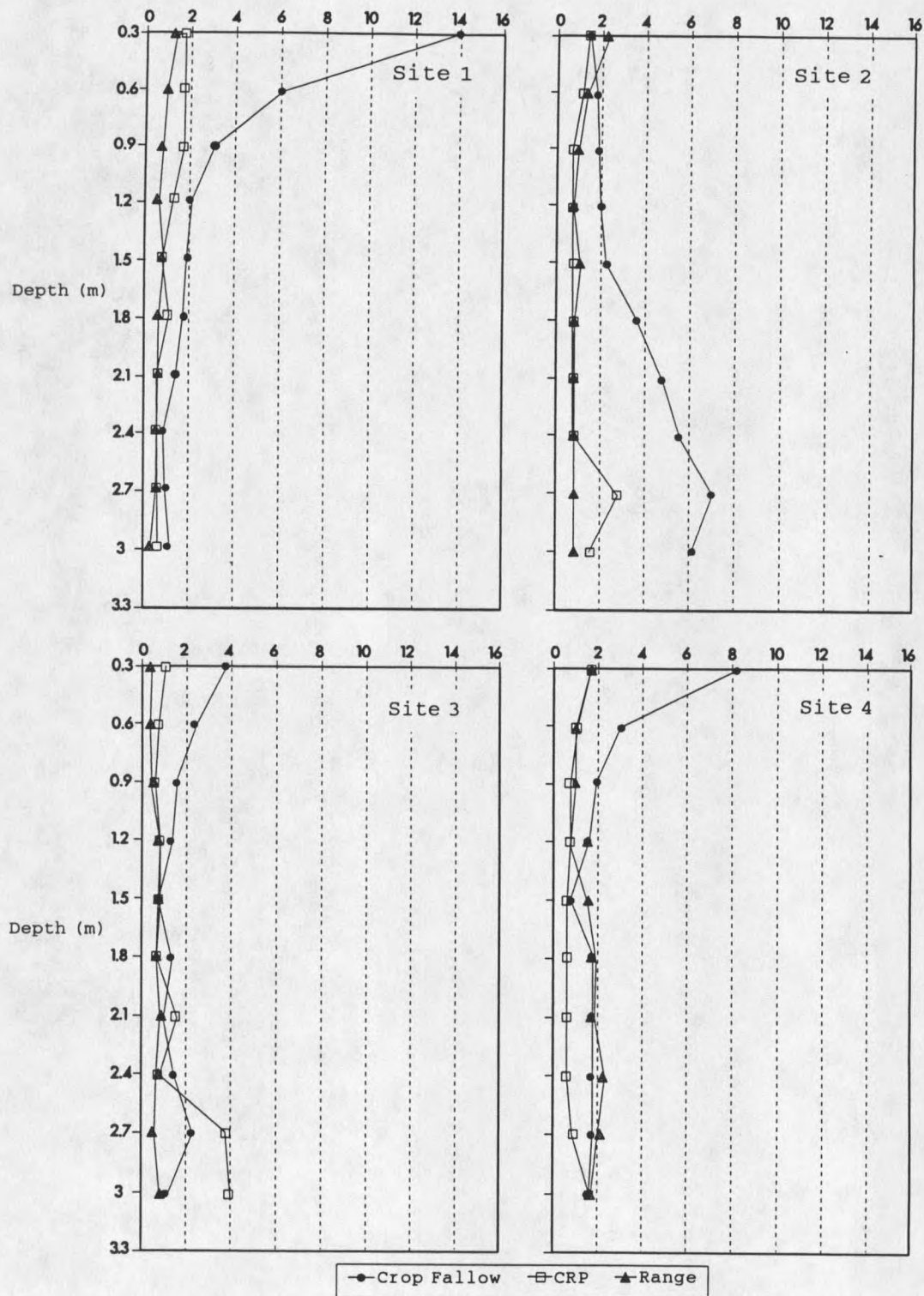
Figure 16. NO 3 - -N concentration (mg/kg) for crop fallow, CRP, and range land use systems for sampled sites in Judith Basin County, MT.
