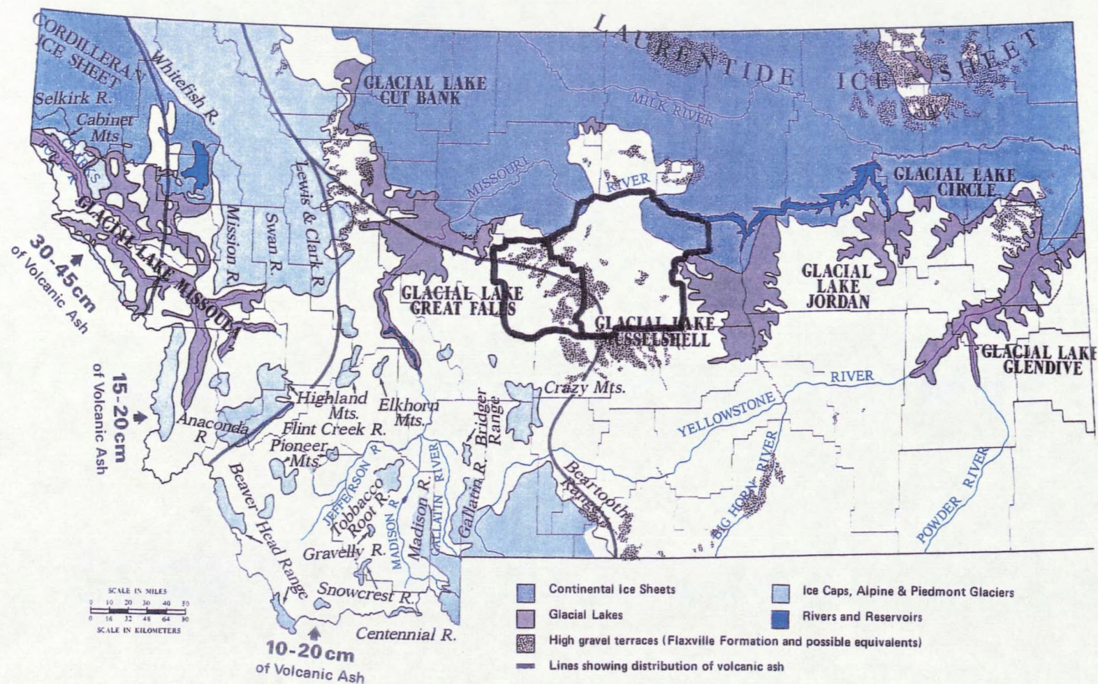
Figure 3. Location of high gravel terraces in Judith Basin and Fergus Counties, Montana (Montagne et al., 1982).
