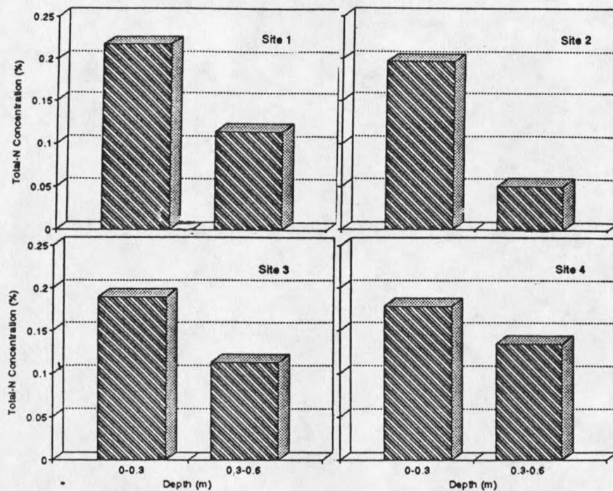
Figure 18. Total-N concentration (% of sample) for individual sampling sites in Judith Basin County at depths 0 to 0.3m and 0.3 to 0.6m.
