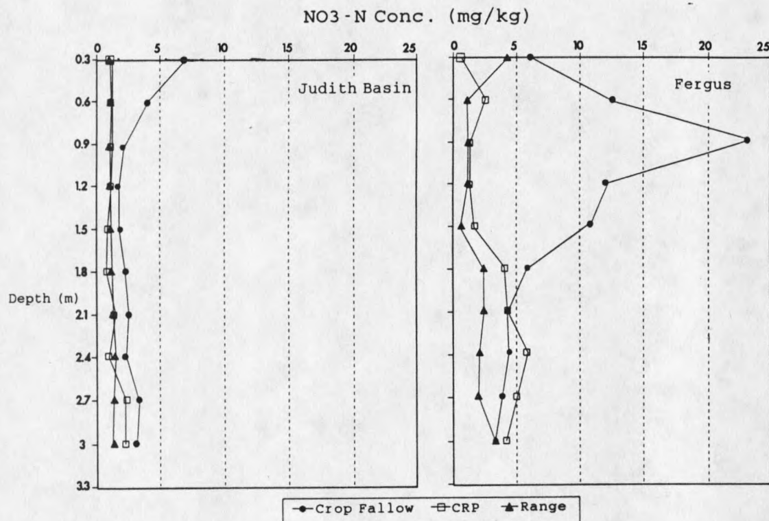
Figure 13. Average \text{NO}_3^- -N concentration (mg/kg) for crop fallow, CRP, and range land use systems for Judith Basin and Fergus Counties, MT, n=4 .
