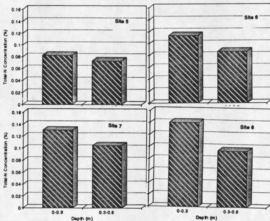
Figure 19. Total-N concentration (% of sample) for individual sampling sites in Fergus County at depths 0 to 0.3m and 0.3 to 0.6m.
