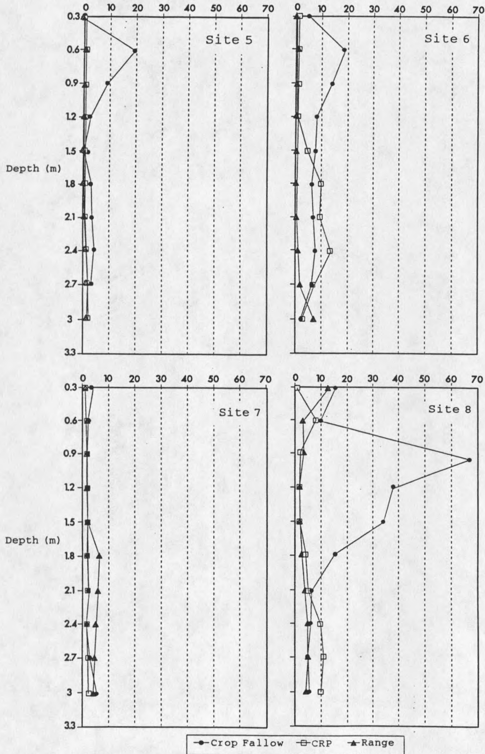
Figure 17. NO 3 - -N concentration (mg/kg) for crop fallow, CRP, and range land use systems for sampled sites in Fergus County, MT.
