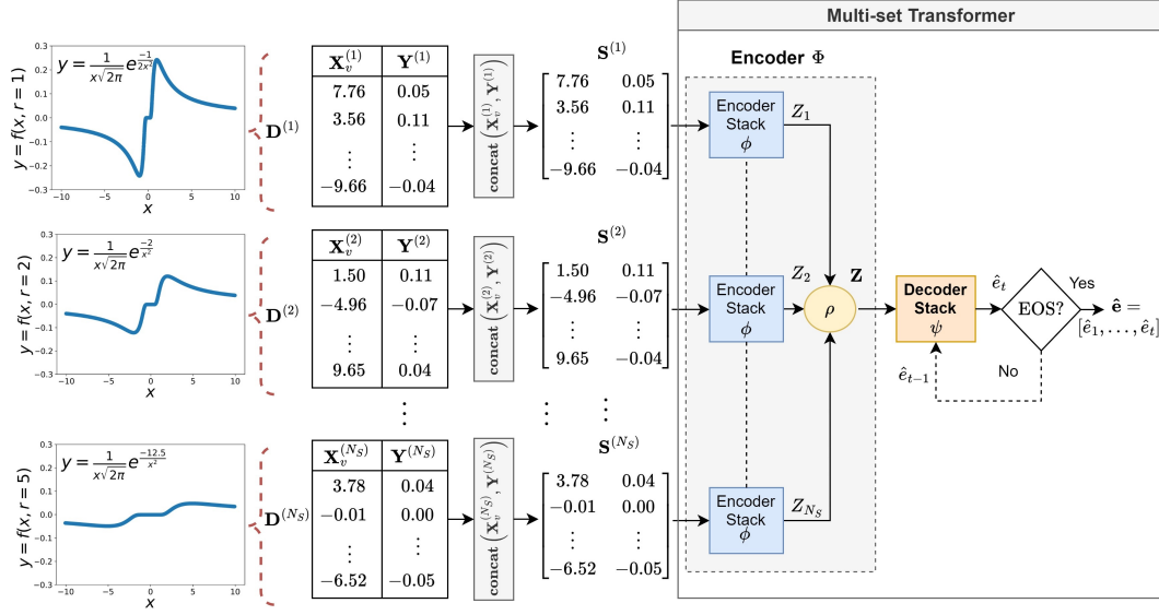
Figure 6: An example of an MSSP problem using the Multi-Set Transformer.
