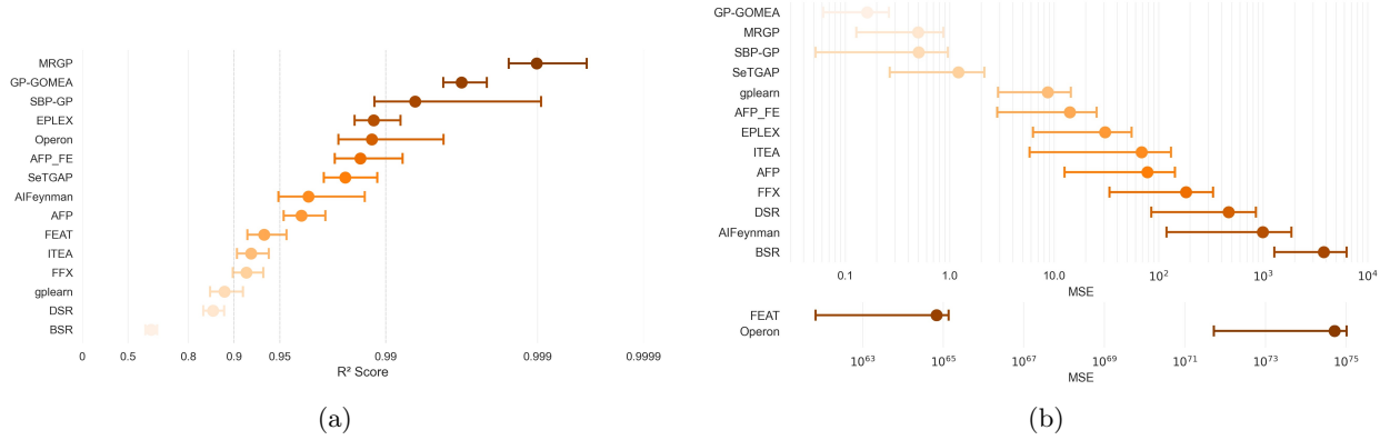
Figure 5: Comparison of the (a) R^2 and (b) MSE distributions obtained on the Feynman dataset
