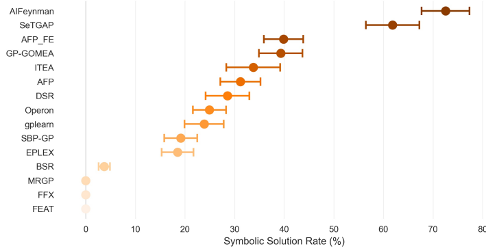
Figure 4: Comparison of the symbolic solution recovery rate distribution obtained on the Feynman dataset
