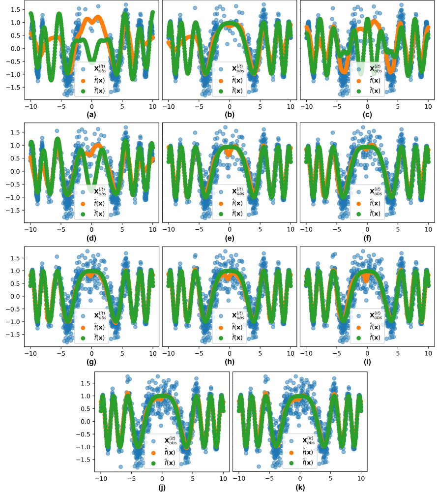
Figure 3: \hat{f}_{it}(\mathbf{x}) vs. \tilde{f}_{it}(\mathbf{x}) throughout the AS process for cosqr . it = (a) 1 (b) 5 (c) 10 (d) 15 (e) 20 (f) 25 (g) 30 (h) 35 (i) 40 (j) 45 (k) 50 (Morales & Sheppard, 2026)
