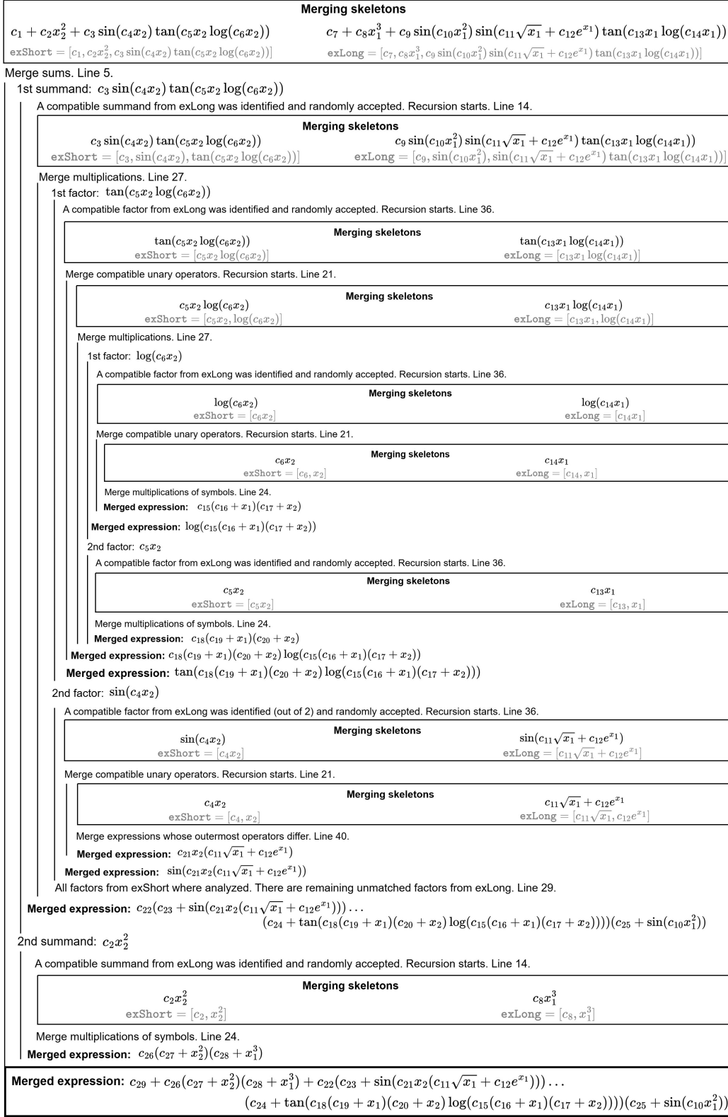
Figure 7: Example of a random merging process, according to Algorithm 2.
