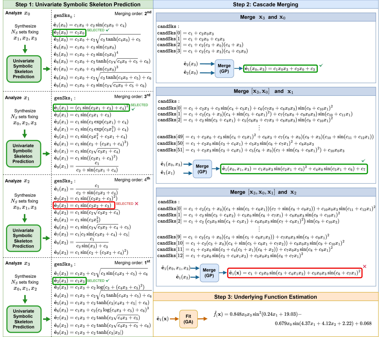
Figure 9: SeTGAP result for Feynman problem I.50.26 with f(\mathbf{x}) = x_0 x_3 \cos^2(x_1 x_2) + \cos(x_1 x_2)
