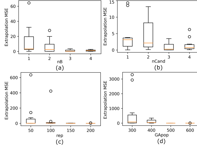
Figure 8: Ablation experiments for (a) n_B , (b) n_{cand} , (c) rep , and (d) GA_{pop} .
