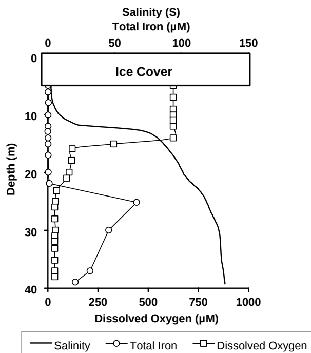
Figure 2. Geochemical profile for West Lobe Lake Bonney. The lake is covered by 4.5 m of permanent ice. The solid line represents salinity, open circles represent total iron and open squares show dissolved oxygen.
