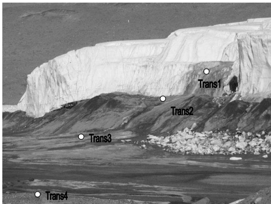
Figure 1. Blood Falls at the terminus of the Taylor Glacier in December 2002. Transect sample collection points are marked. Trans5 is not visible in this image.
