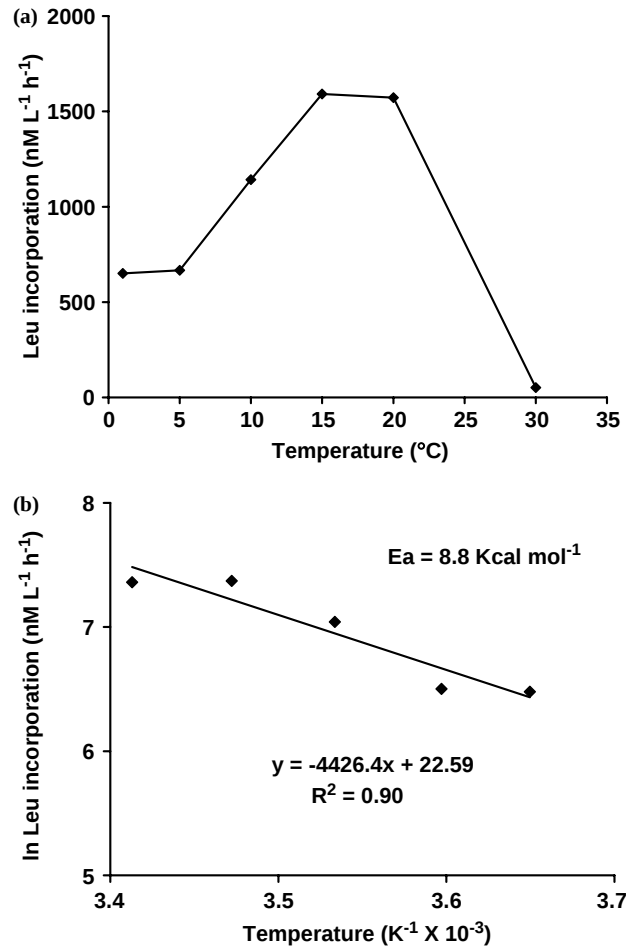
Figure 3. Effect of temperature on Blood Falls outflow plotted arithmetically (a) and with the Arrhenius equation (b).
