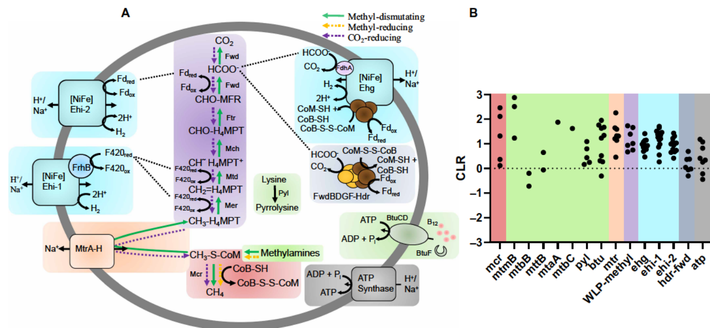
Fig. 3. Proposed methane, hydrogen, and formate metabolism in Ca. M. fastidiosum YNP3N. (A) Metabolic reconstruction of methanogenesis, energy conservation, and vitamin B12 import in YNP3N. A list of genes used to construct this figure can be found in table S4. (B) Gene expression of YNP3N during growth on MMA ( n = 1 due to low RNA yields) suggests a methyl-dismutating methanogenic lifestyle. Dotted line represents the geometric mean expression of all genes. Unless a specific subunit is listed, each dot represents the expression of a subunit in a multisubunit enzyme or functional class, or expression of multiple copies of a particular gene. Explicit values can be found in table S5.
