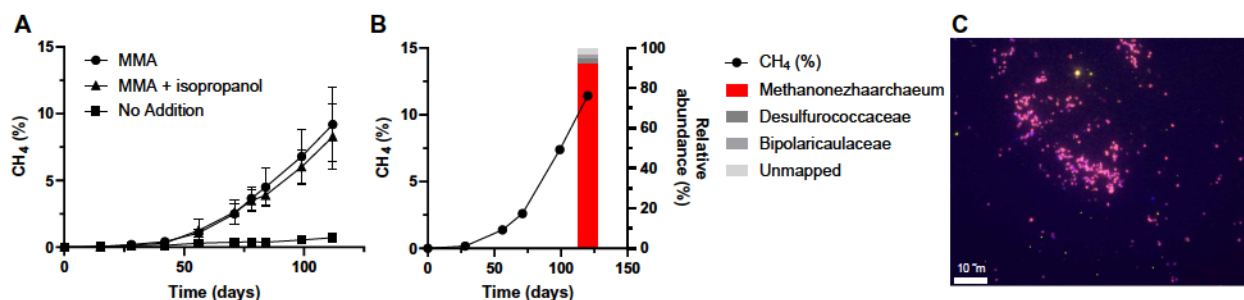
Fig. 1. Enrichment cultivation and visualization of Ca. Methanonezhaarchaeum fastidiosum YNP3N. (A) Methane production by the culture under varying amendments: MMA only ( n = 9 ), MMA and isopropanol ( n = 9 ), and no addition ( n = 3 ). Symbols are the mean from biological replicates and error bars are one SD. Where not visible the error bars are smaller than the symbol. (B) Long-term cultivation on MMA and multiple transfers produced a sediment-free culture >90% enriched in strain YNP3N according to metagenomics ( n = 1 ). (C) Fluorescence microscopy image of Methanonezhaarchaeia cells imaged by FISH. Abundant coccoid cells double hybridized (appearing in pink) with a general archaeal probe (Arch915, red) and a probe specific to Methanonezhaarchaeia (Mnez277, yellow). Cells were counterstained with DAPI (blue). Bright yellow signals stem from autofluorescent sediment particles.
