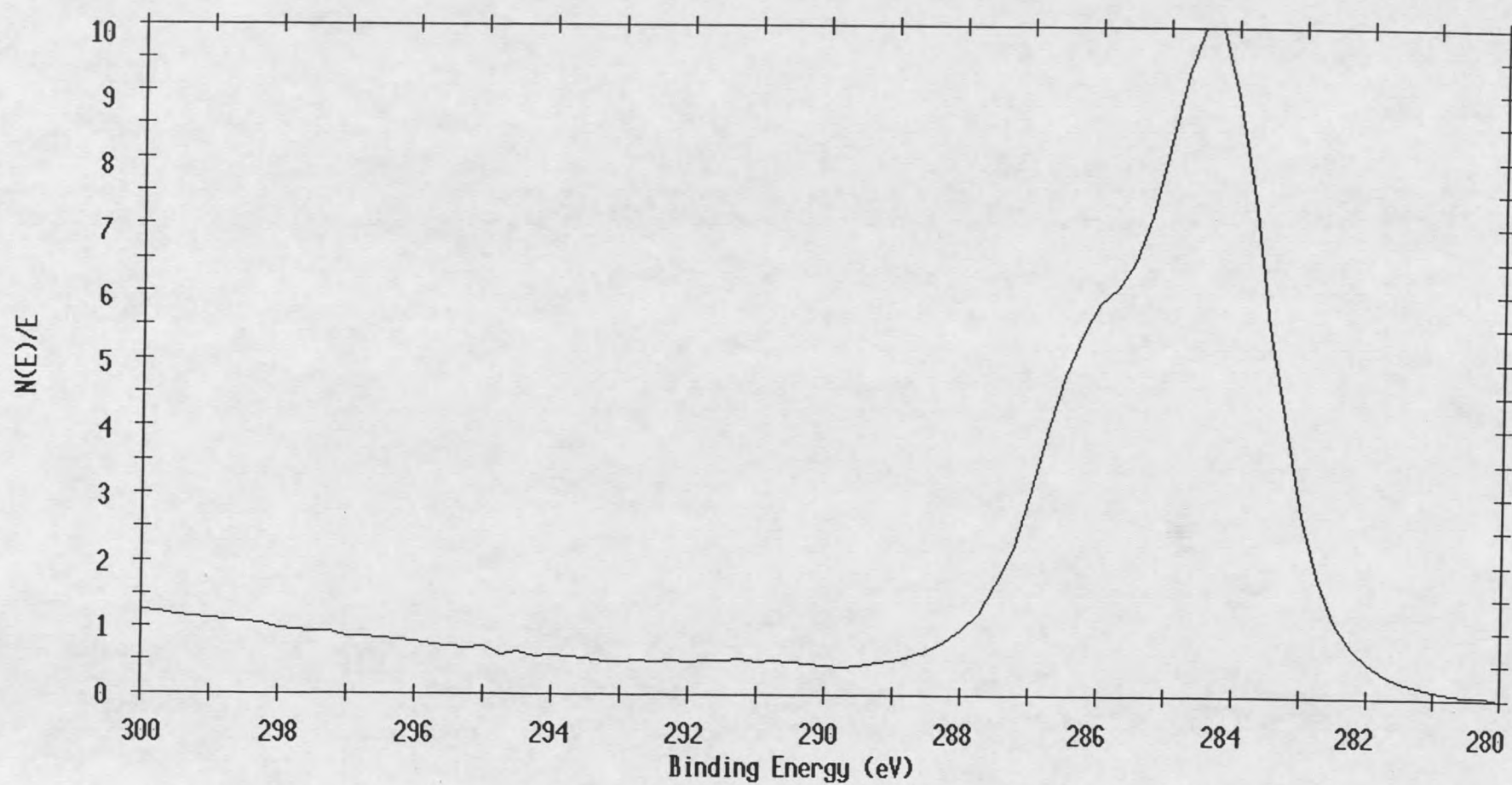
Figure 21. XPS Carbon Spectrum for Coated Fiber
