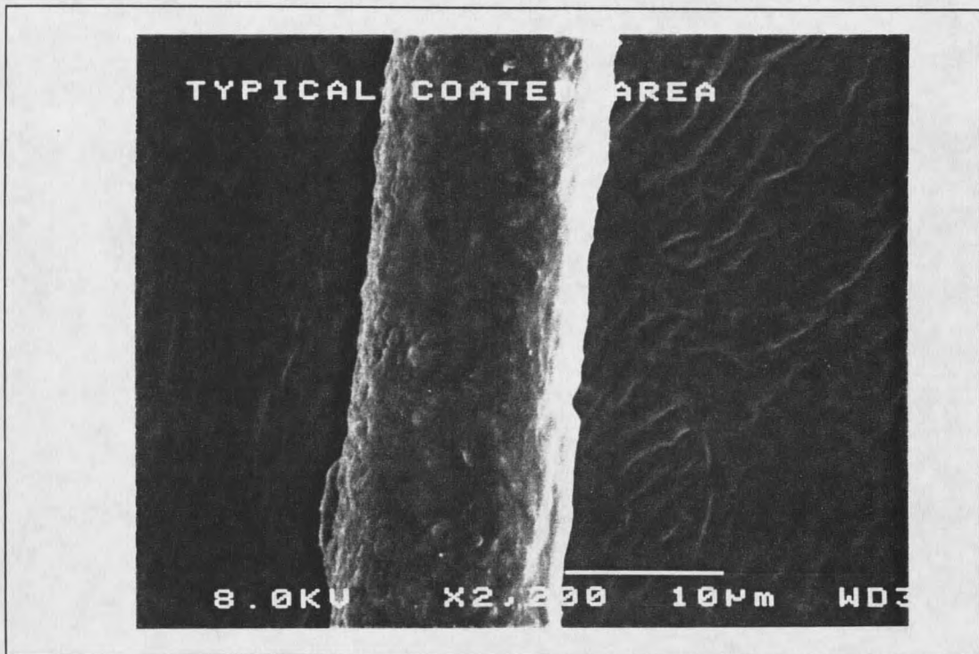
Figure 18. SEM Image of 5% Graphite Coated Fiber
