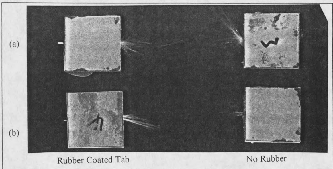
Figure 24. Photograph of Half of Broken Specimens (a) Static Test (b) Fatigue Test With and Without Rubber Coated Tabs
