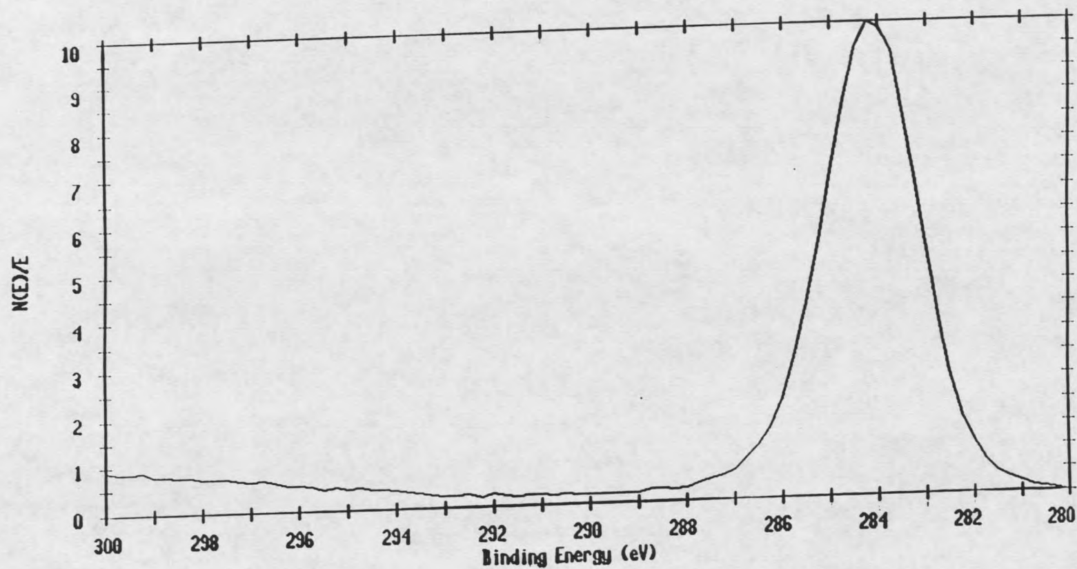
Figure 22. XPS Carbon Spectrum for As-received Fiber
