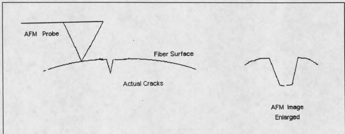
Figure 15. AFM Image of Sharp Crack
