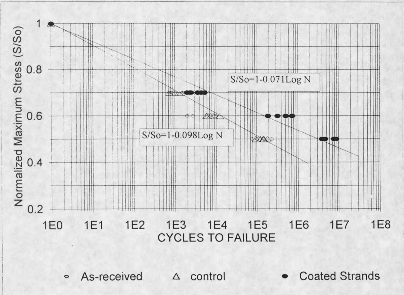
Figure 27. S-N Curves for Glass Fiber Strand Composites With and Without Fiber Coatings, R=0.1
