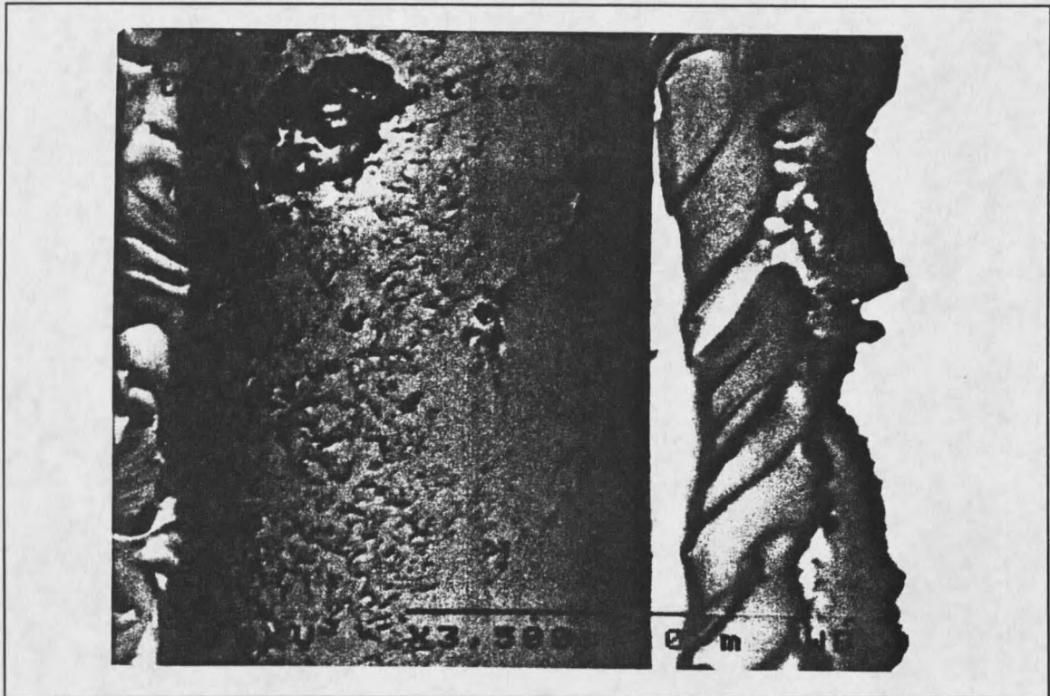
Figure 23. SEM Micrograph of Coated Fiber on Fracture Surface After Transverse Tensile Test
