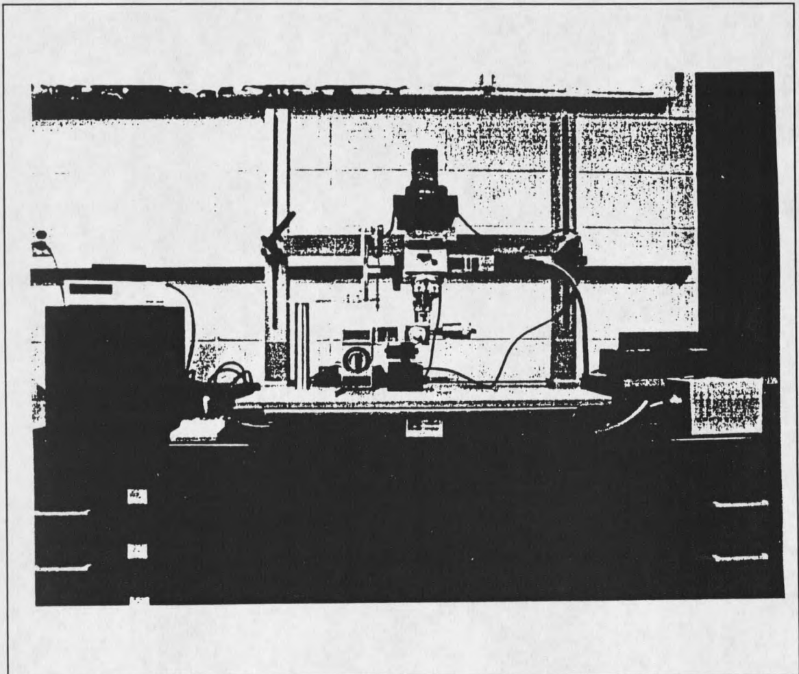
Figure 5. Microdebonding Apparatus
