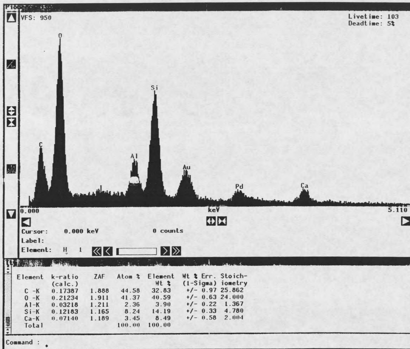
Figure 20. Element Analysis Diagram of Control Fiber
