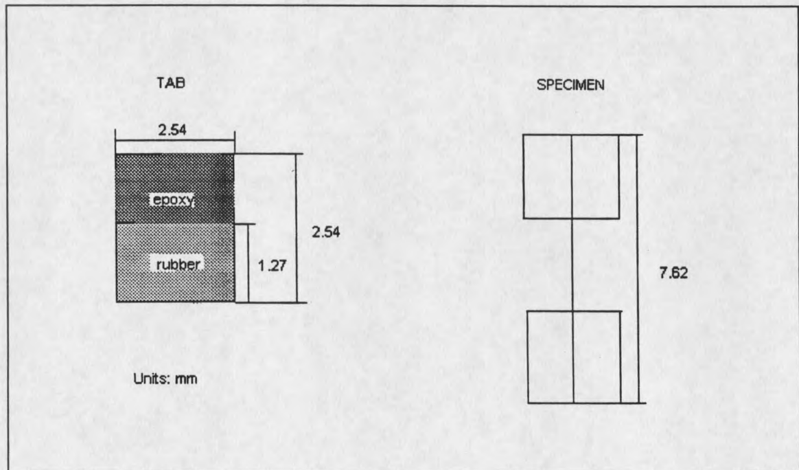
Figure 9. The Geometry of Tab and Strand Composite Specimen
