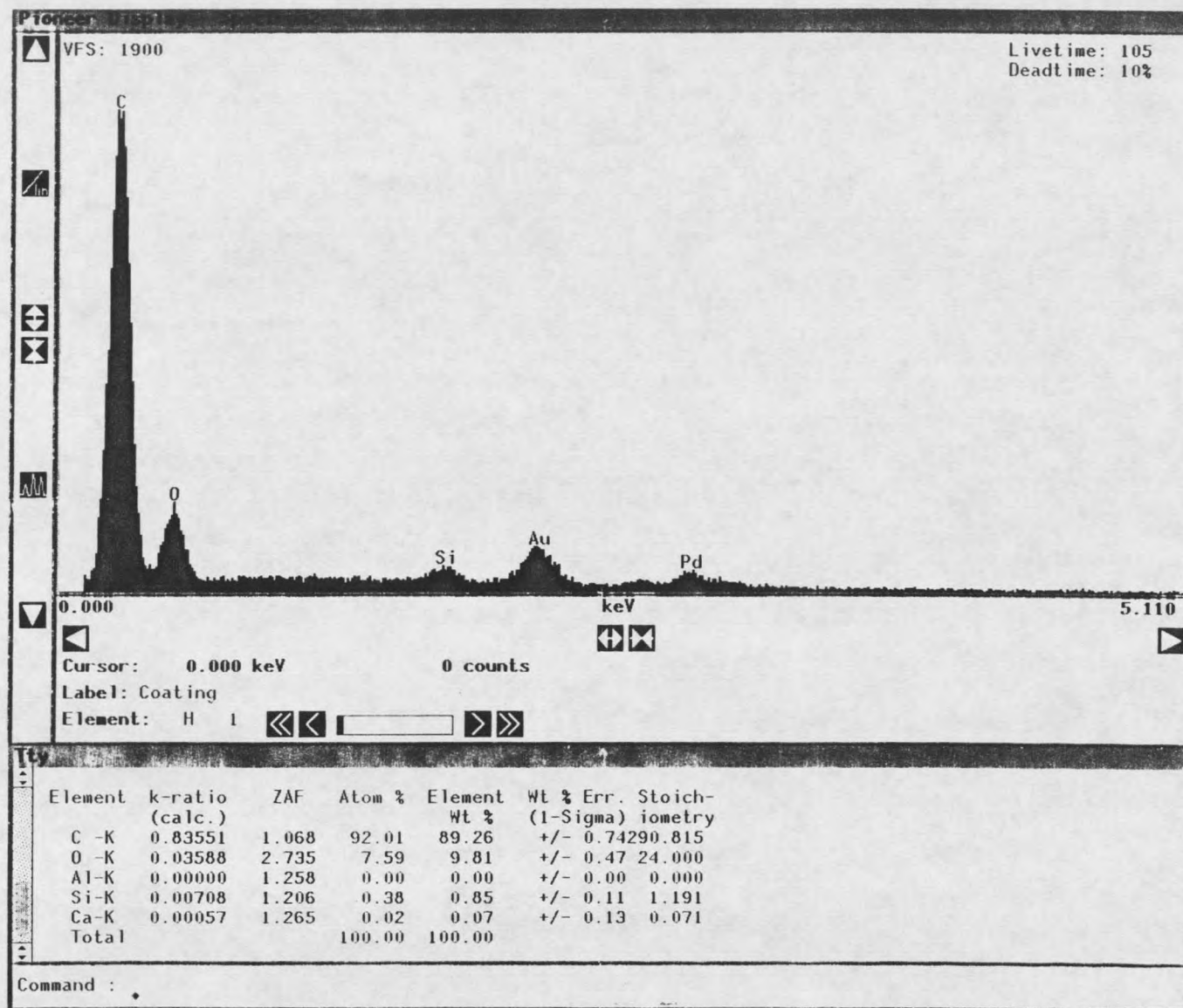
Figure 19. Element Analysis Diagram of Coated Fiber
