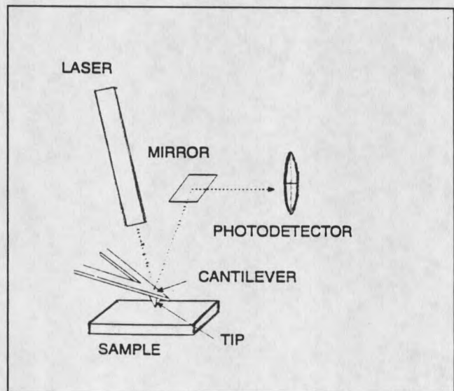
Figure 3 Operation Sketch of AFM detector.
