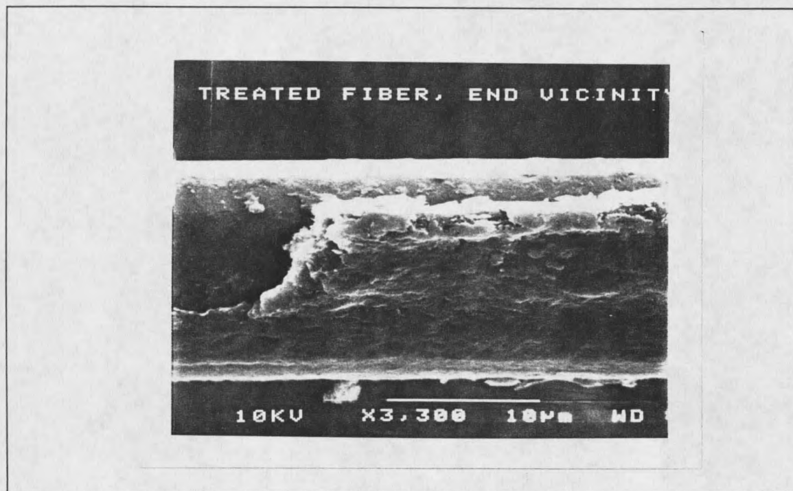
Figure 16. SEM Image of 1% Graphite Coated Fiber
