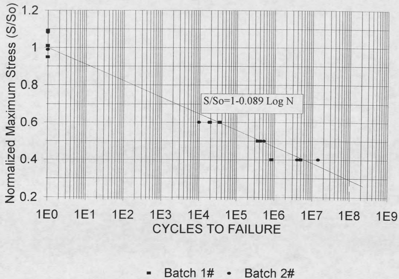
Figure 30. S-N Data for Different Batches of Fabric Composite, R=0.1
