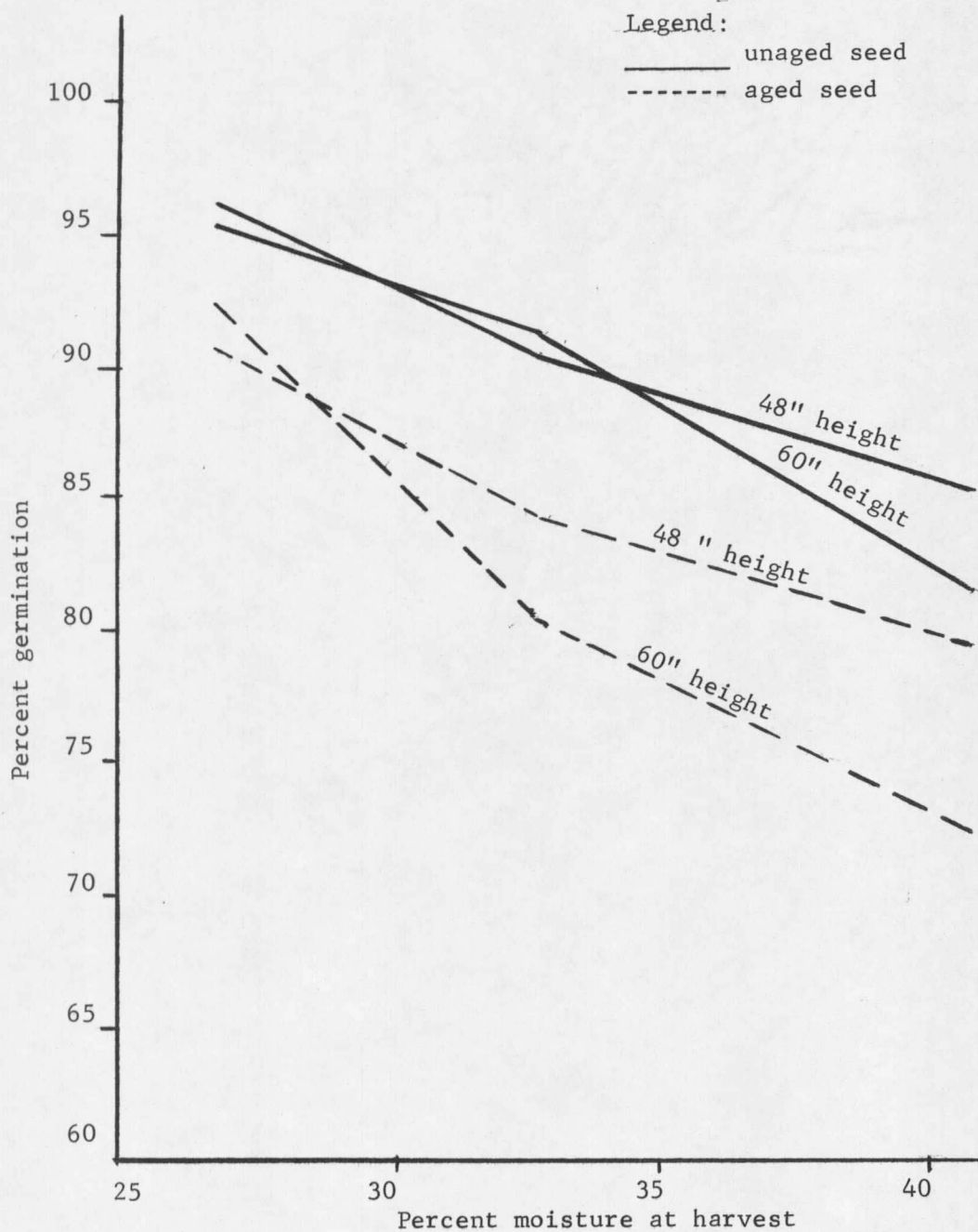
Figure 2. Relationships between moisture at harvest and height of grain in column as they affect germination of aged and unaged seed corn.
