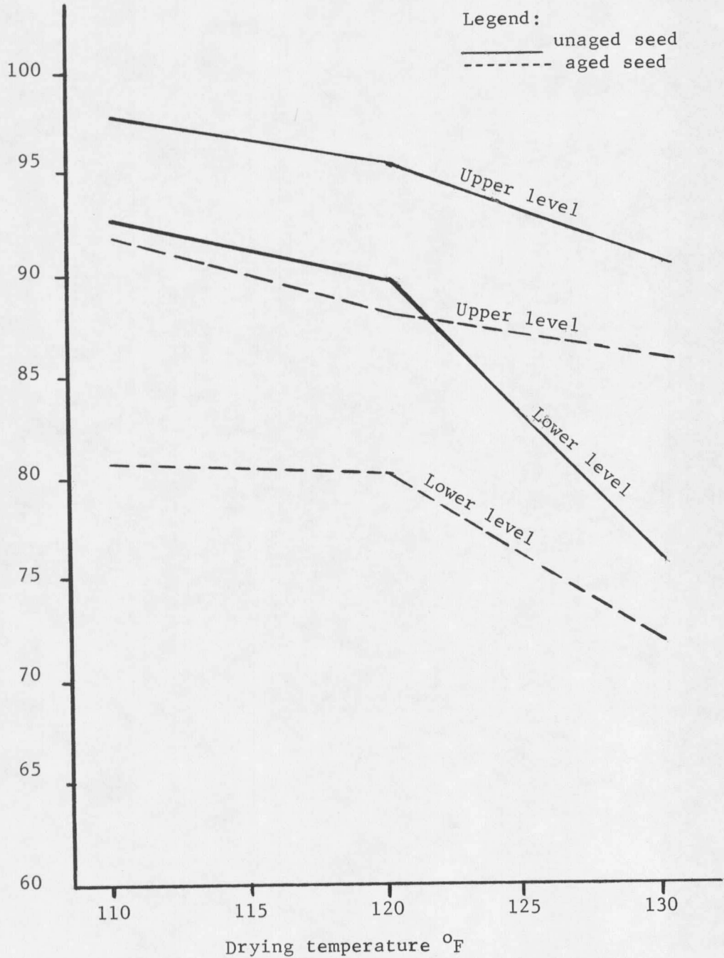
Figure 4. The relationships between temperature and the level in the drying column from which corn is removed as they affect germination of drying aged and unaged corn seed.
