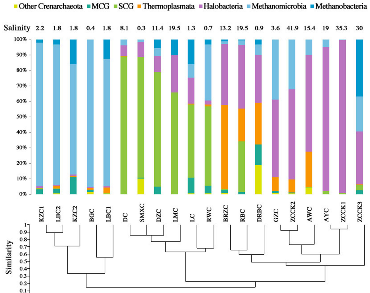
Figure 2. Relative proportions of the archaeal classes within each lake sediment. SCG and MCG represent Soil Crenarchaeotic Group and Miscellaneous Crenarchaeotic Group, respectively. Cluster analysis of archaeal community composition was done using Bray-Curtis similarity; the dendrogram was inferred from an unweighted pair-group average algorithm (UPGMA).
