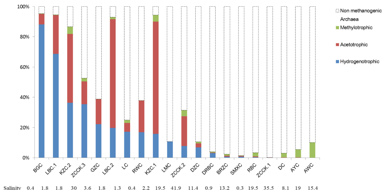
Figure 3. Relative proportions of hydrogenotrophic, acetotrophic and methylotrophic methanogens relative to total archaea in each lake. Columns were arranged in decreasing order of the proportions of hydrogenotrophic methanogens. Sediment salinities are indicated on the x-axis. The hydrogenotrophic methanogens include the genera Methanocella , Methanocalculus , Methanolinea , Methanoregula , Methanoculleus , Methanomicrobium , Methanospirillum , Methanobacterium , Methanobrevibacter and Methanosphaera , and the taxonomically unclassified groups Rice cluster II, LR-13, GOM Arc1 and WCHA2-08. The acetotrophic methanogens include the genera Methanosaeta and Methanosarcina . The methylotrophic methanogens include the genera Methanohalophilus , Methanolobus , Methanomethylovorans and Methanosalsum .
