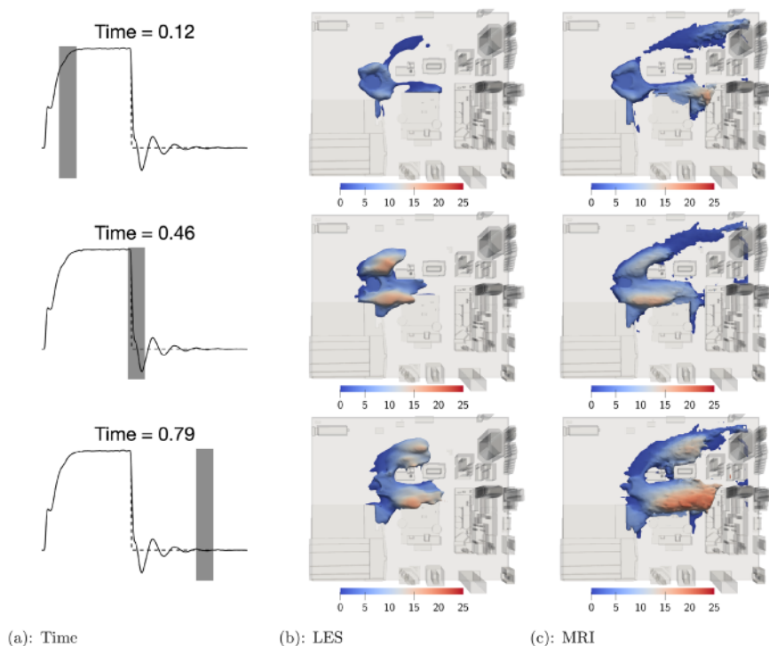
Fig. 12 Comparison of 5% isosurface of contaminant colored by vertical position (mm) for LES (center column) and MRI (right column). Results are organized by rows that vary in time. The time associated with each row is shown in the left column, which shows the time with-respect-to contaminant injection phases
