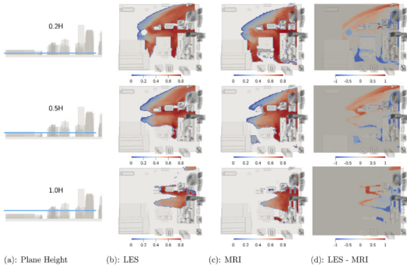
Fig. 15 Comparison of cloud residence time (s) for for LES (b) and MRI (c) and the difference between them (d). Results are organized by rows that vary the non-dimensional height of the cut plane. The height associated with each row is shown by the plane in the left column (a)
