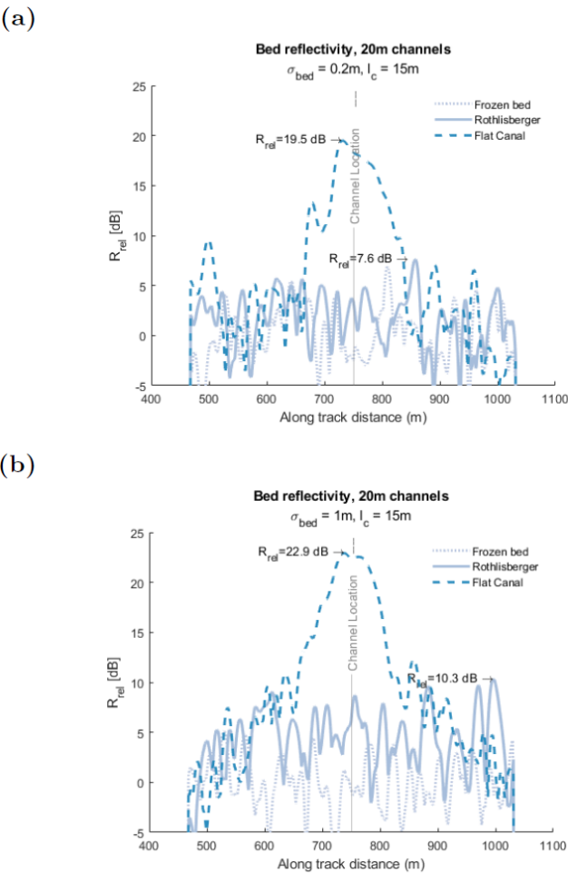
Figure 4. Simulated along-track R_{rel} for 20 m channels compared to a dry substrate with (a) \sigma_{bed} = 0.2 m and (b) \sigma_{bed} = 1 m. All simulations had the same Gaussian roughness correlation length of l_c = 15 m.
