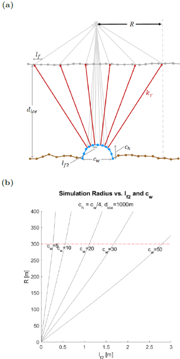
Figure 3. (a) Schematic of simulation geometry for an elliptical cross-section of the Röthlisberger channel at nadir. A second, smaller facet length scale l_{f2} is introduced to facilitate accurate representation of curvature and divergent reflection character. (b) Relationship between R and l_{f2} is defined for a range of c_w . We seek to limit R \leq 300 m for computational efficiency, imposing an upper limit on l_{f2} when simulating Röthlisberger channels
