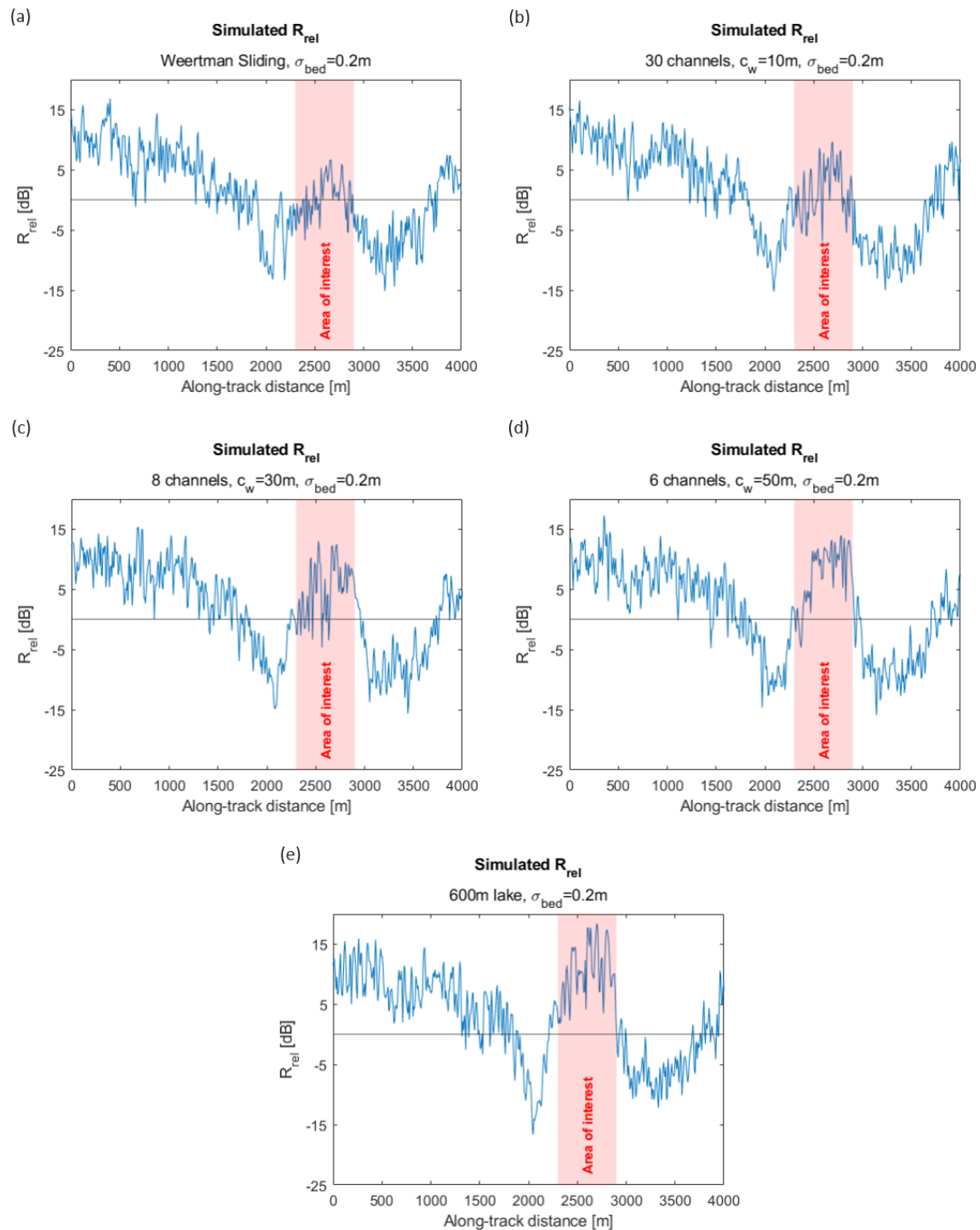
Figure 10. R_{\text{rel}} for distributed hydrology simulations at 2300–2900 m along track. (a) A 600 m wet bed surface (Weertman sliding), (b) 30 flat canals with c_w = 10\text{ m} , (c) 8 flat canals with c_w = 30\text{ m} , (d) 6 flat canals with c_w = 50\text{ m} , and (e) the entire 600 m area covered with a flat, specular waterbody (e.g., sub-glacial lake).
