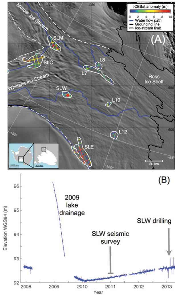
Fig. 1. (a) Overview of the Whillans Ice Plain, with inferred subglacial water flow paths indicated by blue lines (Carter and others, 2013) and subglacial lake outlines by solid white lines (SLC: Subglacial Lake Conway; SLM: Subglacial Lake Mercer; SLW: Subglacial Lake Whillans; SLE: Subglacial Lake Engelhardt; L7: Lake 7; L8: Lake 8; L10: Lake 10; and L12: Lake 12). The red dot on SLW indicates the borehole location. Ice, Cloud and land Elevation Satellite (ICESat) elevation change anomaly amplitudes and lake outlines are from Fricker and Scambos (2009); background imagery and grounding lines (black) come from the Moderate Resolution Imaging Spectroradiometer (MODIS) Mosaic of Antarctica (Scambos and others, 2007); and the lateral limits of fast ice flow (dashed white lines) are derived from Rignot and others (2011). Projection is south polar stereographic (km) with standard latitude at 71° S. (b) The vertical ice motion between late 2007 and early 2013 based on data from a GPS station located ~700 m from the SLW borehole at the time of drilling. The 2009 lake drainage (Siegfried and others, 2014), timing of SLW active-source seismic survey (Horgan and others, 2012) and SLW drilling are labeled for reference.
