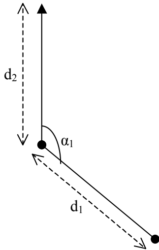
Figure 2A.2. A bison travel vector consisting of two significant movements. By definition, for a significant movement the distance of each segment must be \geq 800 m (i.e., d_1 \geq 800 m; d_2 \geq 800 m) and the turning angle must be \leq 90^\circ .
