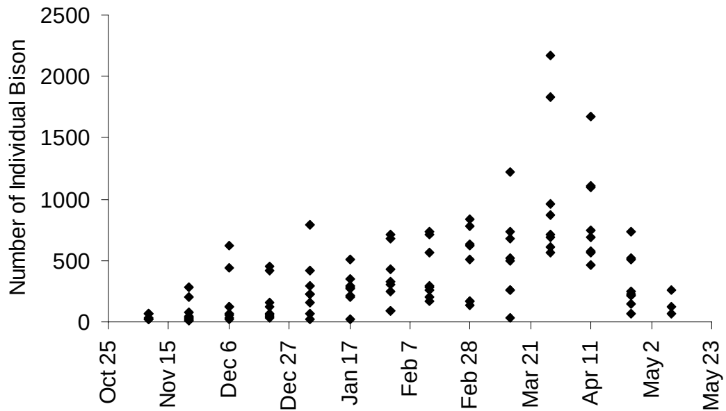
Figure 3C.6. The number of individual bison observed traveling on roads for each period and year during bison road use surveys from 1997-98 through 2004-05.
