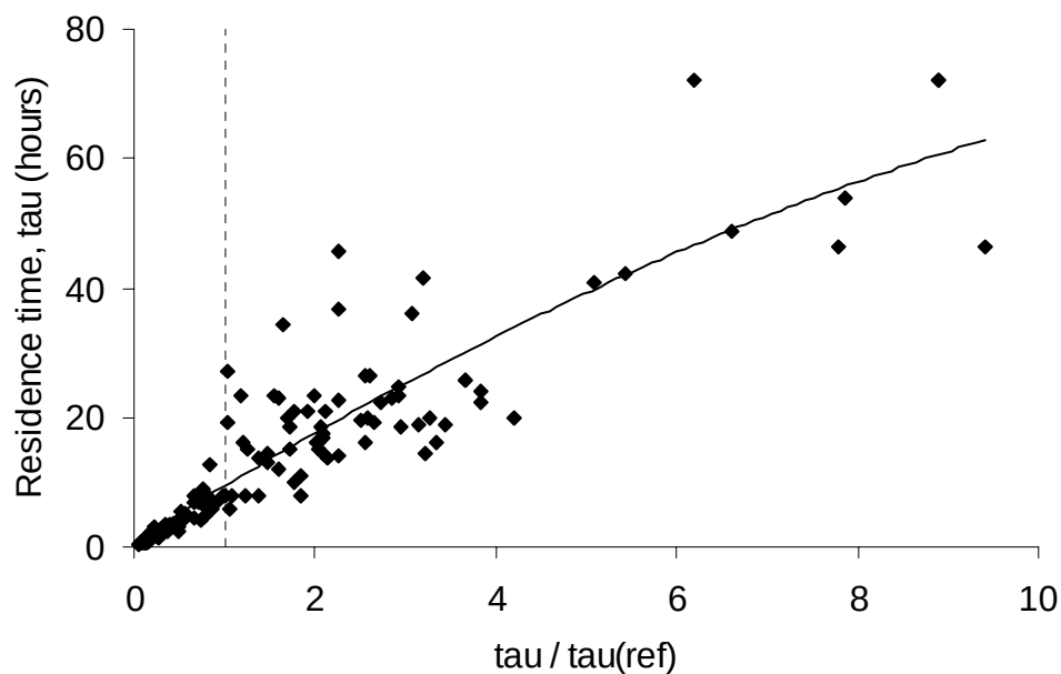
Figure 4.8. Plot of \tau versus \tau/\tau_{ref} for bison foraging areas in the Madison-Gibbon-Firehole area of Yellowstone National Park during January-March 2004 and 2005. Data points to the left of the dashed line denoting \tau/\tau_{ref}=1 indicate areas of negative perceived value; points to the right of the line denote areas of positive perceived value.
