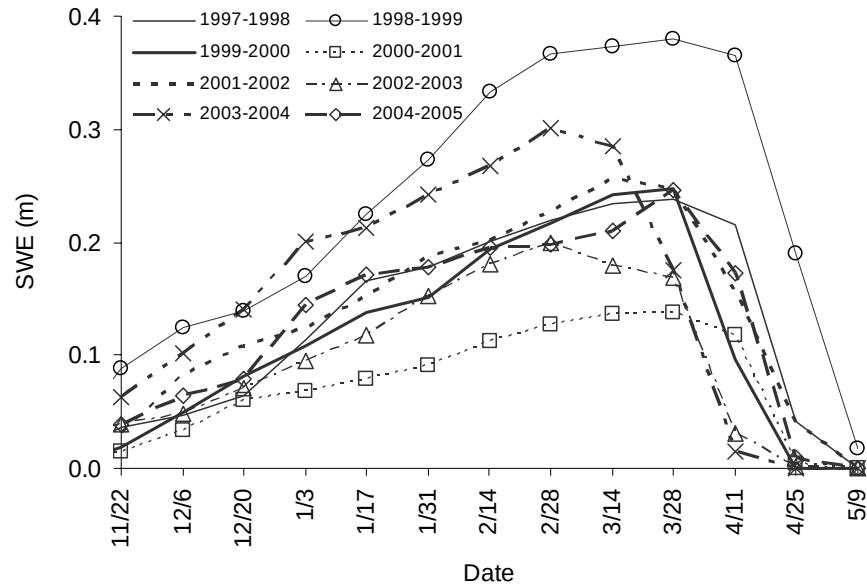
Figure 3.2. Temporal patterns in snow water equivalent in the Madison-Gibbon-Firehole area of Yellowstone National Park during winter, 1997-98 to 2004-05. Snow water equivalent (SWE) values were measured at a SNOTEL site near West Yellowstone, Montana, and averaged over two-week intervals.
