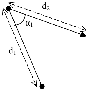
Figure 2A.3. A set of bison vectors that are representative of a foraging or searching trajectory for which the turning angle between segments has a value >90^\circ and/or segment distances ( d ) are <800 m (i.e., d_1 < 800 m; d_2 < 800 m).
