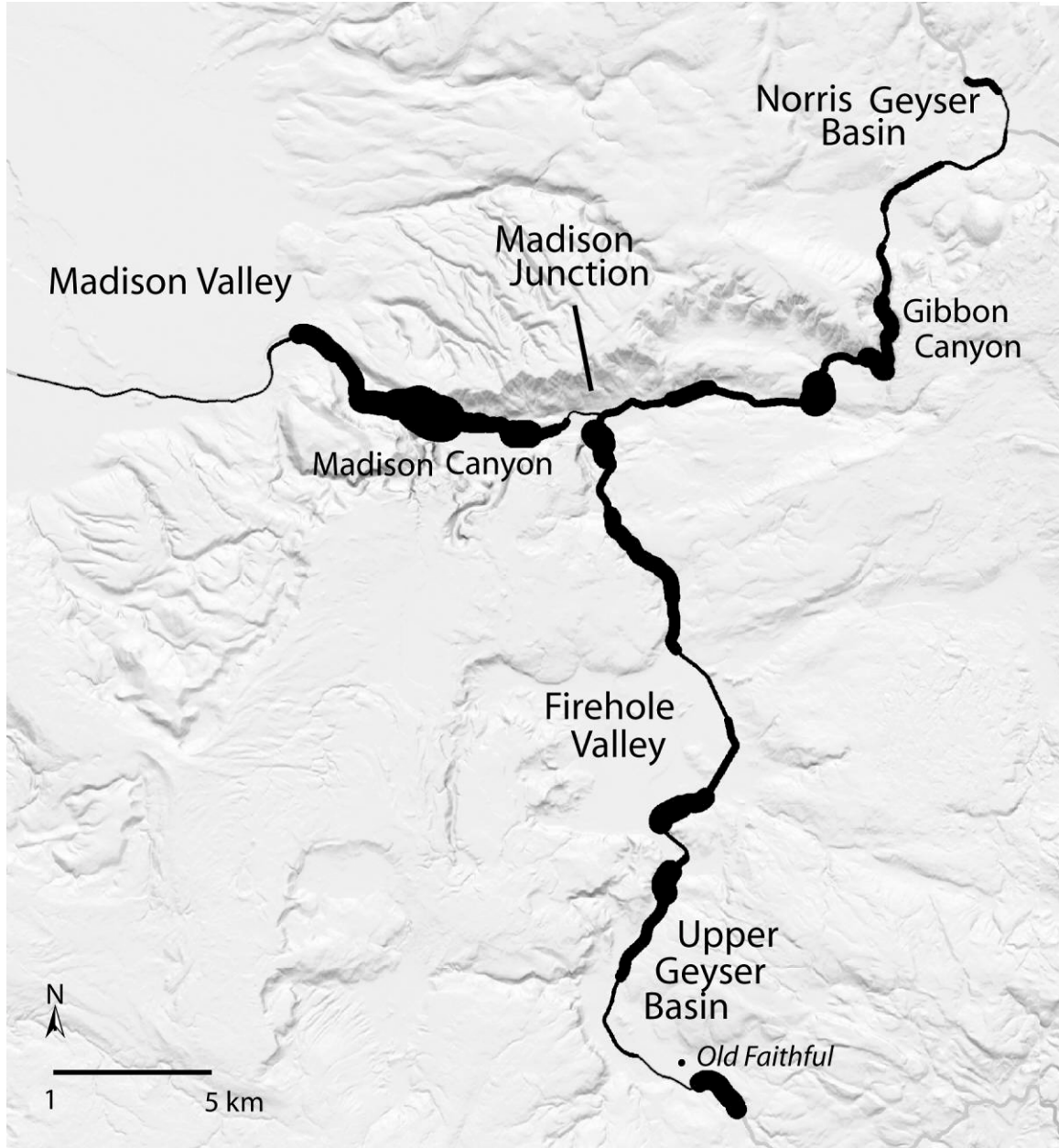
Figure 2.5. Map depicting spatial variability in the amount of bison road travel for the Firehole, Gibbon, and Madison drainages in west central Yellowstone National Park. The width of the black lines represents the magnitude in average bison road travel for each road segment for 2002-03 to 2004-05 with values ranging between 0.0-11.7 bison groups observed in segment/100 km traveled in segment. Roads are depicted in dark gray. Data on bison road use were obtained during winter bison road use surveys conducted from 2002-03 to 2004-05 in the Madison, Gibbon, and Firehole drainages.
