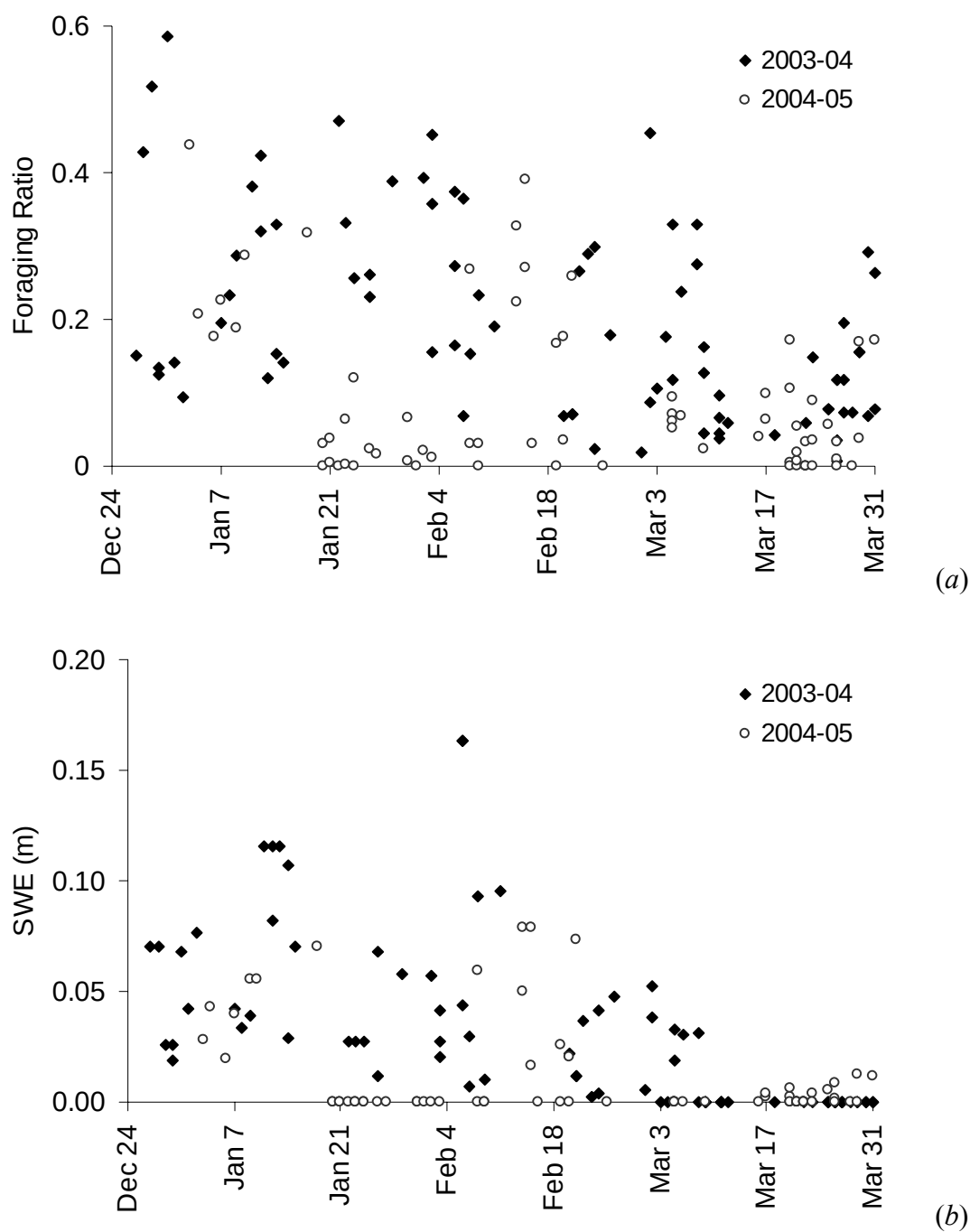
Figure 5.3. Temporal patterns in (a) the foraging ratio from bison observations, and (b) snowpack snow water equivalent (SWE) for bison locations in the Madison-Gibbon-Firehole area of Yellowstone National Park obtained from December-March during 2003-04 and 2004-05.
