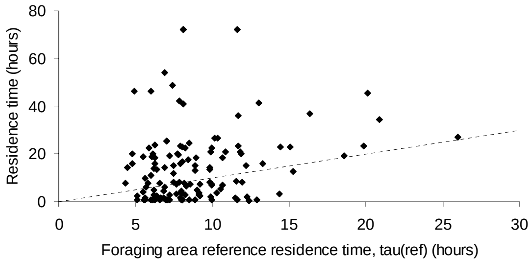
Figure 4.6. Plots of data points for foraging area residence time ( \tau ) versus the reference foraging area residence time ( \tau_{ref} ) with the line \tau = \tau_{ref} denoted. Data are from bison foraging area locations in the Madison-Gibbon-Firehole area of Yellowstone National Park obtained from January-March during 2004 and 2005.
