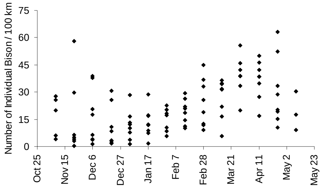
Figure 3C.7. The number of individual bison observed traveling on roads per 100 km of road survey effort for each period and year during bison road use surveys from 1997-98 through 2004-05.
