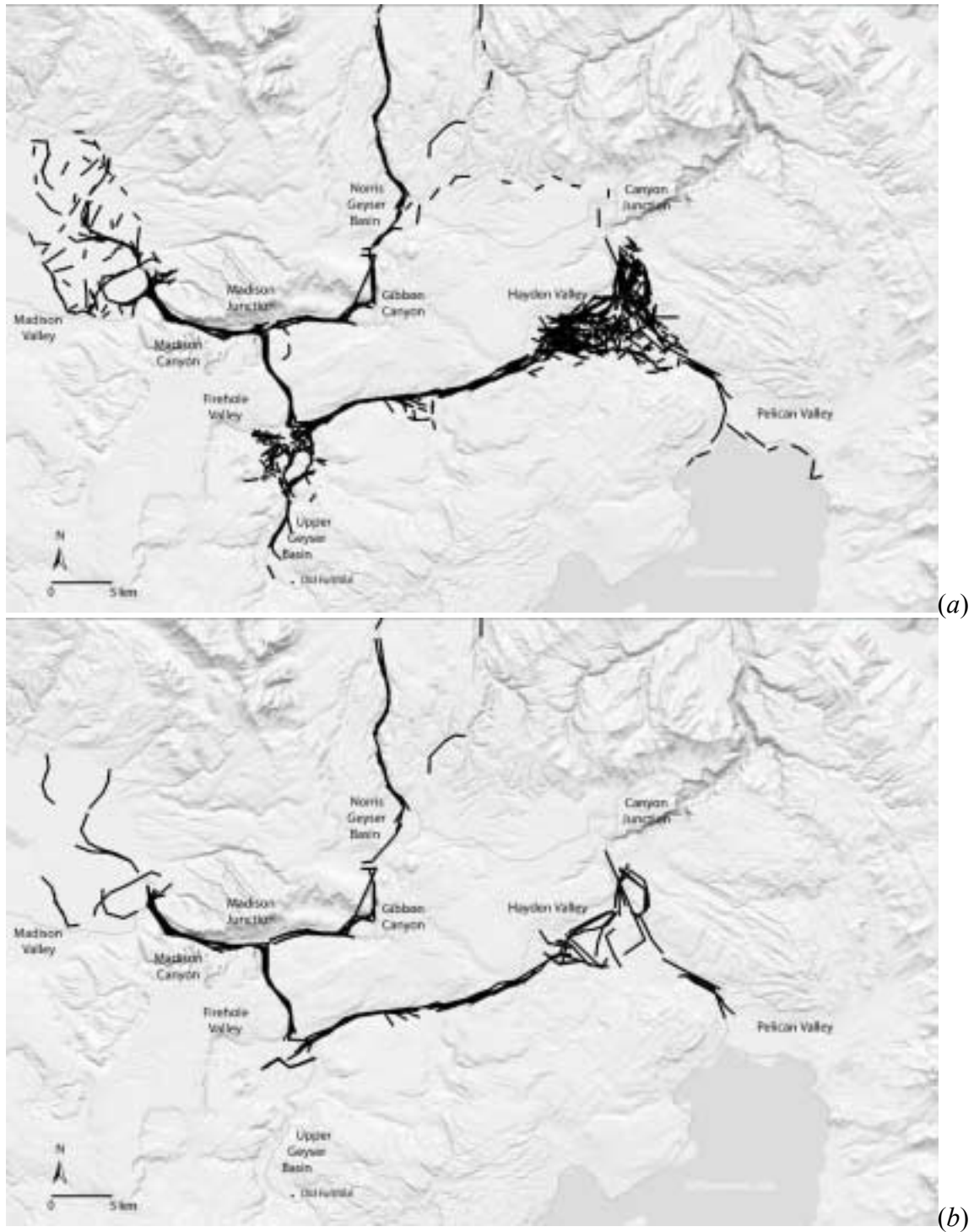
Figure 2.2. Maps of the spatial distribution of vectors from GPS collared bison for (a) general bison travel, and (b) long distance bison travel throughout central Yellowstone National Park. Black lines denote vectors and dark gray lines depict the road system.
