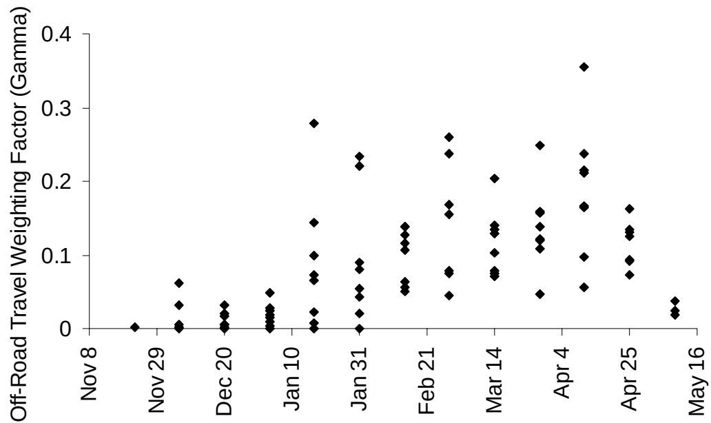
Figure 3C.10. The off-road travel weighting factor ( \gamma_{ij} ) for each period and year as calculated using data from bison ground distribution surveys from 1997-98 through 2004-05.
