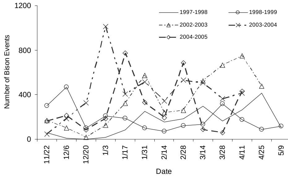
Figure 3.7. Number of bison movement events recorded by a trail monitor on the Mary Mountain trail between the Firehole and Hayden Valleys in Yellowstone National Park. Data were collected during the 1997-1999 and 2002-2005 seasons.
