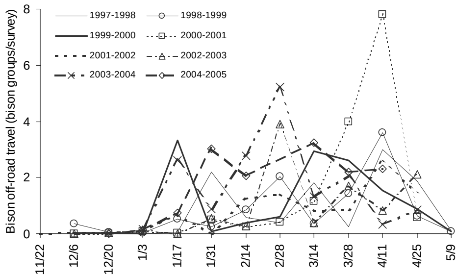
Figure 3.5. Temporal variability in bison off-road travel in the Madison-Gibbon-Firehole area of Yellowstone National Park during winter, 1997-98 to 2004-05. Bison groups traveling off-road per survey ( \tau_{ij} ), calculated from my ground distribution surveys, are presented for each time interval ( i ) and year ( j ).
