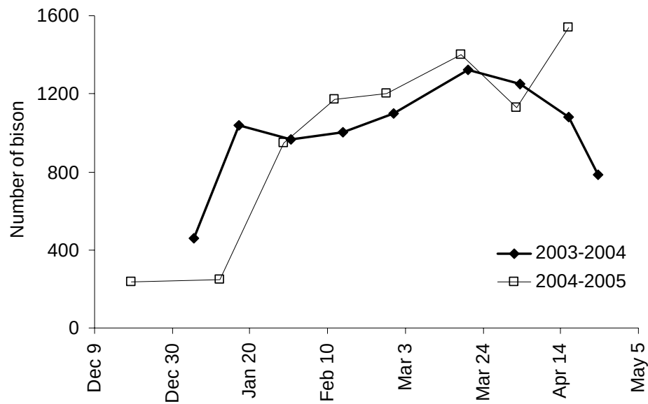
Figure 4.4. Temporal trends in the number of bison in the Madison-Gibbon-Firehole area of Yellowstone National Park as determined from ground surveys conducted every 14 days during December-April 2003-04 and 2004-05. The data were used to determine the BISONMGF covariate.
