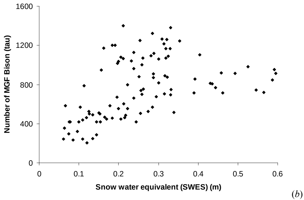
Figure 1.4. Original data demonstrating the relationship between (a) the extent of migration ( \epsilon ) (i.e., maximum number of bison in the Madison-Gibbon-Firehole (MGF)) and DROUGHT, and (b) the timing of migration ( \tau ) (i.e., number of bison in the MGF) and summer range snow water equivalent (SWES).
