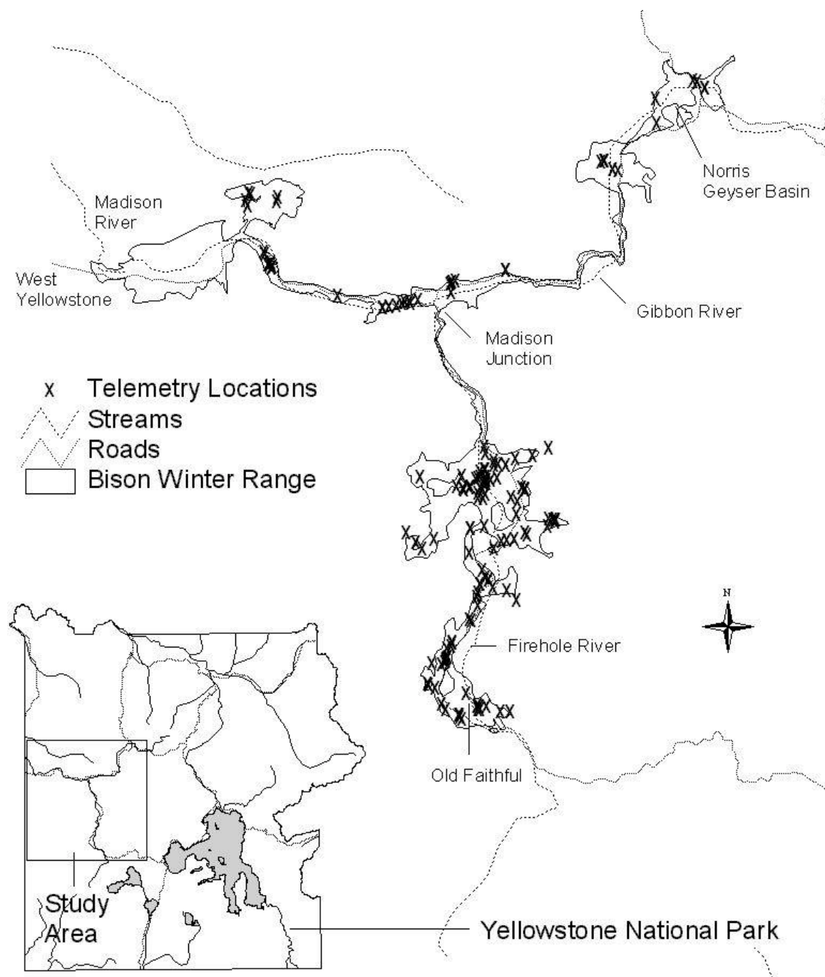
Figure 5.2. The distribution of the 147 telemetry locations throughout the Madison-Gibbon-Firehole study area in Yellowstone National Park obtained from December-March during 2003-04 and 2004-05.
