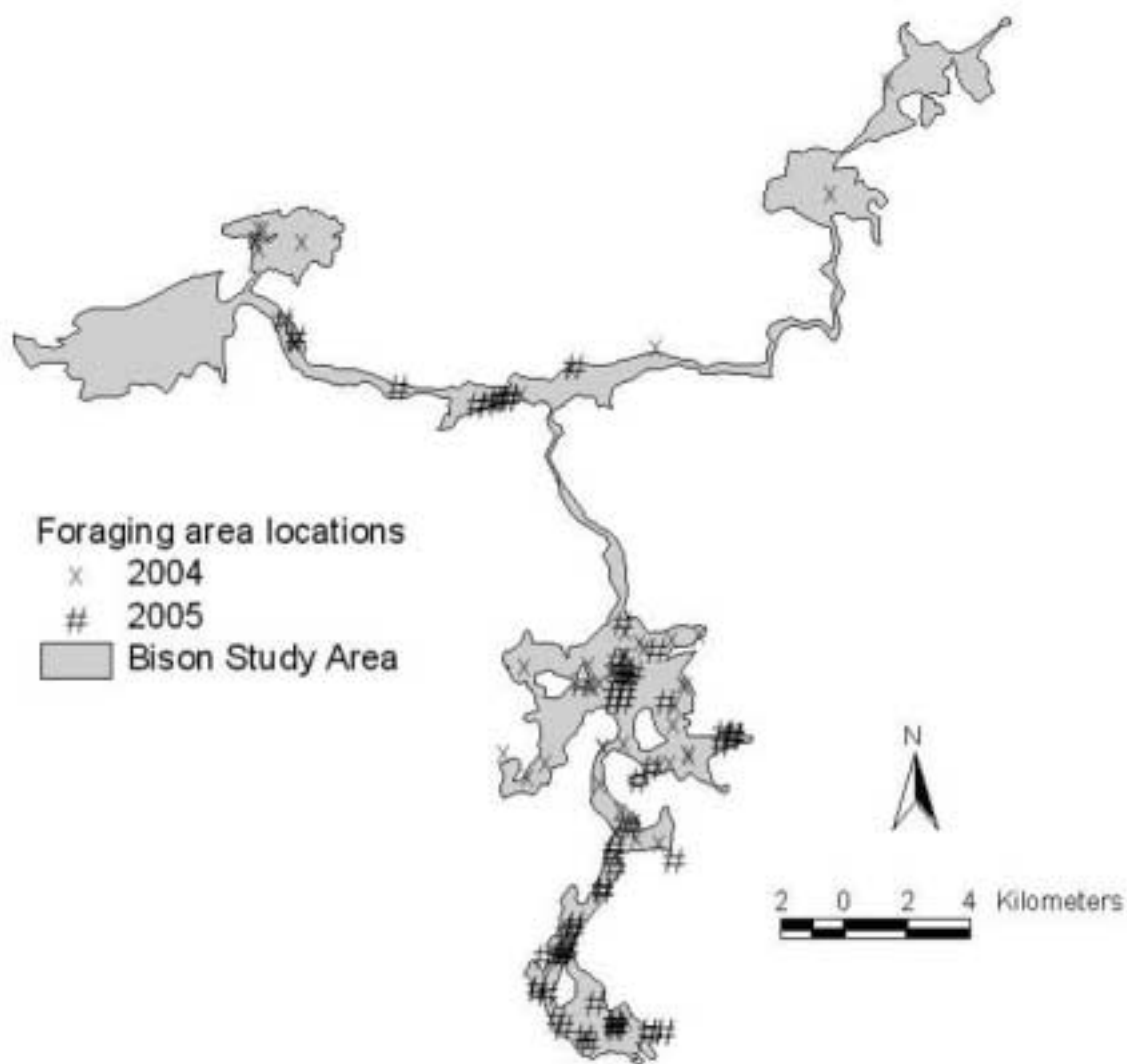
Figure 4.2. The distribution of the 130 foraging areas throughout the Madison-Gibbon-Firehole study area in Yellowstone National Park obtained from January-March during 2004 and 2005.
