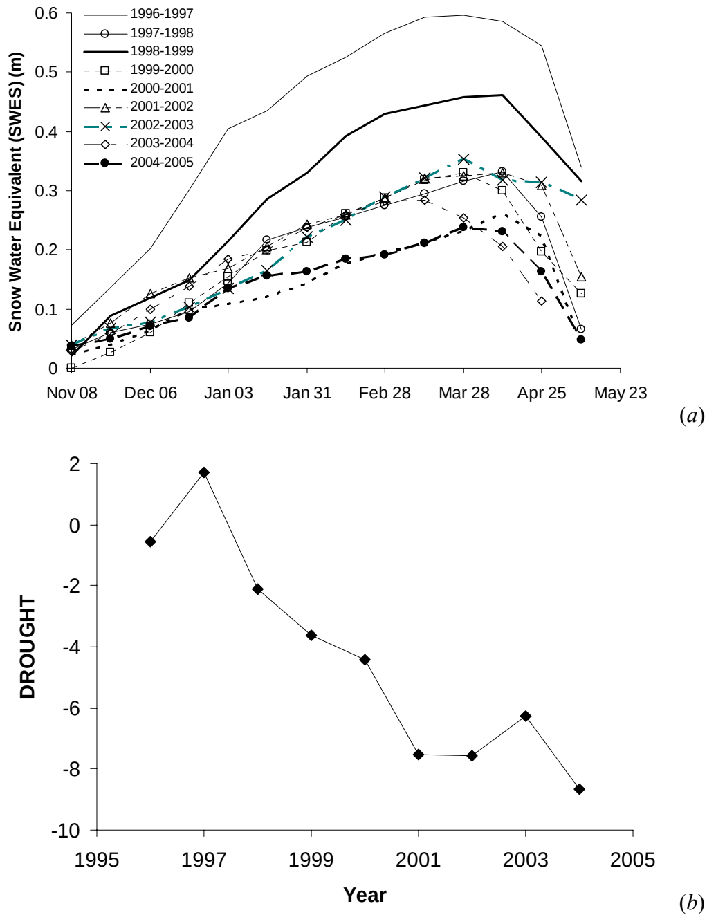
Figure 1.3. Temporal patterns in (a) the summer range snow water equivalent covariate (SWES) during winter, 1996-97 to 2004-05, and (b) the annual drought covariate (DROUGHT), 1996-2004, for Yellowstone National Park. Snow water equivalent values were measured at a SNOTEL site at Canyon, Wyoming, and averaged over two-week intervals. Values for DROUGHT were obtained from monthly averages of the Palmer Drought Severity Index during the growing season. Note that drought severity increases as values of DROUGHT become more negative.
