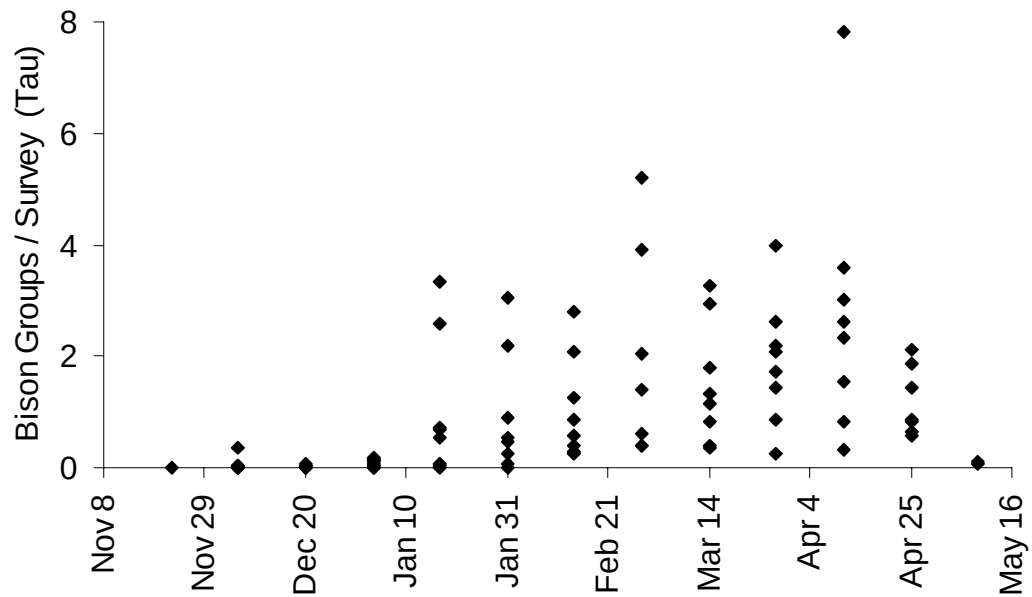
Figure 3C.11. The bison off-road travel response variable ( \tau_{ij} ) for each period and year as calculated using data from bison ground distribution surveys from 1997-98 through 2004-05.
