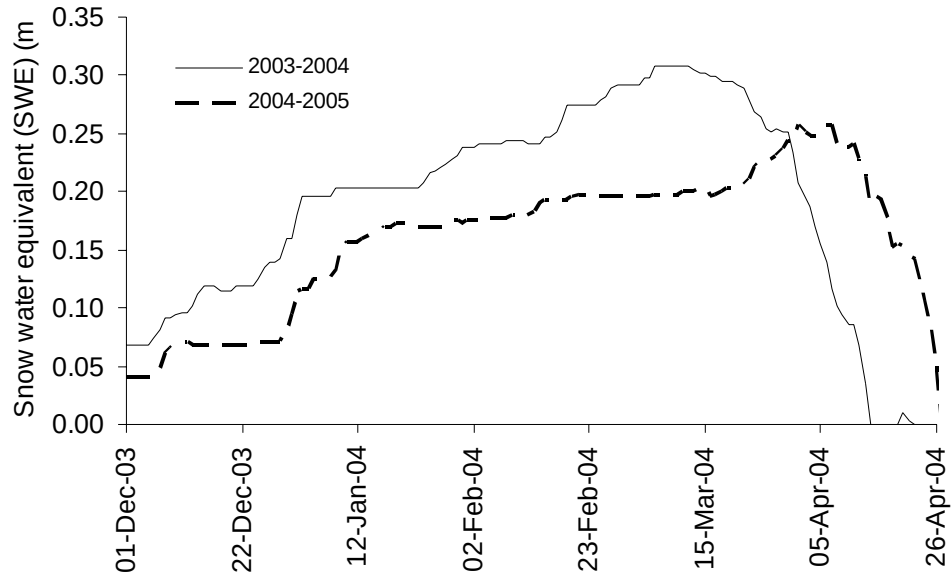
Figure 4.3. Temporal trends in snowpack snow water equivalent (SWE) as determined from daily measurements at the West Yellowstone SNOTEL site from December-April for 2003-04 and 2004-05.
