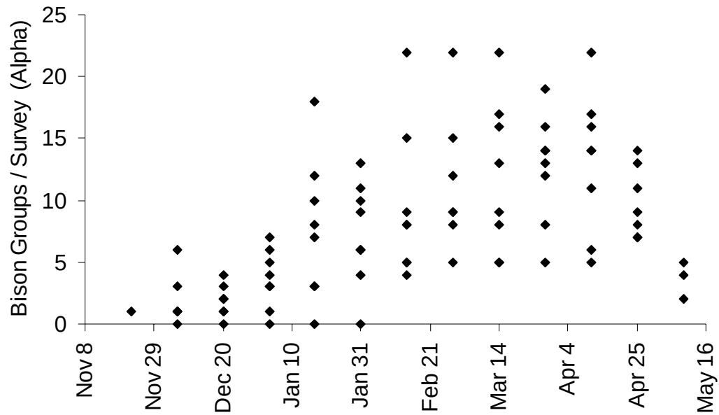
Figure 3C.8. The number of bison groups observed traveling off-roads per survey effort ( \alpha_{ij} ) for each period and year during bison ground distribution surveys from 1997-98 through 2004-05.
