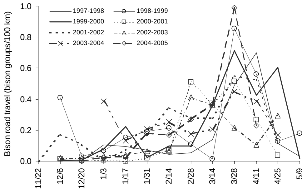
Figure 3.4. Temporal variability in bison road travel in the Madison-Gibbon-Firehole area of Yellowstone National Park during winter, 1997-98 to 2004-05. Bison groups per 100 km of road surveyed ( \rho_{ij} ), calculated from my road use surveys, are presented for each time interval ( i ) and year ( j ).
