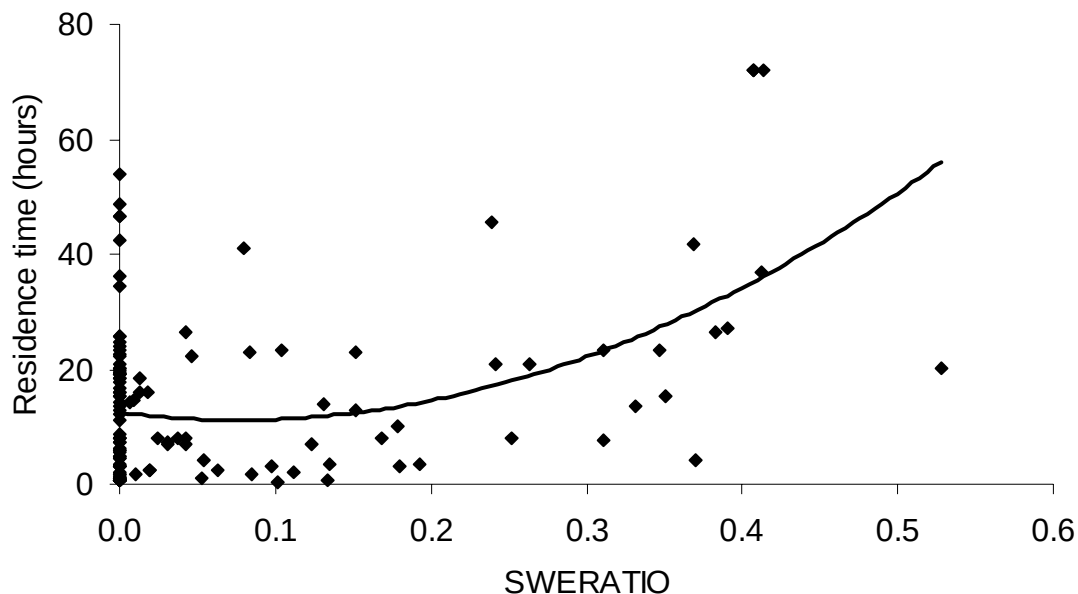
Figure 4.5. Plots of data points for foraging area residence time ( \tau ) versus the SWERATIO covariate. Data are from bison foraging area locations in the Madison-Gibbon-Firehole area of Yellowstone National Park obtained from January-March during 2004 and 2005.
