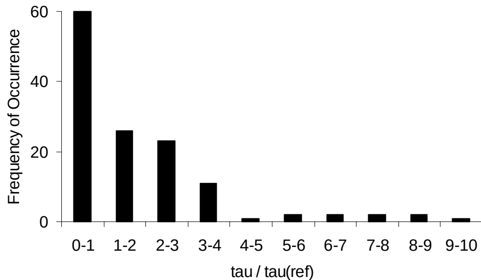
Figure 4.7. Histogram showing distribution of \tau/\tau_{ref} for 130 bison foraging areas in the Madison-Gibbon-Firehole area of Yellowstone National Park during January-March 2004 and 2005.
