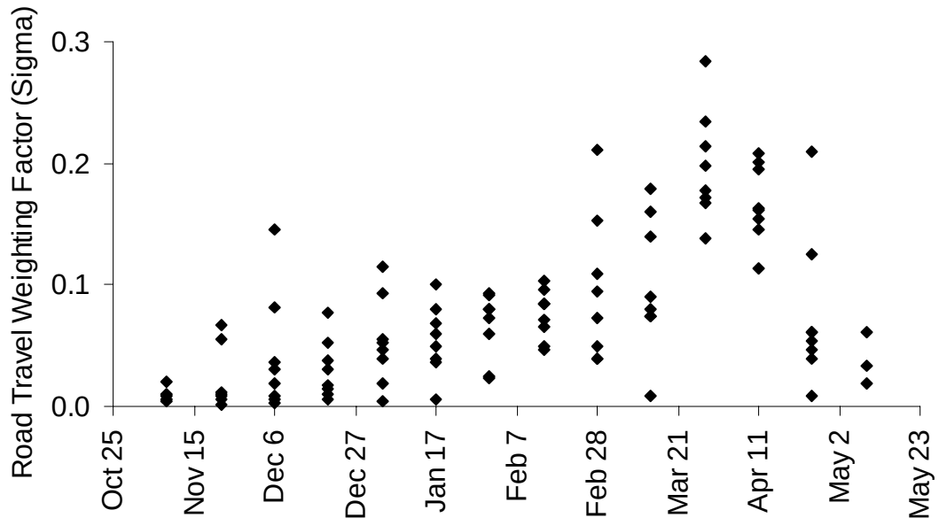
Figure 3C.4. The road travel weighting factor ( \sigma_{ij} ) for each period and year as calculated using data from bison road use surveys from 1997-98 through 2004-05.
