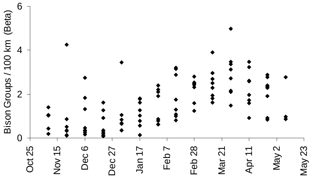
Figure 3C.2. The number of bison groups observed traveling on roads per 100 km of road survey effort ( \beta_{ij} ) for each period and year during bison road use surveys from 1997-98 through 2004-05.
