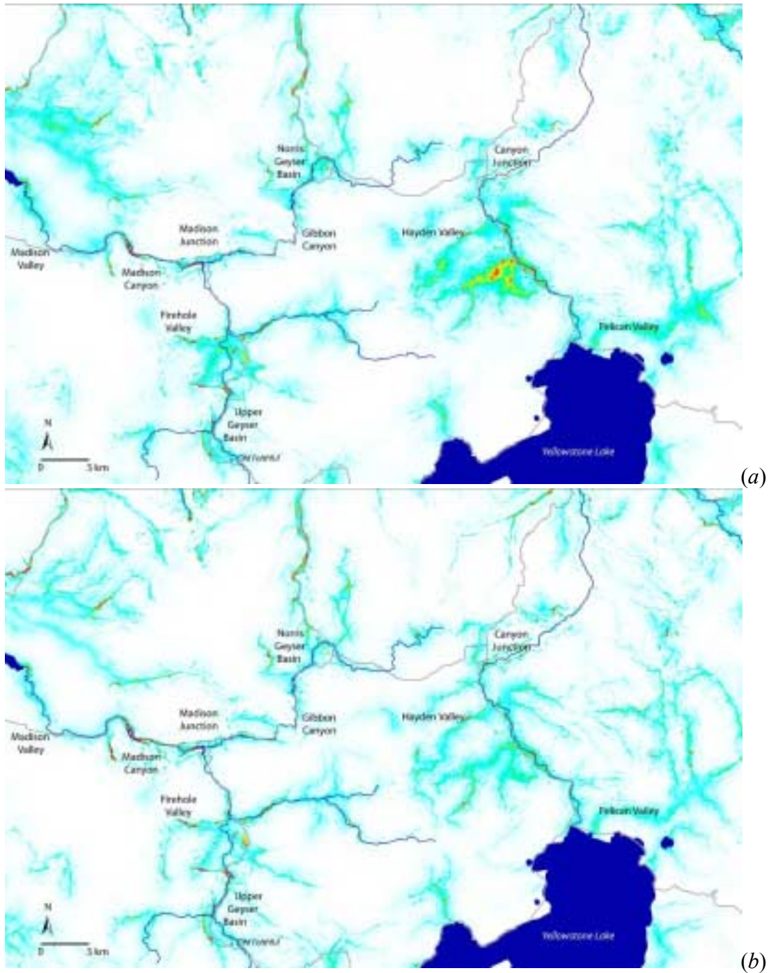
Figure 2.3. Probability maps developed from the best approximating a priori models examining the effects of topography and habitat type attributes on (a) general bison travel, and (b) bison long distance travel throughout central Yellowstone National Park. White areas represent a travel probability of zero and travel probability increases as colors darken from green to red to dark blue, with dark blue corresponding to a probability of one. Roads are depicted in grayish shading and streams in blue.
