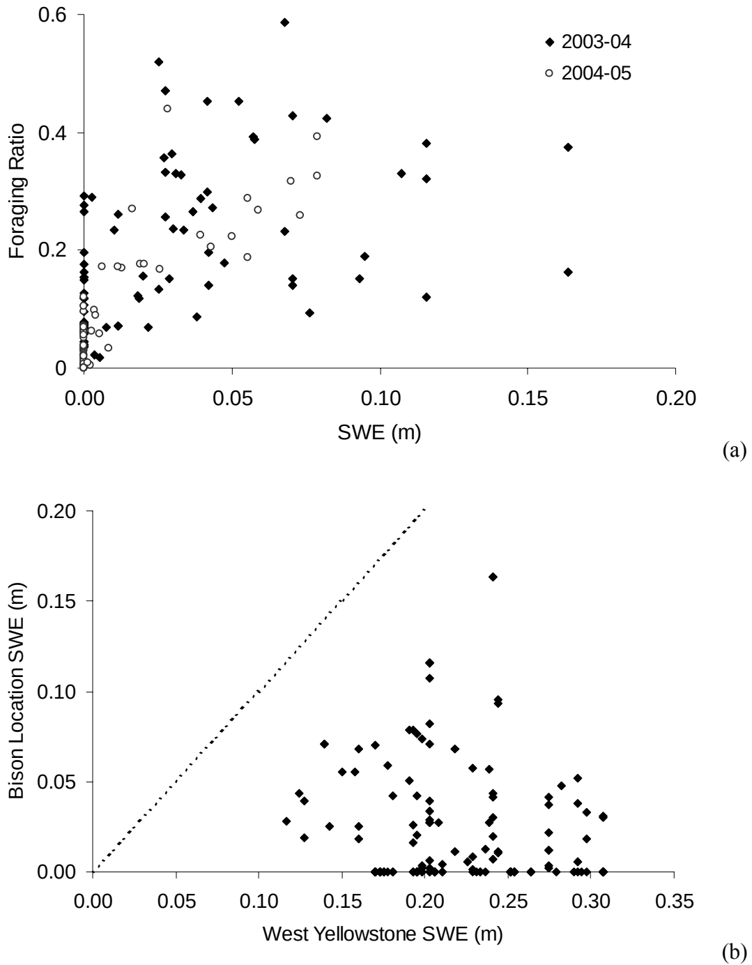
Figure 5.4. The relationship between (a) the foraging ratio and snow water equivalent (SWE) for bison locations obtained throughout the Madison-Gibbon-Firehole study area in Yellowstone National Park from December-March during 2003-04 and 2004-05, and (b) SWE for bison locations and landscape SWE as indexed by the West Yellowstone SNOTEL site. The line y=x is denoted.
