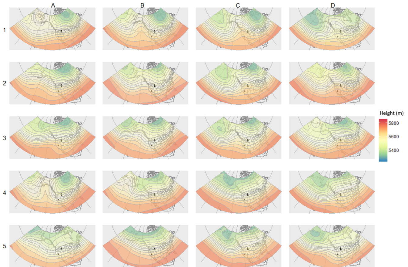
Figure 2. Array of 500 mbar geopotential height map patterns generated using self-organizing maps. Each map pattern, or synoptic type, is a generalization of a group of days exhibiting a similar circulation pattern.
