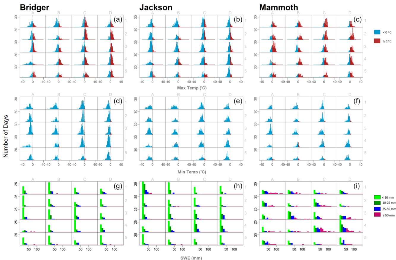
Figure 3. Histograms of daily maximum temperature (a–c), minimum temperature (d–f), and snow water equivalence totals (g–i) for Bridger Bowl (a, d, g), Jackson (b, e, h), and Mammoth Mountain (c, f, i). For each of the nine arrays, the position of the plot corresponds with the map pattern shown in Figs. 2 and 3. For example, the histograms located in the upper left corner of each array correspond with synoptic type A1.
