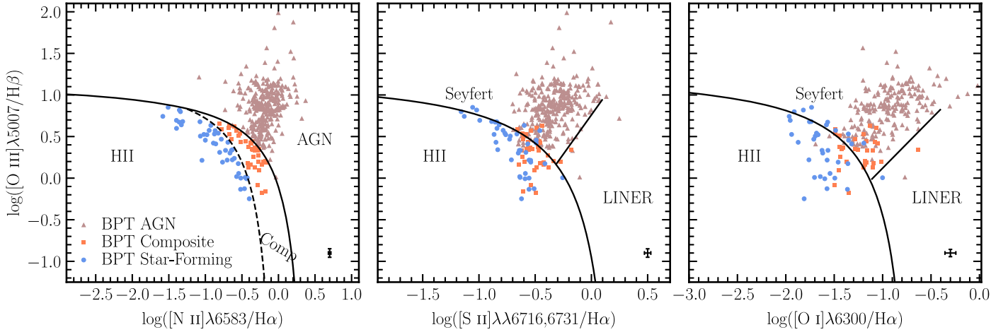
Figure 6. The left panel shows the [O III]/H \beta vs. [N II]/H \alpha narrow-line diagnostic diagram for our outflow candidates in the GAMA survey using the classification scheme summarized in L. J. Kewley et al. (2006). Here, 394/398 of the outflow galaxies with reliable emission lines relevant to this diagram are plotted, of which 312 are AGNs (rosy brown triangles), 39 are composites (coral squares), and 43 are SF galaxies (cornflower blue circles). The middle and right panels show these objects in the [O III]/H \beta vs. [S II]/H \alpha and [O I]/H \alpha diagrams. Only galaxies with reliable emission lines are plotted in these panels. Characteristic error bars are located in the lower-right region of each panel. See Section 4.1 for details.
