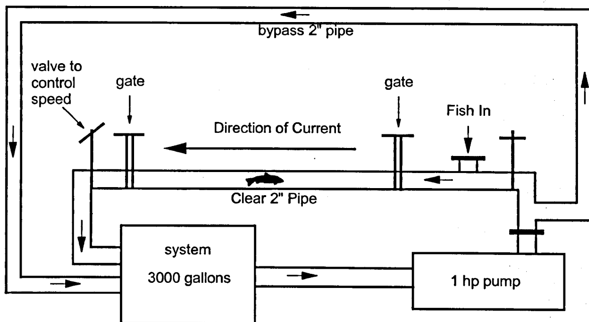
Figure 2.1—Stamina Tunnel. Arrows indicate direction of flow.
