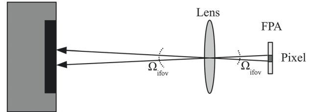
Fig. 1 Geometric optical layout of the camera focal plane array (FPA) viewing an external blackbody with instantaneous field-of-view (ifov) solid angle \Omega_{ifov} determined by the pixel area and the lens focal length.
