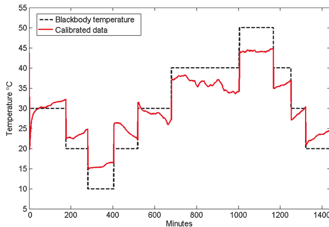
Fig. 4 Time series plot of the blackbody set-point temperature (black dashed line) and the camera output calibrated in a conventional manner without a correction for FPA temperature changes (red solid line). The spatial standard deviation is comparable to the thickness of the solid line.
