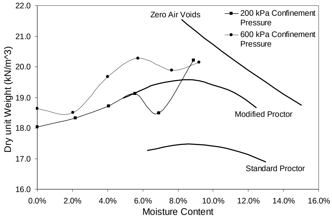
Figure 17: A-1-a Compaction Curve for 500 Gyrations at 200 & 600 kPa Confinement Pressures
