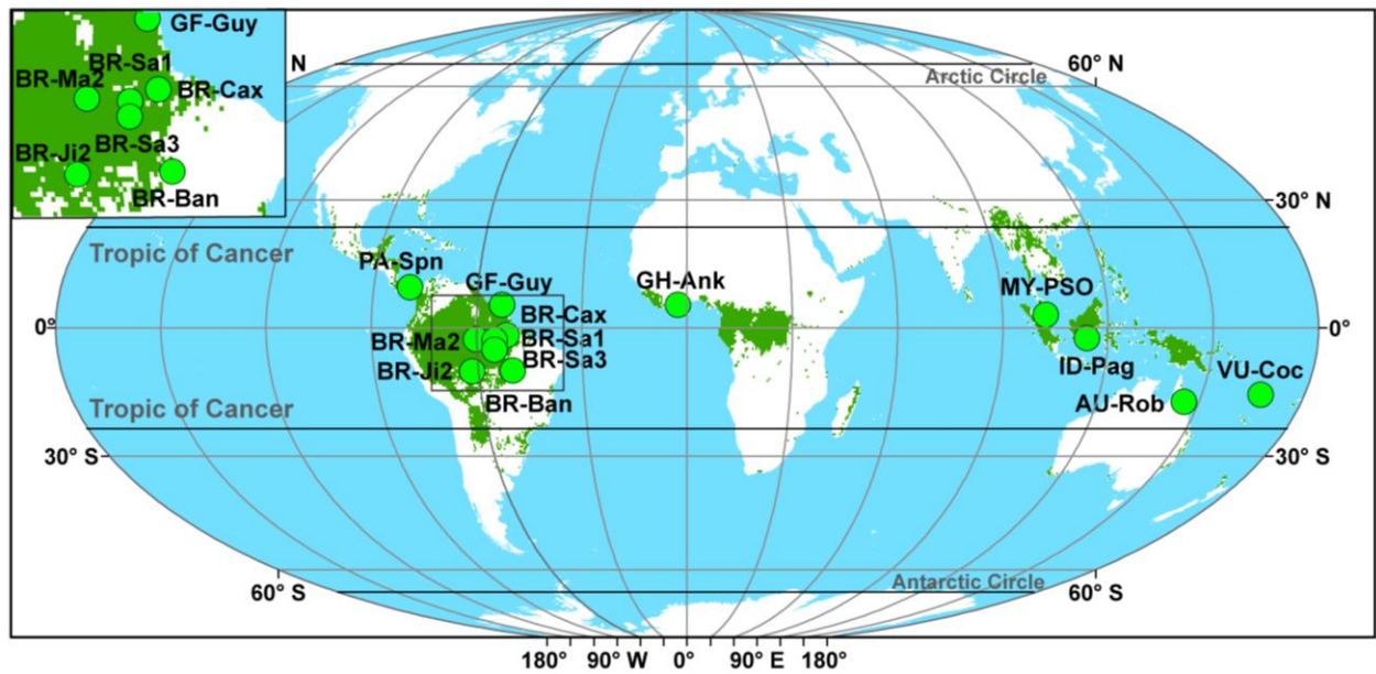
Fig 2. A map of global tropical rainforest area (in green) based on the MODI MCD12C1 land cover classification with the location and distribution of the 13 tropical rainforest eddy covariance sites used in this study (see Table 1).
