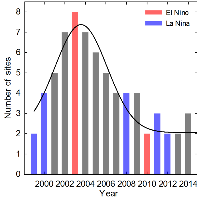
Fig. 3. The number of tropical rainforest eddy covariance research sites per year with data archived in the LaThuile and/or FLUXNET2015 databases per year as of March 2017.
