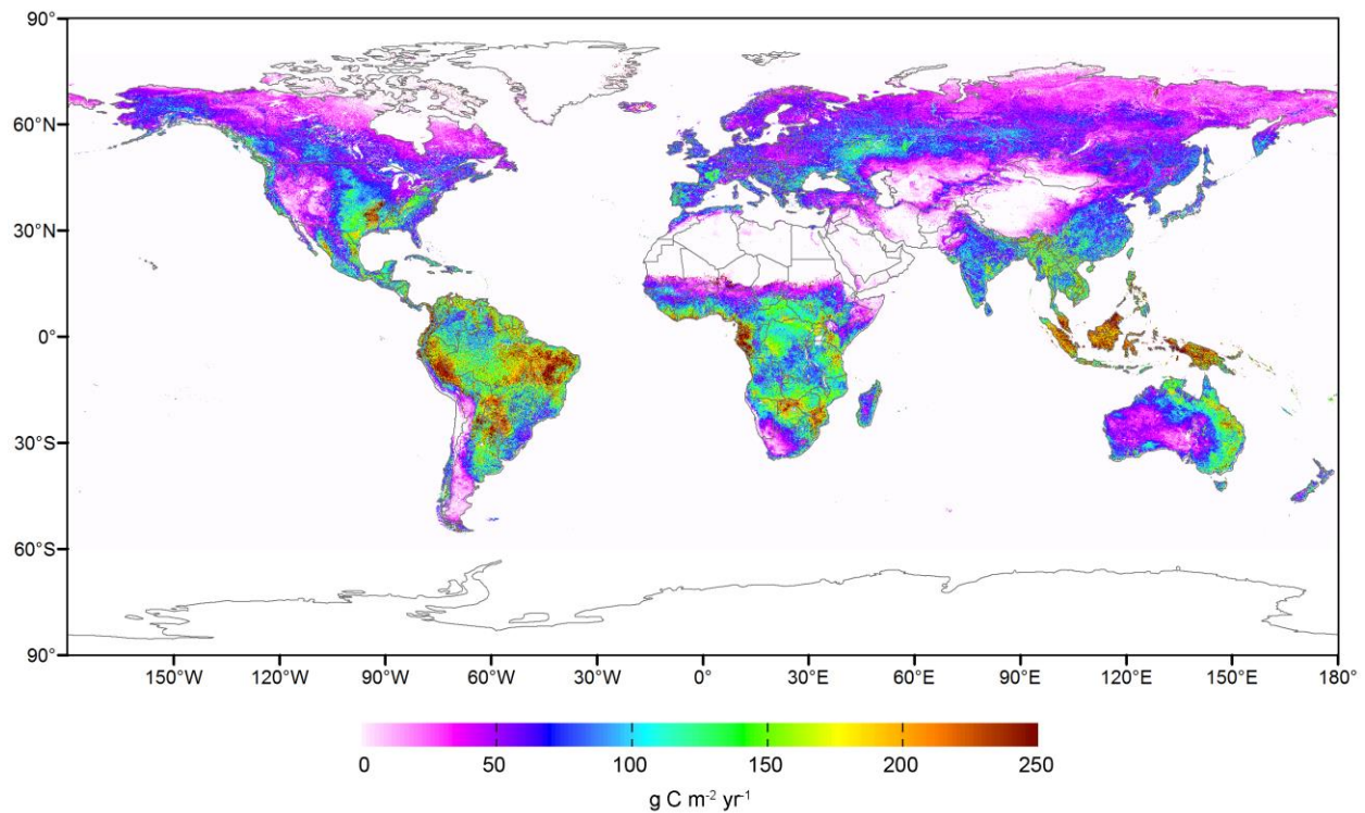
Fig. 1. The standard deviation of annual gross ecosystem productivity (GEP) in the annual totals from MODIS (MOD17A3) for the period 2000-2015.
