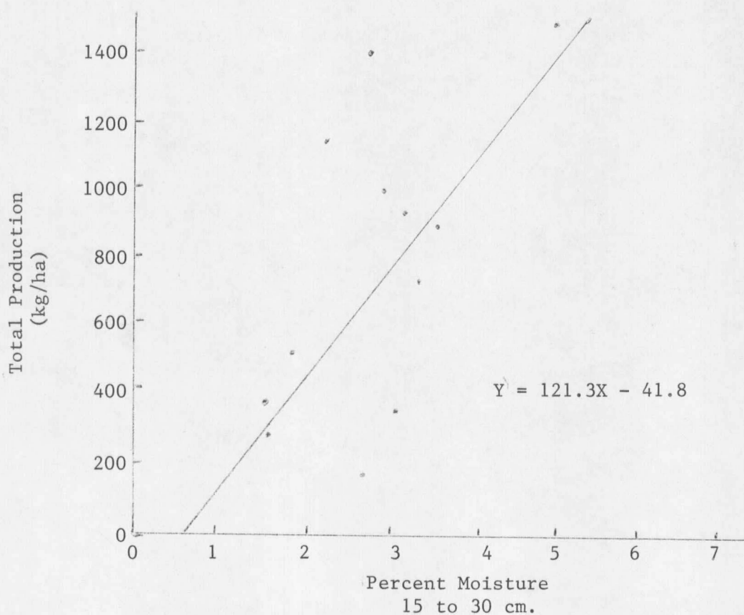
Figure 5. Regression of total production on percent moisture for the sampling depth of 15 to 30 centimeters.
