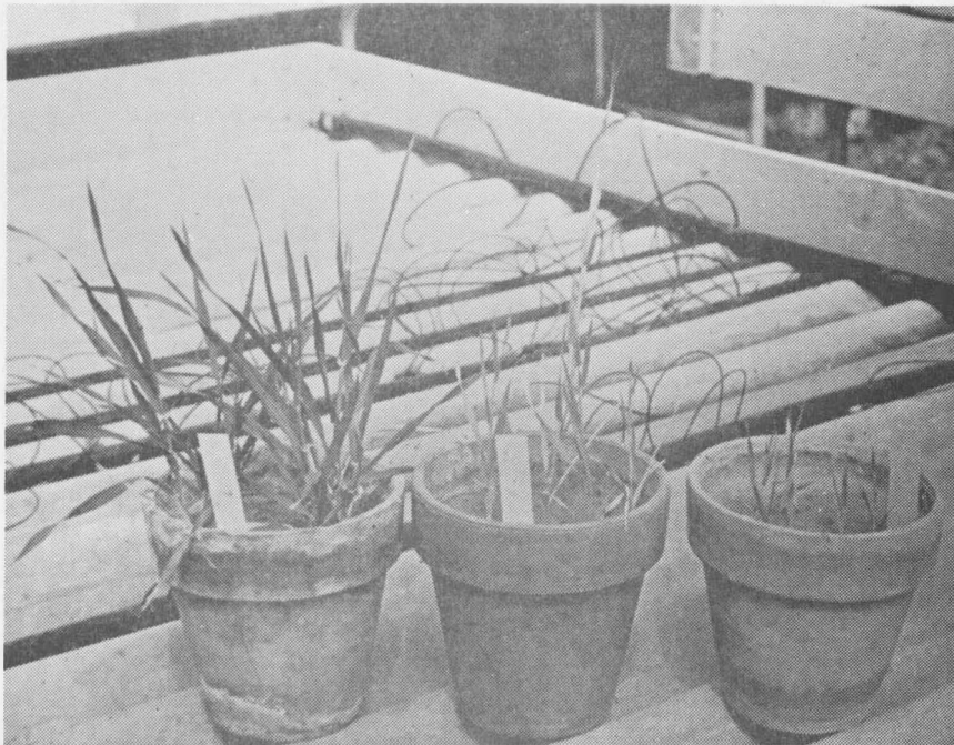
Figure 2. Results of N = 112, P = 112, K = 0 kg/ha in pot one; N = 56, P = 56, K = 56 kg/ha in pot two; and N = 0, P = 56, K = 112 kg/ha in pot three.
