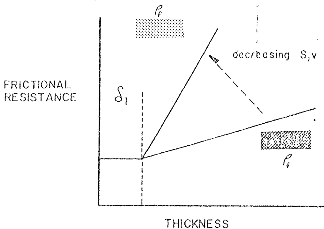
Figure 8b. Change in frictional resistance related to change in biofilm thickness.
