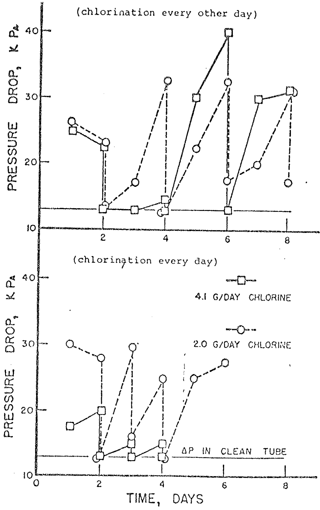
Figure 13. Shock Chlorination Effect on Frictional Resistance.
