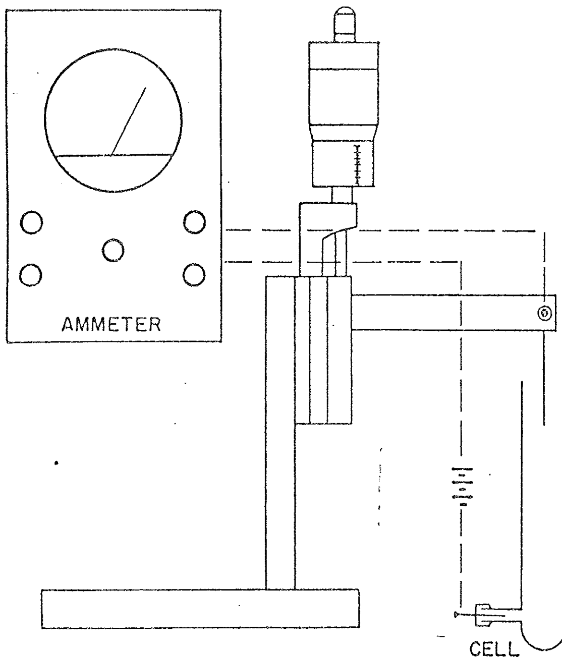
Figure 5. Volumetric Displacement Method for Biofilm Thickness Measurement.
