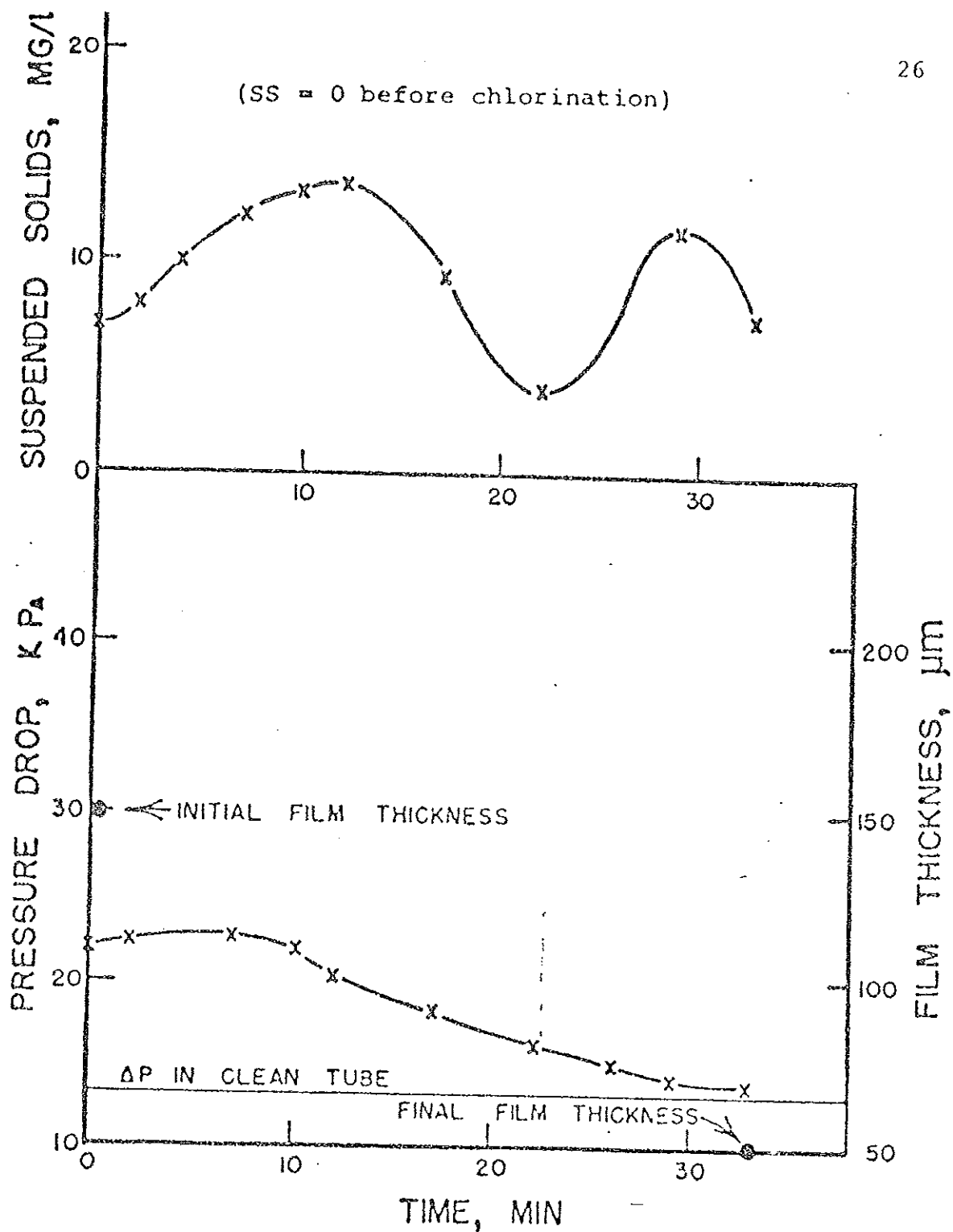
Figure 12. Pressure Drop, Thickness, and Suspended Solids Concentration During Shock Chlorination at 4.1 mg/l, Flow Rate = 11.4 l/min.
