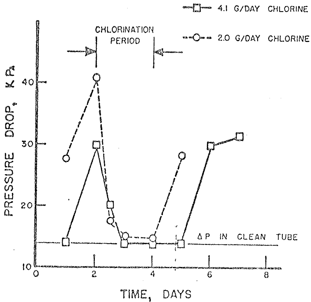
Figure 14. Effect of Continuous Chlorination on Frictional Resistance at Flow Rate = 11.4 l/min.
