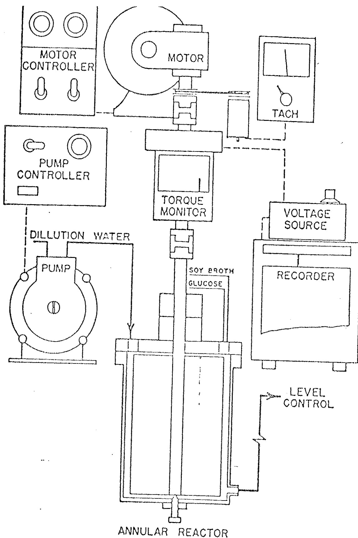
Figure 2. Experimental System for Evaluating Effect of Velocity, Water Quality and Bulk Temperature on Biofouling Rate (AFR). Also Used for Determining Kinetics of Fouling Control via Chemical Treatment (e.g., chlorine, ozone, etc.).
