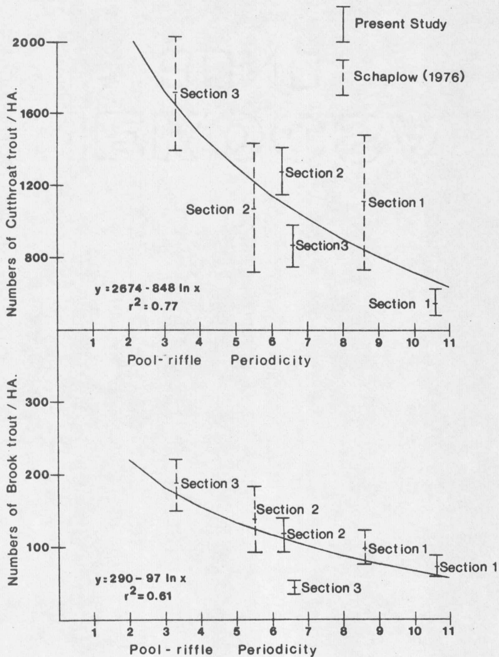
Figure 8. The curvilinear relationships of the total numbers of (A) cutthroat trout and (B) brook trout to pool-riffle periodicity. Bars represent 80% confidence intervals.
