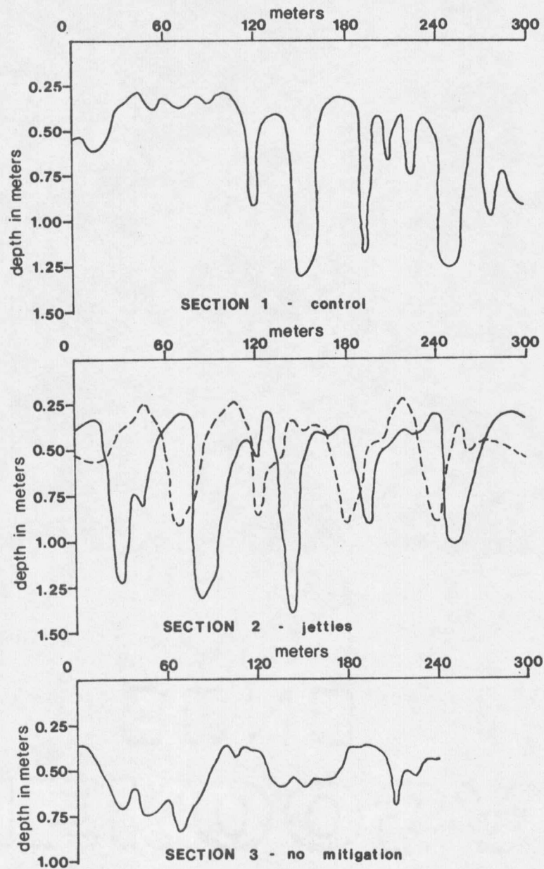
Figure 9. Profiles of the stream bed along the thalweg in the sections of Little Prickley Pear Creek from the present study (solid line) with comparable measurements from Elser (1968) (dotted line).
