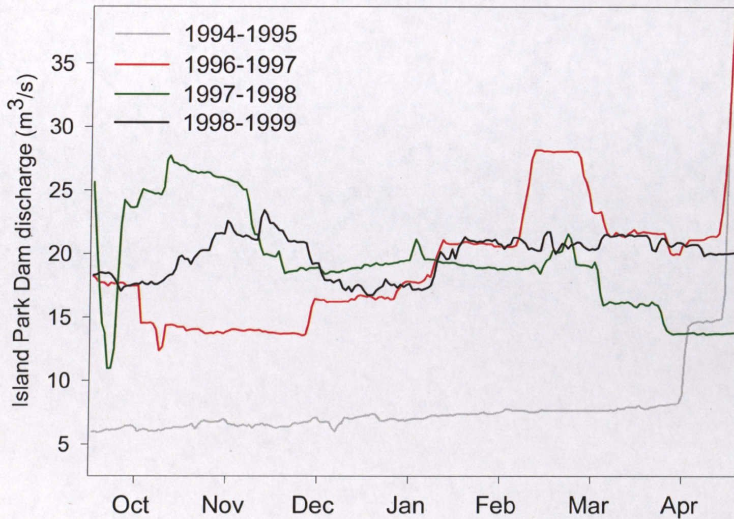
Figure 6.5.—Discharge ( \text{m}^3/\text{s} ) from Island Park Dam from October through April in four winters. Tick marks indicate the 15 th day of each month.
