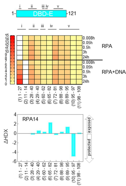
Figure 2. Global deuterium uptake profiles and DNA induced changes in RPA. Heat map representing the deuterium content of (A), RPA70, (B) RPA32 and (C) RPA14 peptides in unbound and DNA bound states as a function of time. Each row represents a timepoint and each column represents a peptide. The heat map gradients are color coded yellow (low deuterium uptake) to red (high deuterium uptake). The white boxes depict absence of a corresponding dataset for specific peptides under one condition (presence or absence of DNA). • denotes peptides in DNA-binding sites, and + marks peptides from the linker regions. To map the peptide location in RPA70, RPA32 and RPA14, peptides in same region were grouped and assigned roman numerals. Binding to ssDNA leads to varying patterns of protection by HDX-MS and the differences are denoted as bar graphs below the respective heat maps. The arrows denote whether the peptides were protected or exposed to solvent upon DNA binding. The data show the cumulative difference in deuterium uptake ( \Delta HDX) in RPA over all five HDX timepoints.
