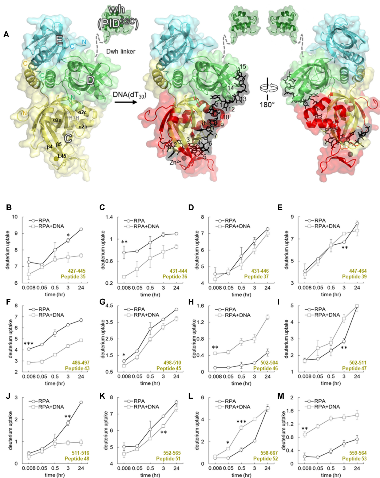
Figure 4. Time-resolved HDX-MS analysis of DNA-induced conformational changes in DBD-C. (A) Crystal structure of the Tri-C core of human RPA composed of DBD-C, RPA32 and RPA14. The peptides identified in the MS analysis corresponding to DBD-C are denoted in red. DNA is denoted as black sticks. (B–M) Deuterium exchange profiles of individual peptides from DBD-C are shown. Error bars reflect standard deviations, calculated as described in ‘Material and Methods’. */**/** are P -values calculated using a two-tailed unpaired t -test between the respective time points for the RPA and RPA+DNA samples. Each star denotes t -test values that differ by an order of magnitude. P -values are denoted in Supplementary Table S2. No significance indicated as ‘ns’.
