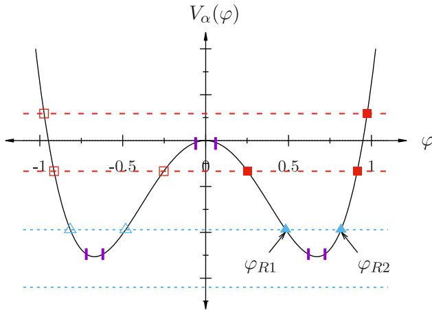
FIG. 2. Schematic diagram of the conformal coupling potential, where we used \beta = -4.5 and \delta = 10 . Purple dashes represent boundaries of the regions consistent with pPN constraints [determined by Eq. (13)]. Horizontal dashed lines (as well as the squares and triangles marking their intersections with the potential) are a representation of BBN constraints on the speedup factor and determine the regions in the potential consistent with nucleosynthesis at the end of the radiation era. Because of the symmetry of the potential, we shade in the squares/triangles on the right to indicate that one only needs to consider these initial conditions without loss of generality. \varphi_{R1} and \varphi_{R2} indicate the points we investigate in this paper.
