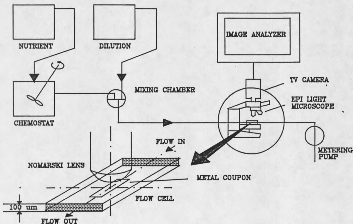
Figure 2. Experimental system
