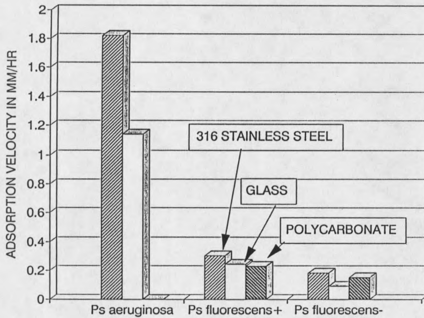
Figure 26. Comparison of reversible and irreversible adsorption velocities to 316 stainless steel, glass and polycarbonate of Pseudomonas aeruginosa , Pseudomonas fluorescens (mot+), and Pseudomonas fluorescens (mot-). Shear stress 0.75 \text{ N m}^{-2} .
