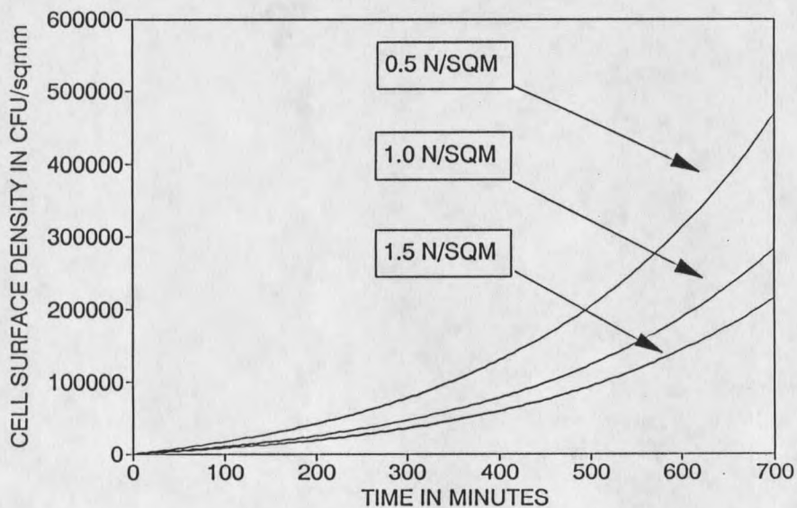
Figure 21. Simulation of cell accumulation of Pseudomonas aeruginosa on 316 stainless steel at various shear stress. Bulk water cell concentration 6 \times 10^6 \text{ cells ml}^{-1} .
