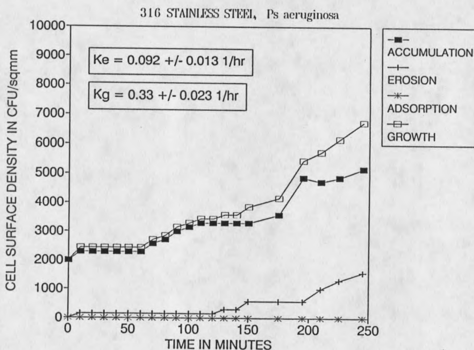
Figure 7. Cell accumulation of Pseudomonas aeruginosa on 316 stainless steel using a bulk water concentration of 1.1 \times 10^6 \text{ cells ml}^{-1} (Figure 7 a) and a sterile nutrient (40 ppm C) after initial cell colonization of 2000 \text{ CFU mm}^{-2} (Figure 7 b). Shear stress 0.75 \text{ N m}^{-2} .
