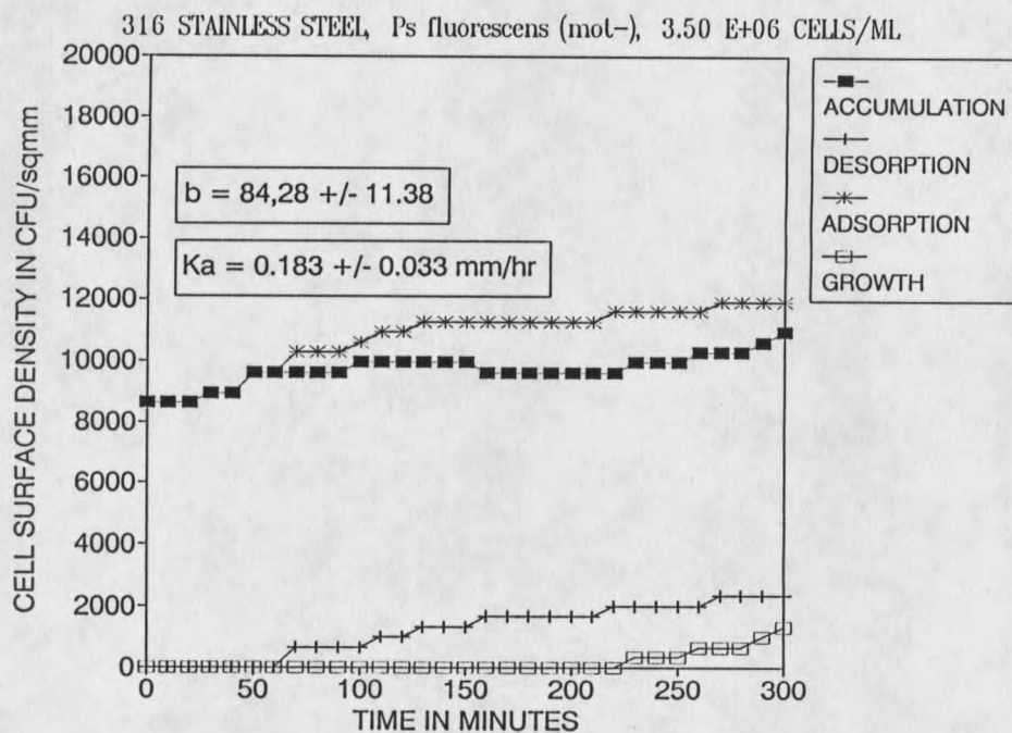
Figure 12. Cell accumulation of Pseudomonas fluorescens (mot-) on 316 stainless steel using a bulk water concentration of 3.5 \times 10^6 \text{ cells ml}^{-1} . Shear stress 0.75 \text{ N m}^{-2} .
