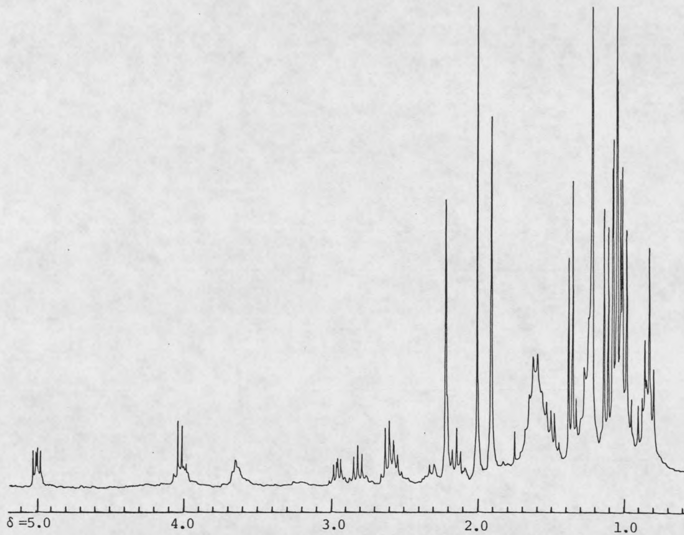
Figure 10. ^1\text{H} NMR spectrum of siphonarin I.
