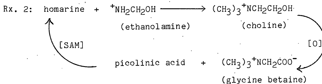
Figure 3. Homarine as a methylating agent.
