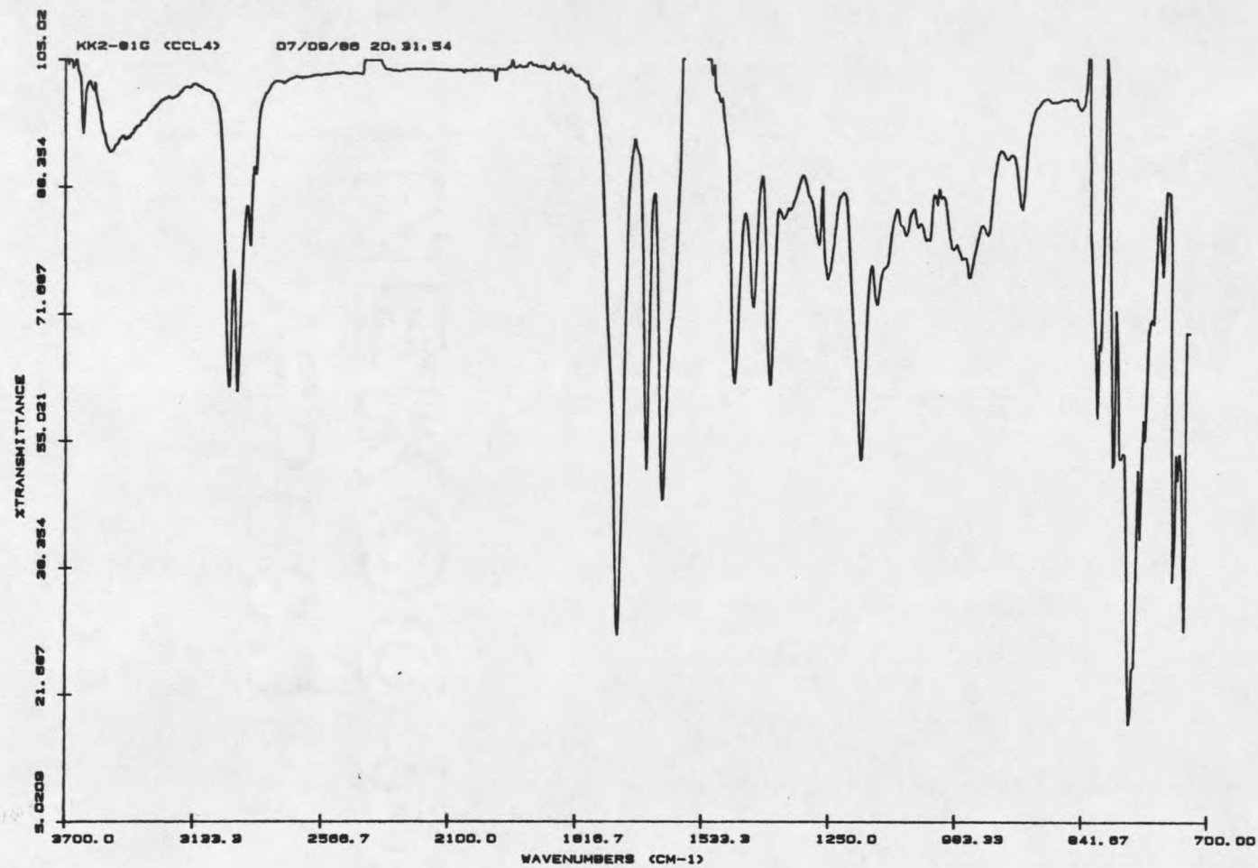
Figure 8. IR spectrum of siphonarin J.
