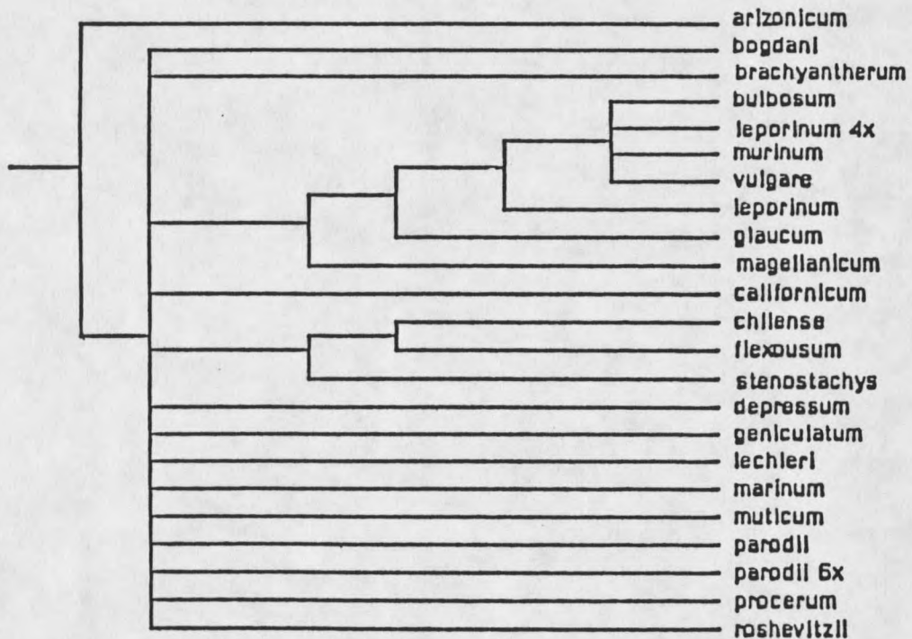
Figure 25. Strict consensus tree for 23 Hordeum species when only intraspecific monomorphic PCR fragments were included in the data matrix.
