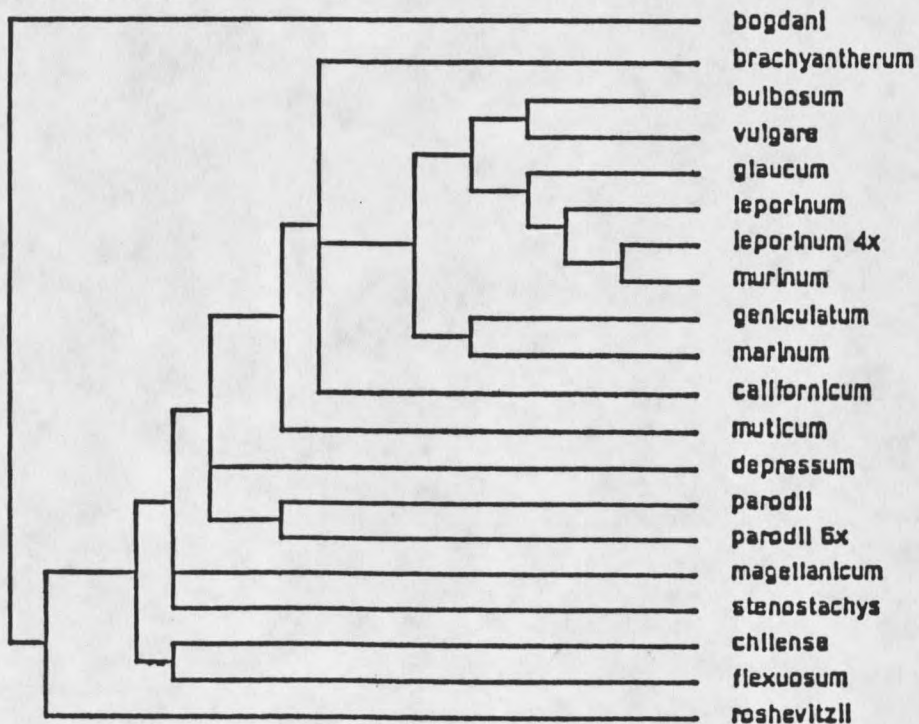
Figure 26. Strict consensus tree for 20 Hordeum species after PCR data for allopolyploid species were excluded from the analyses.
