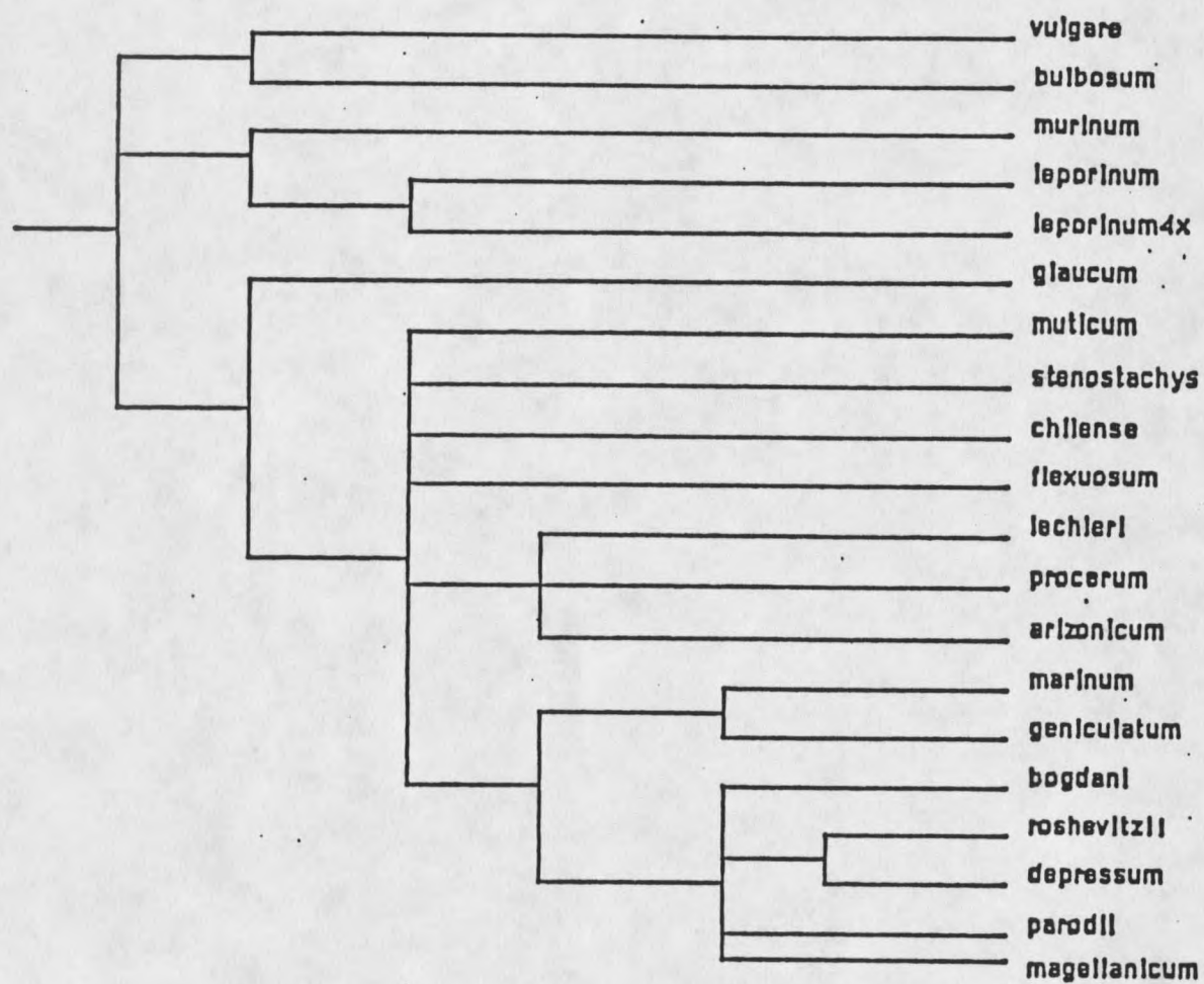
Figure 18. Strict consensus tree for Southern data of 20 Hordeum species.
