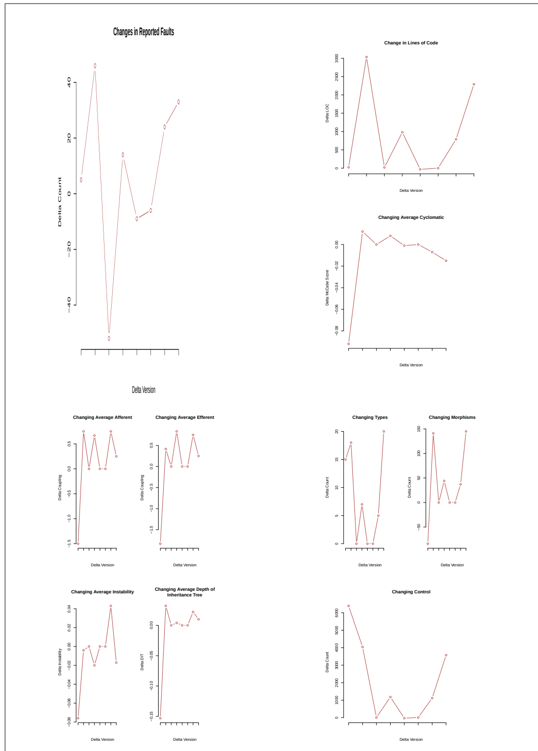
Figure A.4: Commons-Lang Delta Profile
