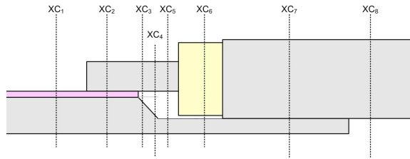
Figure 5.7: Side view of the coaxial cable segments used within the FEA tool. These are defined in table 5.1.
