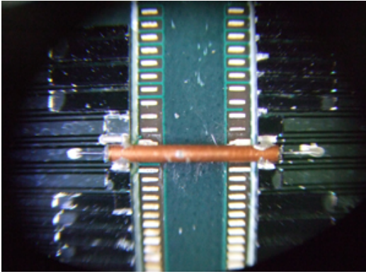
(a) Image shows the coaxial cable connecting the two dies together. The cable replaced the original wire bonds.
