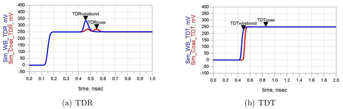
Figure 5.9: The TDR and TDT results based on the models from the FEA, comparing both the wire bond system to the coax cable system.
