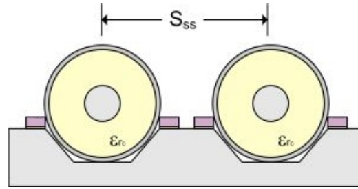
Figure 3.5: Dimension of two side by side coaxial cables mounted within separate trenches.
