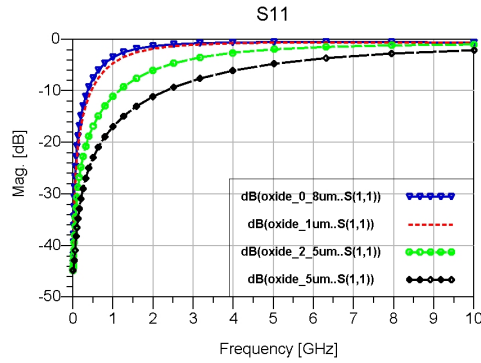
(a) The S_{11} S-parameter Substrate losses
