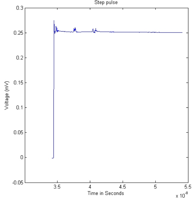
Figure 5.2: The TDR/TDT Gaussian Step.
