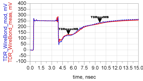
(a) Wire bond TDR
