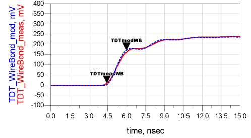
(b) Wire bond TDT
