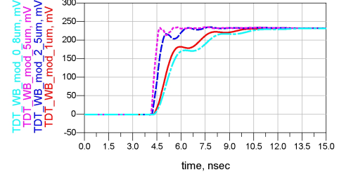
(b) The TDT plot.
