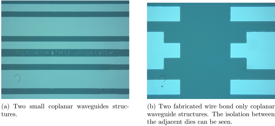
Figure 4.5: Shows the details of the coplanar waveguide structures fabricated with aluminium.
