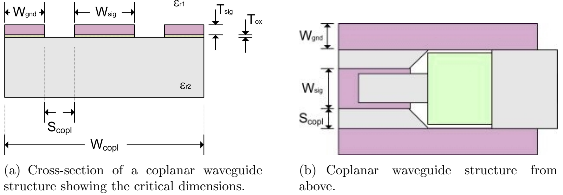
Figure 3.3: The Coplanar transmission line dimensions
