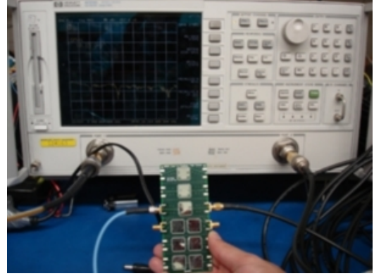
(b) The setup for VNA Test.
