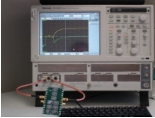
(a) The setup for TDR/TDT Test.
