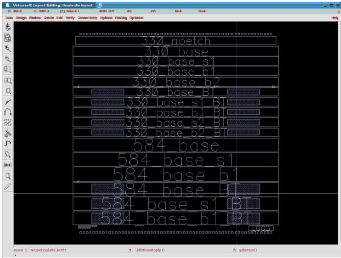
Figure A.3: Shows the different coplanar waveguide structures. The different sizes can be seen by the text describing in terms of small/large and if the signal trace has been increased or decreased.
