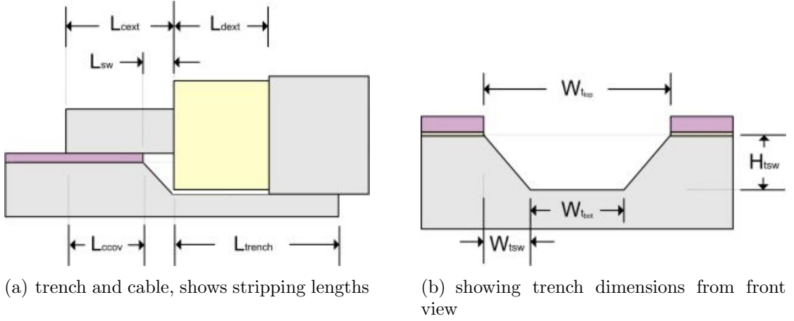
Figure 3.4: Trench and transition dimensions
