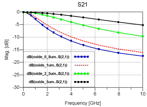
(b) The S_{21} S-parameter Substrate losses
