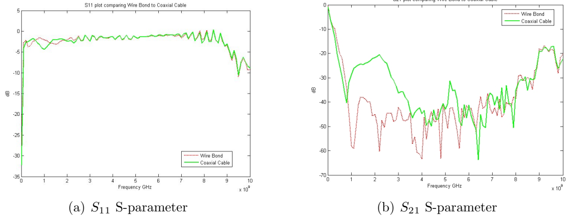
Figure 5.4: The S-parameters of Wire Bond compared to Coaxial Cable.
