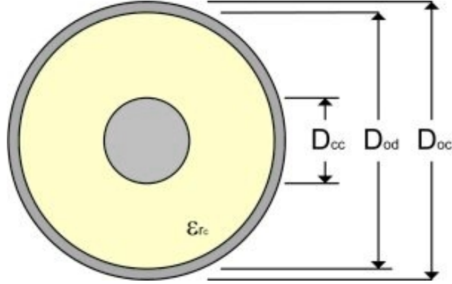
Figure 3.2: Coaxial Cable Dimensions
