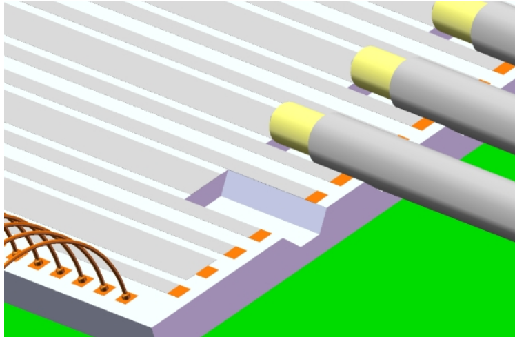
Figure 3.1: Magnified view of the etched transition trenches and coplanar waveguide structures. This figure shows trenches with and without cables.
