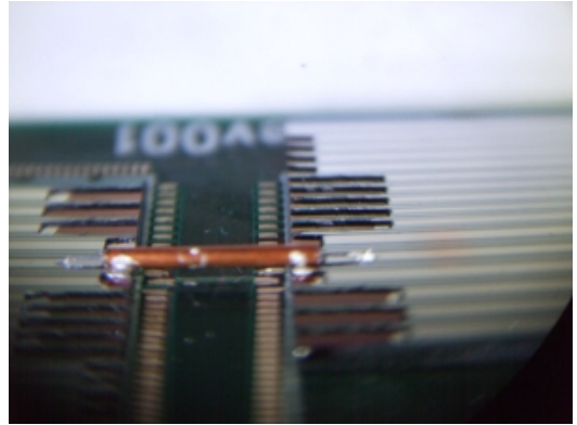
(d) Coax Cable connecting adjacent dies together.
