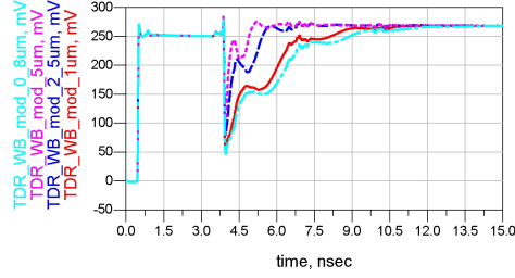
(a) The TDR plot.
