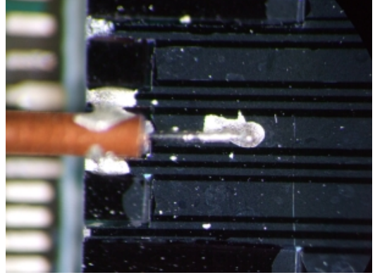
(b) Image shows the coaxial cable connections to the CPW for the signal path and return paths
