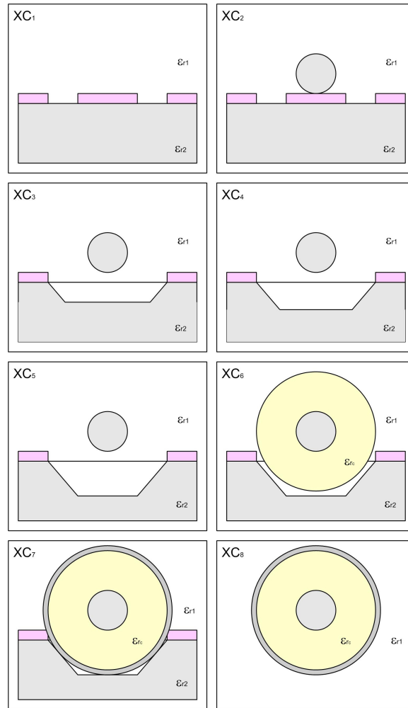
Figure 5.8: Shows the cross sections of the coaxial cable. These sections match up the segments in figure 5.7.
