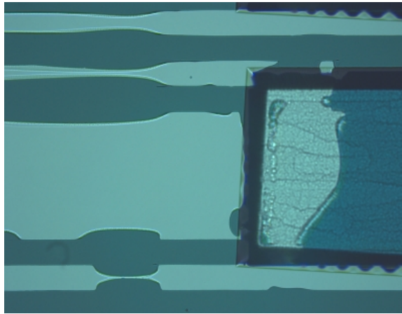
Figure 6.3: Aluminium traces of the coplanar waveguide structure etched incorrectly due to Photoresist streaking.
