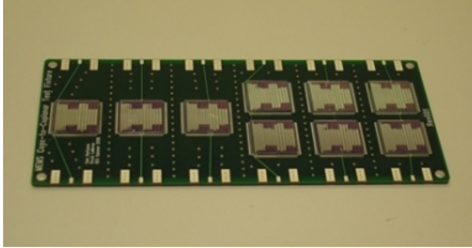
Figure 4.6: Test Fixure for test comparision between wire bond to coax cable launch.
