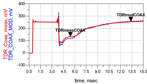
(c) Coax Cable TDR
