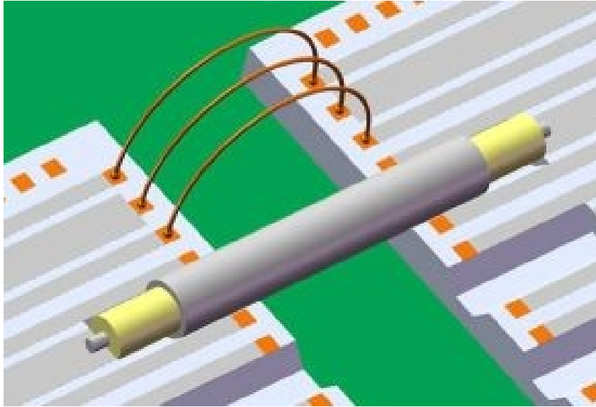
Figure 1.1: Shows 3 dimensional of how two dies could be connected by both wire bonds and coaxial cable.
