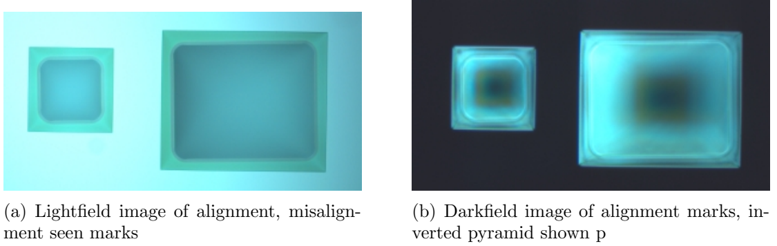
Figure 4.4: Alignment marks showing the silicon crystal plane.
